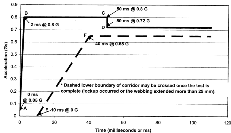
Figure 8: Acceleration Corridors
