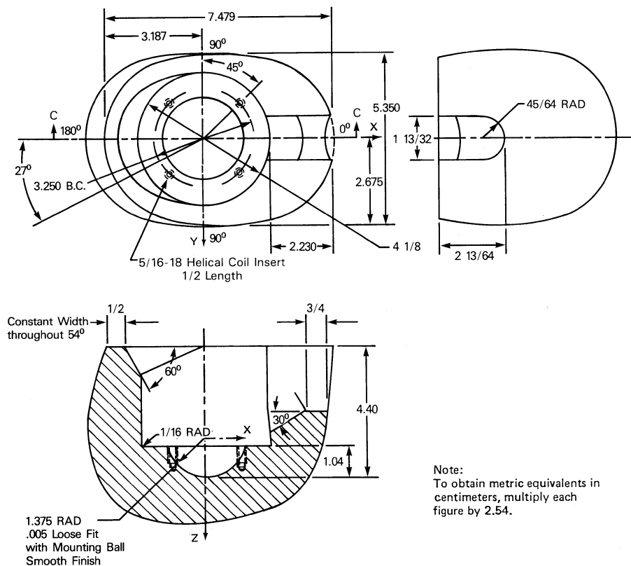
Section C-C
