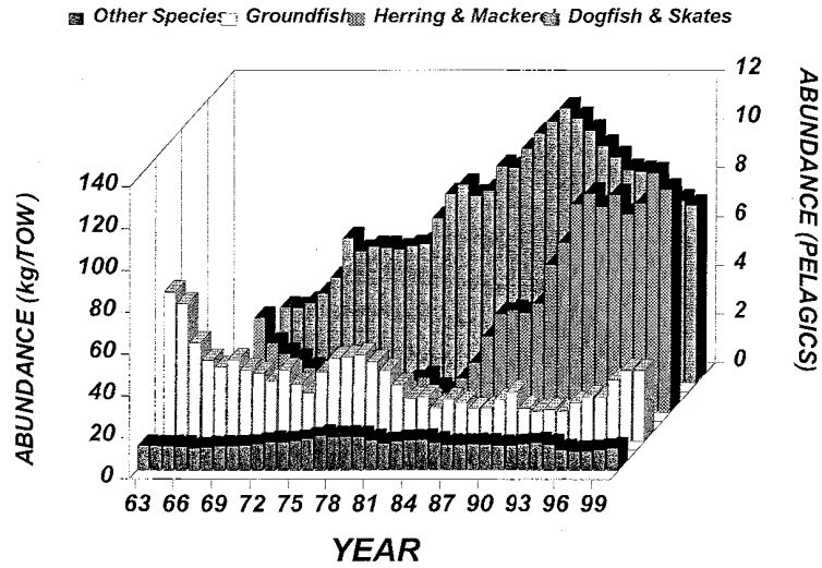
Exhibit 1. Trends in the relative abundance (expressed as kilograms per half-hour trawl tow) for four major species groups off the Northeast USA, 1963-2000. Data are collected from National Marine Fisheries Service bottom trawl surveys.
