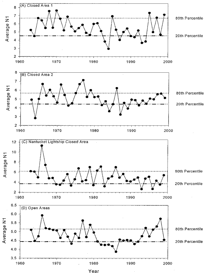
Exhibit 5. Trends in a species diversity index (N1) for three groundfish closed areas (Exhibit 3) and all open areas, 1963-1999. Note that the areas were closed in 1994. Data are based on fish catches from NMFS bottom trawl surveys.
