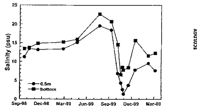
Fig. 2. Surface and bottom water salinities (in psu) at station C-3 in the western PS.
