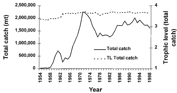
Exhibit 1. Historical estimates of the total groundfish (including halibut and herring) and shellfish catch and trophic level (TL) of the catch in the eastern Bering Sea.
