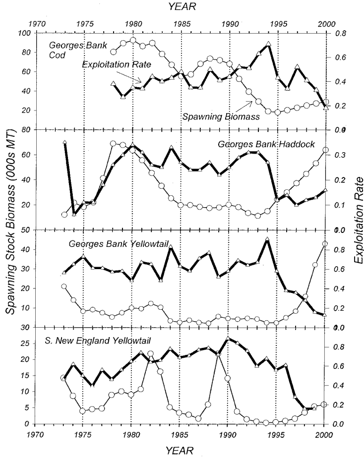
Exhibit 2. Trends in the exploitation rate (proportion of the stock killed by fishing) and spawning stock biomass for four important Northeast groundfish resources.
