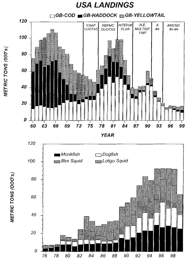
Exhibit 4. Trends in fishery landings for three important traditional New England groundfish stocks (above) and four non-traditional species (below)
