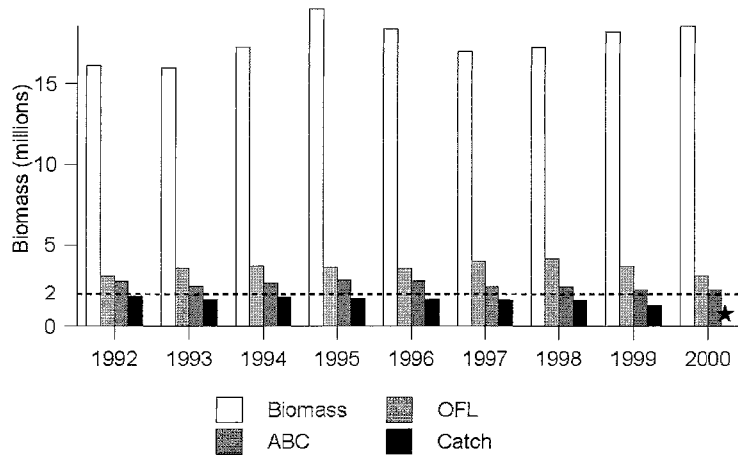
Exhibit 2. Exploitable biomass and catch specifications for Bering Sea and Aleutian Islands groundfish complex, 1992-2000. The dashed line shows the 2 million t optimum yield limit.
