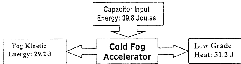
Figure 1. Cold Fog Energy Flow
