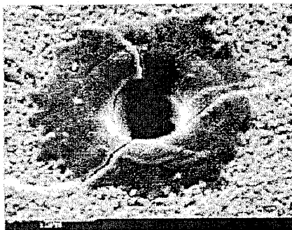
Figure 7. Charge cluster borehole into lead glass. Hole is about 10 micron diameter. Penetration is about 1 mm per kV. The lowest speed clocked has been 1 cm in 50 nanoseconds. With an estimated 100 billion electrons carrying 100,000 positive ions, the kinetic energy exceeds 180 microjoules. It has been suggested that a Casimir effect pushes them together, overcoming Coulomb repulsion of like charges. (photo credit: Ken Shoulders)
