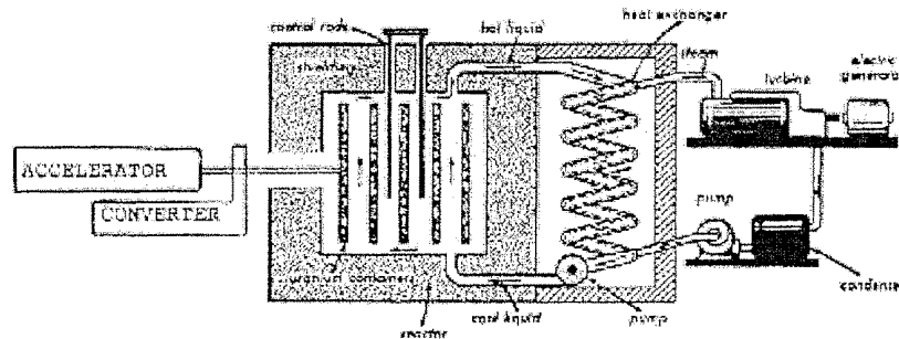
Figure 3. Accelerator Driven Reactor
