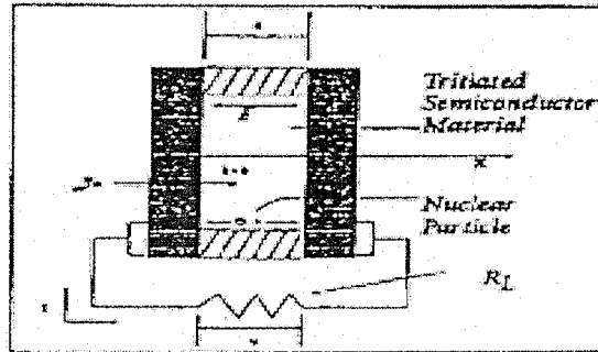
Figure 2. Tritium Battery
