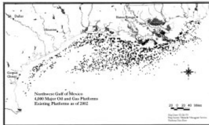
The platforms reside on thousands of sq miles of turbid ocean floor resulting from millions of year of sedimentation from the Mississippi and other tributaries. They provide reef fish in the region hard substrate and the necessary resources for survival.
