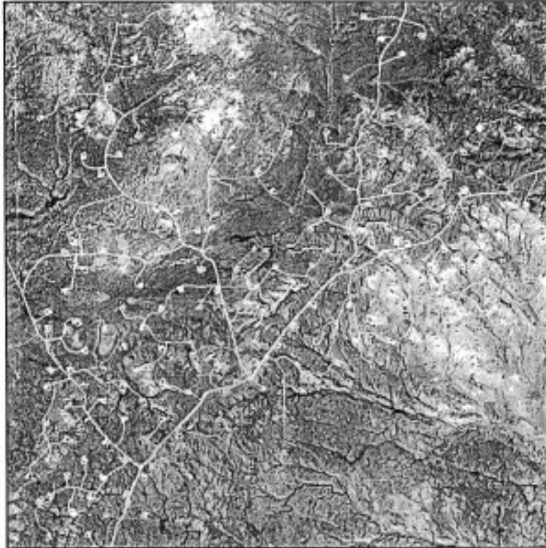
Figure 3. Landsat image of the same area, taken on October 26, 1999 after nearly 150 new gas wells and connecting roads had been installed with 80-acre spacing. Each bright rectangular region is a well pad as seen in Figure 1, representing the location of a single well. Dark spots on many of the pads are open pits containing drilling fluids and produced fluids that are separated from the gas.
