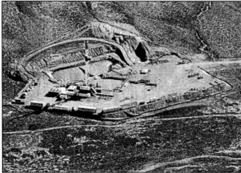
Figure 1. Photograph taken in 2002 of a gas well being drilled on a typical well pad. Note pits containing drilling fluids, equipment trailers, and access road.
