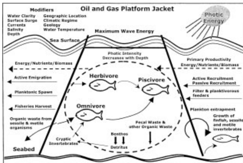
Fig 2. Conceptualized model of trophic dynamics of an oil and gas production platform artificial reef.
