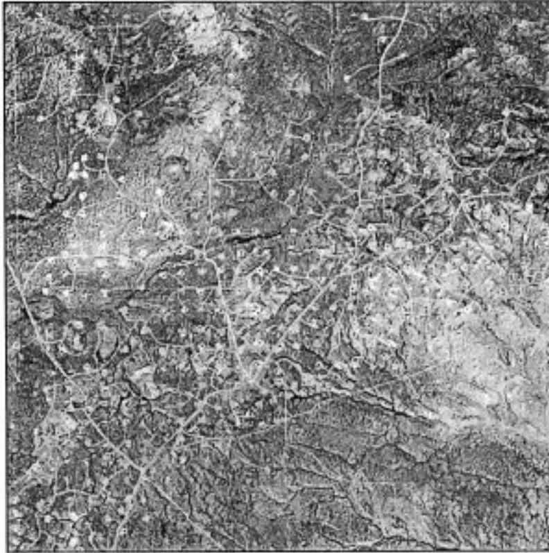
Figure 5. Landsat image taken on October 18, 2002. By this time Jonah field now contains more than 400 gas wells and hundreds of miles of connecting roads. If the infill-drilling proposal is approved, up to 850 new well pads will be added to the field.
