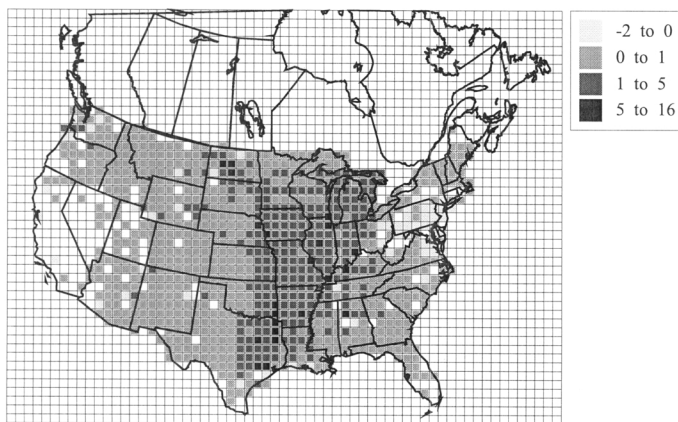
Fig. 5. Simulated percentage change in total deposition of mercury between Scenario 2 and Scenario 1.
