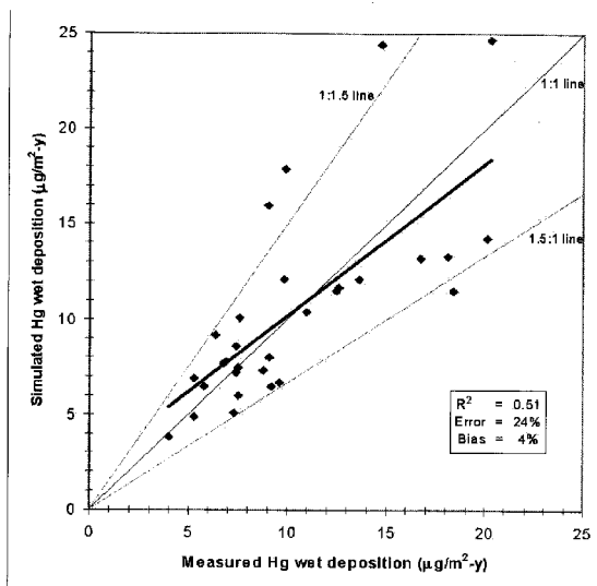
Fig. 2. Comparison of simulated and measured wet deposition fluxes of mercury at MDN sites in 1998.
