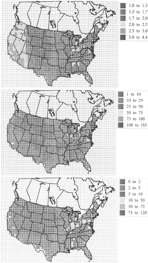
FIGURE 4. U.S. annual-average surface concentrations of Hg(0) (ng/m 3 , top), Hg(II) (pg/m 3 , middle), and Hg(p) (pg/m 3 , bottom).
