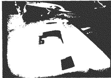
Photograph 19. Test 51502 production roof vehicle with significant roof/pillar deformation
