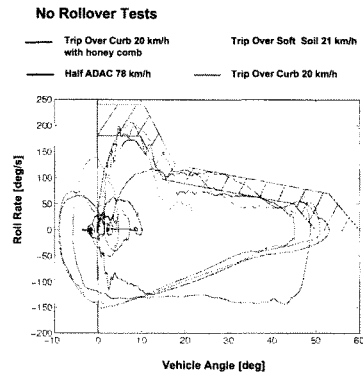
Figure 1b: Measuring vehicle responses in 24 full-scale rollover and non-rollover tests, defining sensor and sensing requirements.
