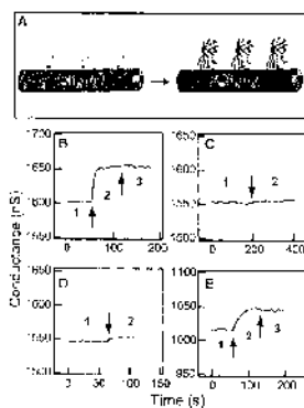
Real-time detection of protein binding: biotin-modified SiNW and subsequent binding of streptavidin (shown approximately to scale). (B) region 2 corresponds to the addition of 250 nM streptavidin, (E) 25 pM streptavidin.
