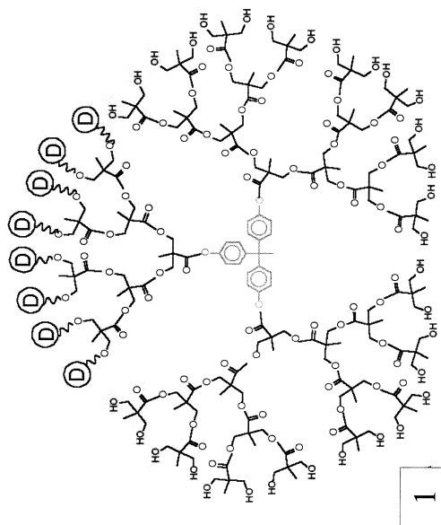
Dendrimer structure, from Jean Frechet, U.C. Berkeley
