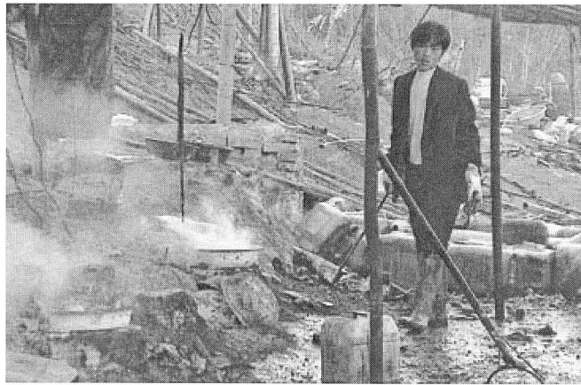
Acid Worker: A laborer heats aqua regia—a mixture of nitric acid and hydrochloric acid—to dissolve tiny amounts of gold from computer chips. The worker inhales acid fumes all day as she swirls computer chips in the mixture. The sludge left over from the process is dumped directly into the Lianjiang River in Guiyu, China.
