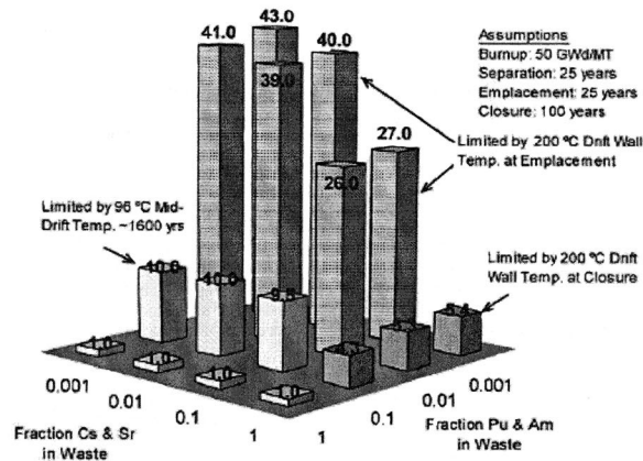
Fig. 7. Potential repository drift loading increase as a function of separation efficiency for plutonium, americium, cesium, and strontium.
