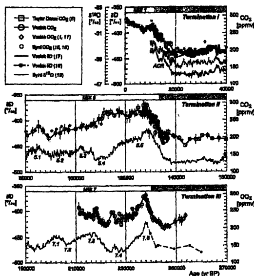
Fig. 1. Records of atmospheric CO 2 concentrations and isotope temperature records derived from the Antarctic Vostok and TD ice cores during the deglaciation and glacialion events around the last three glacial terminations. Error bars in CO 2 concentration data represent 1σ of replicate measurements at the same depth interval. The long-term trend in CO 2 concentrations is indicated by a cubic spline approximation ( P = 5 \times 10^{-7} ) of our data set. For convenience, marine isotope stages (22) are indicated as referred to in the text.
