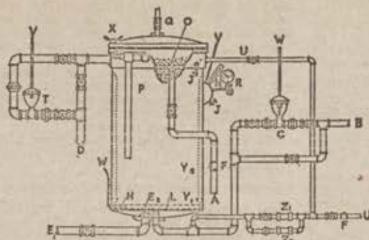
VERTICAL STILL RETORTS FOR WATER PROCESSING
