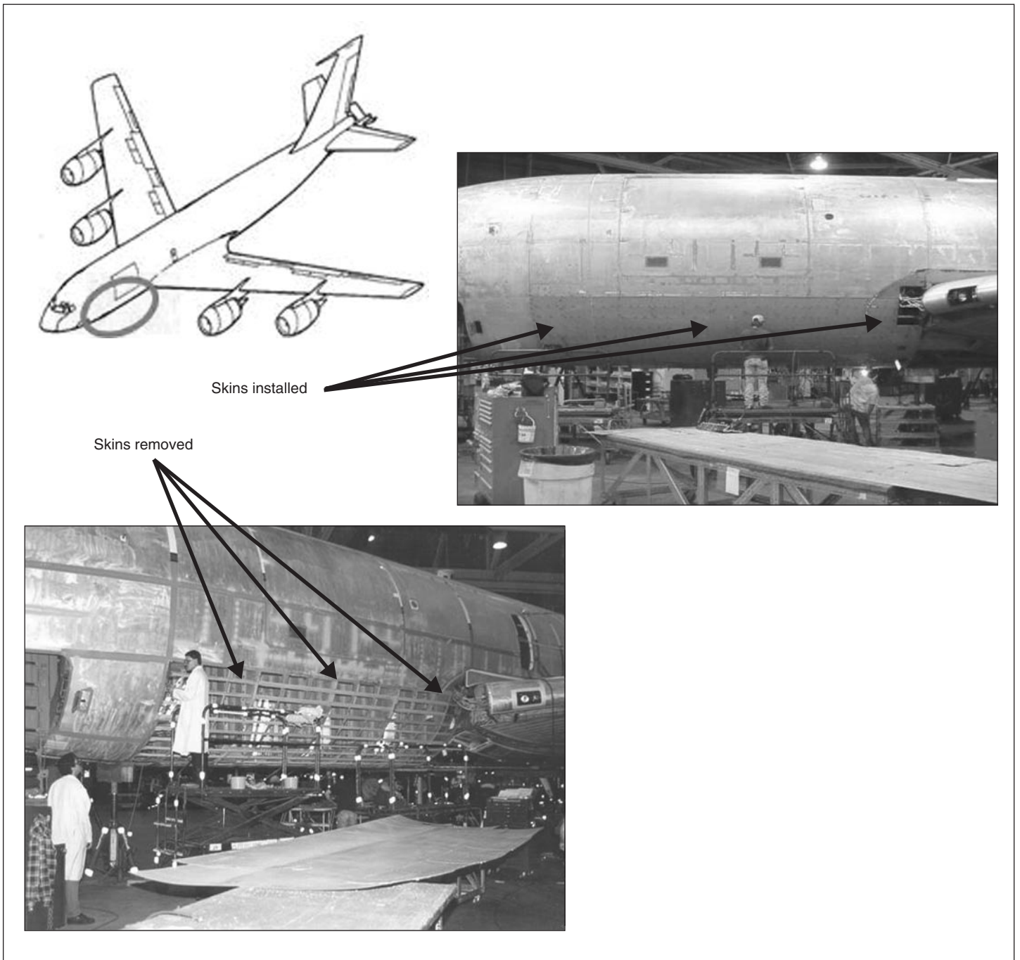
Figure 3: Removal and Replacement of KC-135 Fuselage Skin
