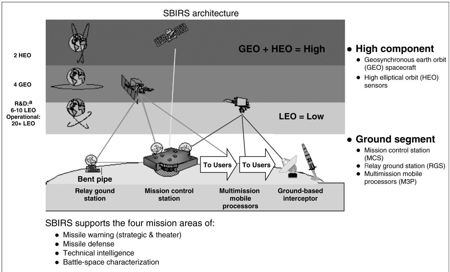
Figure 1: Space-Based Infrared System Description
