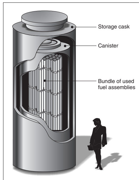
Figure 2: Example of Dry Cask Storage
