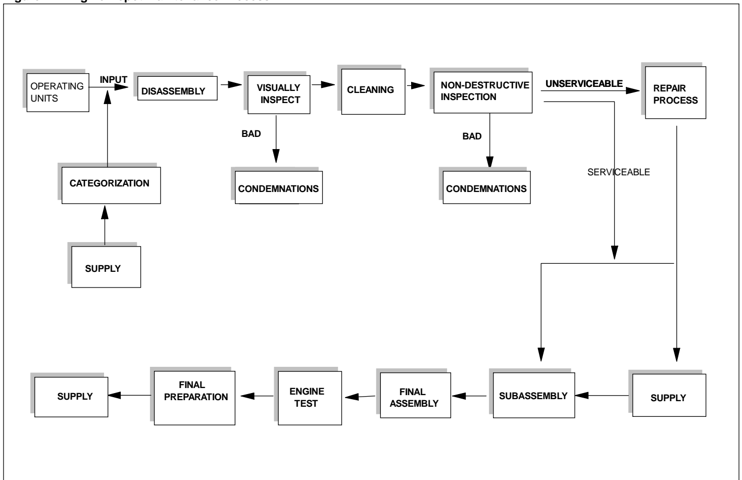
Figure I.1: Engine Depot Maintenance Process
