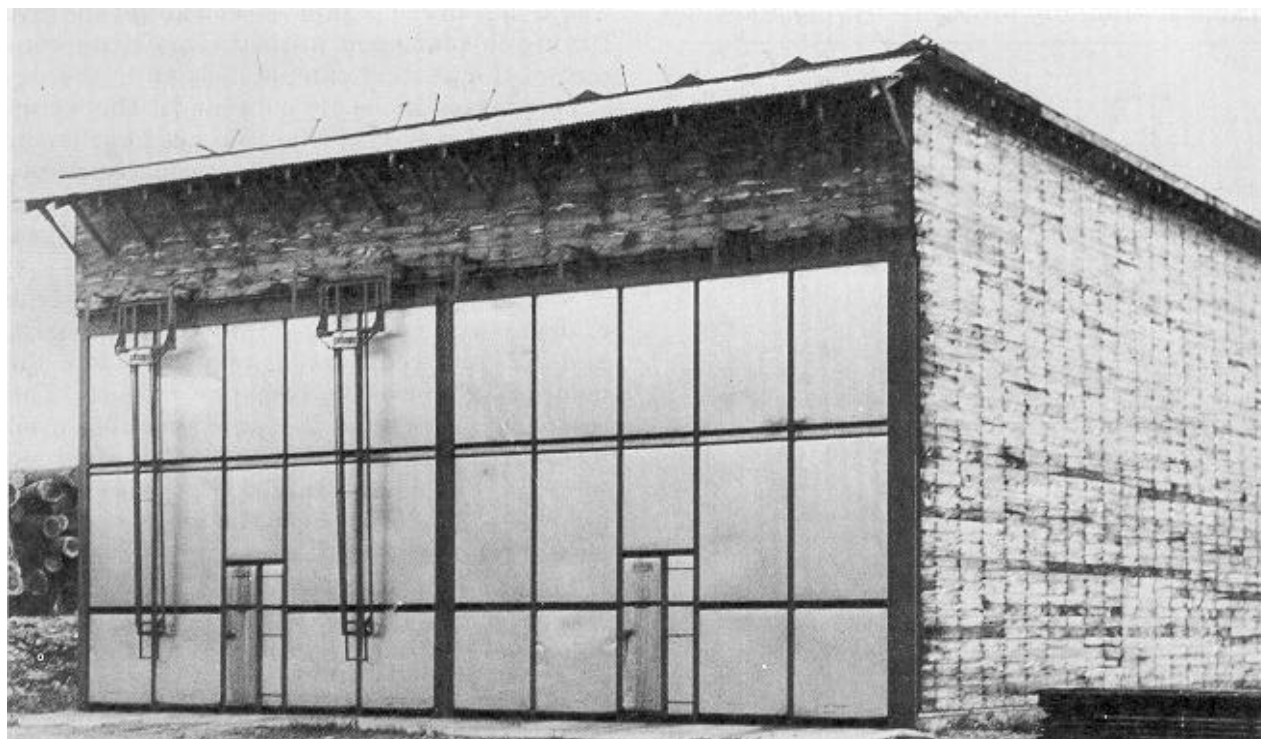
Figure 10.—Low-temperature kiln located at Allegany, N.Y.
