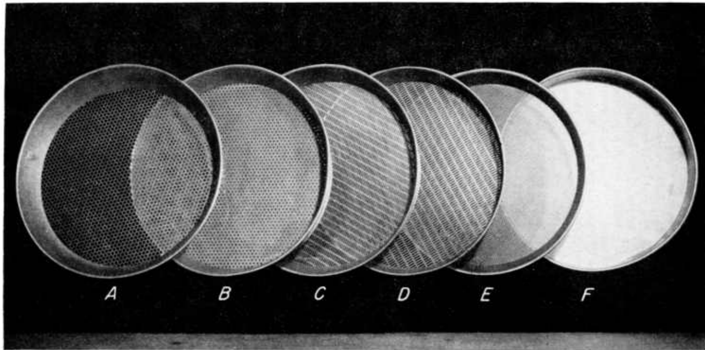
FIGURE 7.—Some of the sieves used to supplement the dockage tester in determining dockage and for removing certain kinds of foreign material from grain; A , Corn sieve with round-hole perforations \frac{1}{4} inch in diameter; B , small buckwheat sieve with triangular perforations the inscribed circles of which are \frac{5}{64} inch in diameter; C , small chess sieve with slotted perforations 0.064 by \frac{3}{8} inch; D , large chess sieve with slotted perforations 0.070 by \frac{1}{2} inch; E , fine-seed sieve with round-hole perforations \frac{1}{12} inch in diameter; F , bottom pan.
