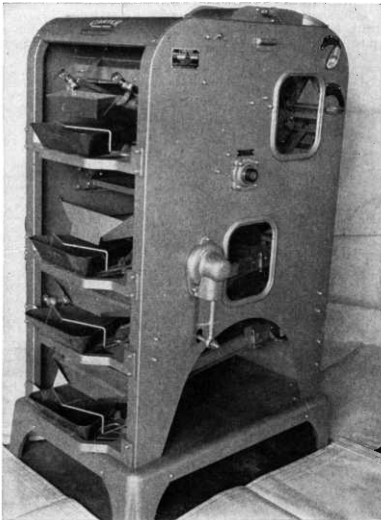
FIGURE 18.—Carter dockage tester, electrically operated. (See figure 20 for details of operation.)
