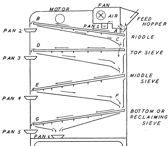
FIGURE 20.—Operations performed by Carter dockage tester on samples of wheat: A , Sample being discharged from feed hopper passes through air stream onto riddle and the material removed by air drops into pan 1; B , tailings (coarse dockage) discharged over riddle drops into pan 2; C , grain that passed through riddle drops into riddle hopper which directs wheat to top sieve, or to middle sieve when no sieve is used in top position; D , clean grain passes over top sieve into pan 3 when top sieve is employed; E , in cases where no top sieve is used, clean grain passes over middle sieve into pan 4, but when the middle sieve is used as a reclaiming sieve, the reclaimed material passes over the sieve into pan 4; F , the material passing through the middle sieve is directed to the bottom sieve for reclaiming or further separation; G , reclaimed material passing over the bottom sieve drops into pan 5; and fine dockage passes through sieve and drops into pan 6.
