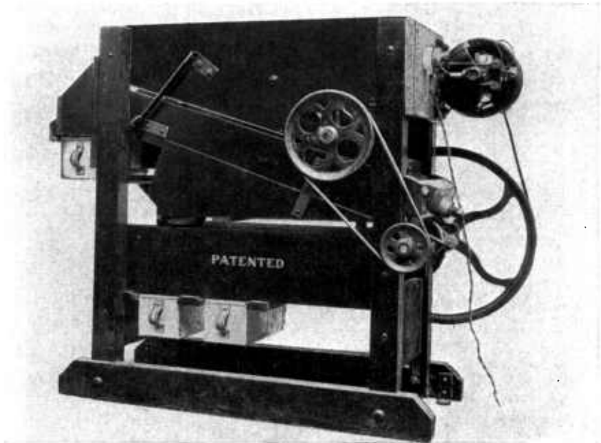
FIGURE 19.—Emerson dockage tester, electrically operated.
