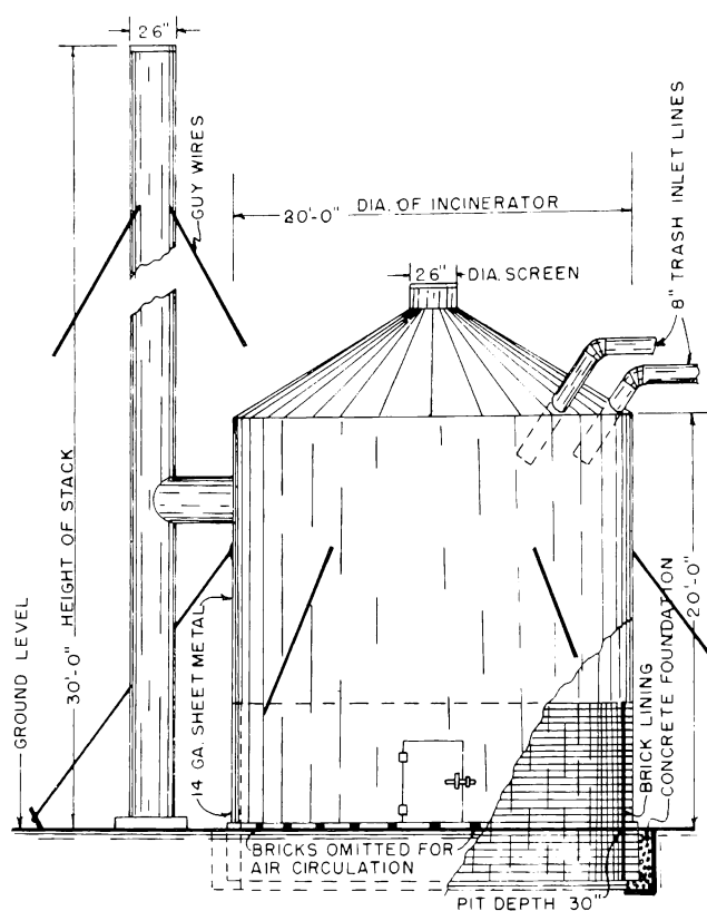
Figure 107.—Boiler plate brick-lined incinerator.
