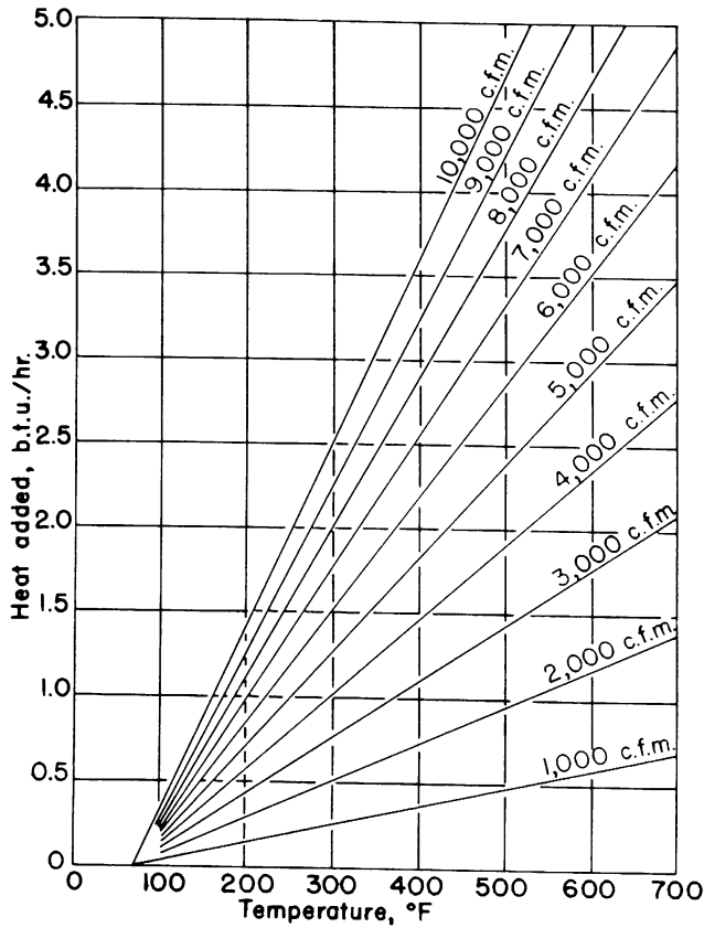
Figure 26.—Temperature effect of adding heat to air moving through a gin drying system.
