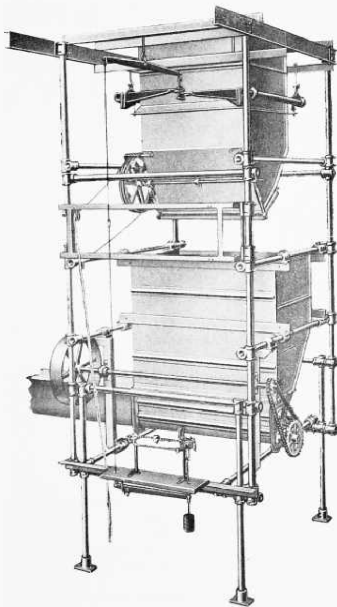
Figure 83.—Cottonseed scales for use in cotton gins.
