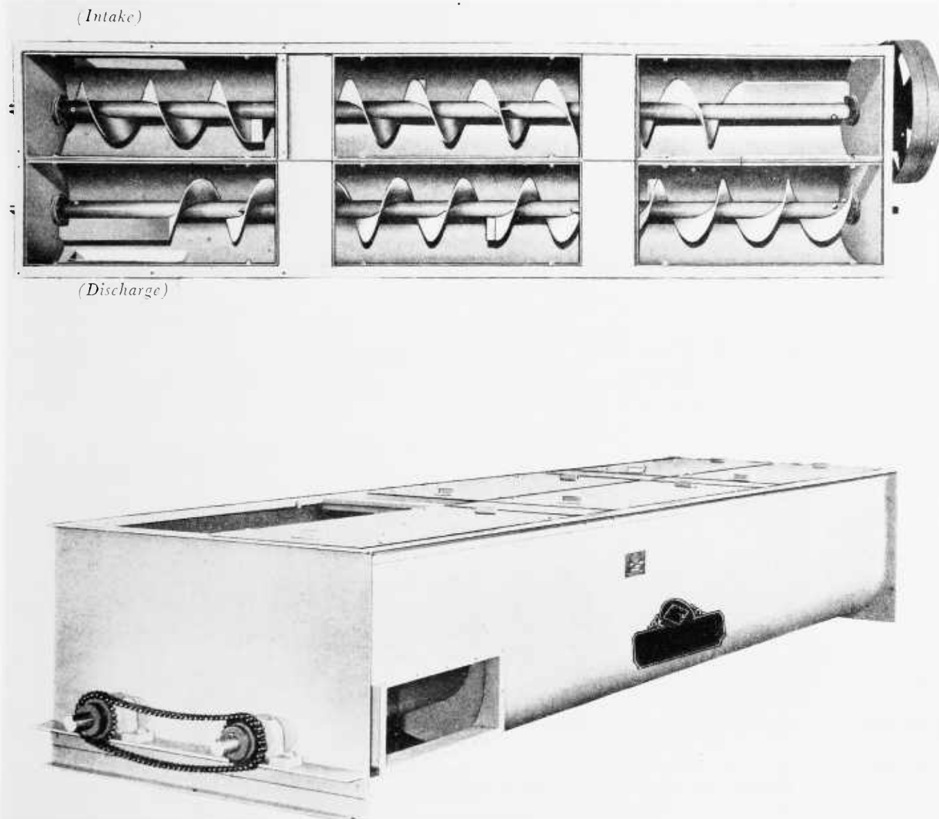
Figure 21. —Top view (with covers off) and oblique view of conveyor-distributor or trough-type drier.
