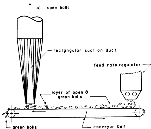
Figure 115.—Experimental green-boll trap.
