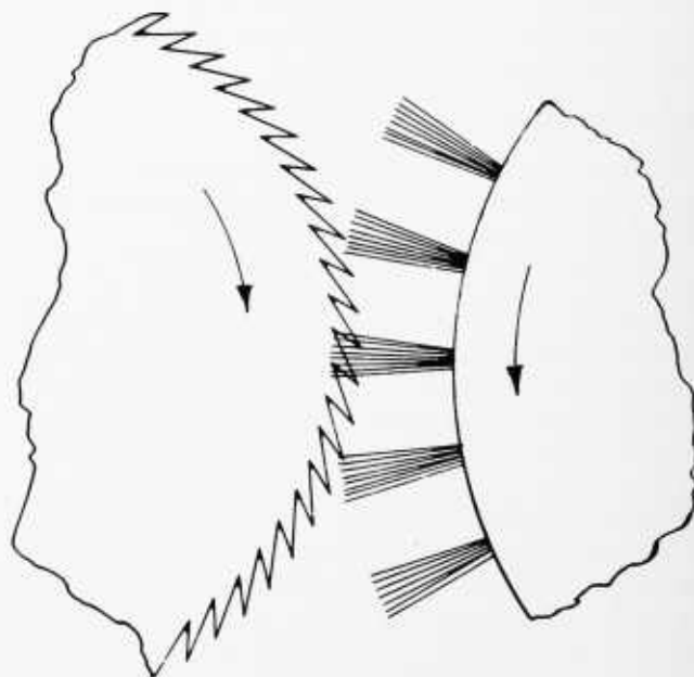
Figure 68.—For proper doffing, the gin brush should be set to mesh with the saw the depth of the saw teeth.
