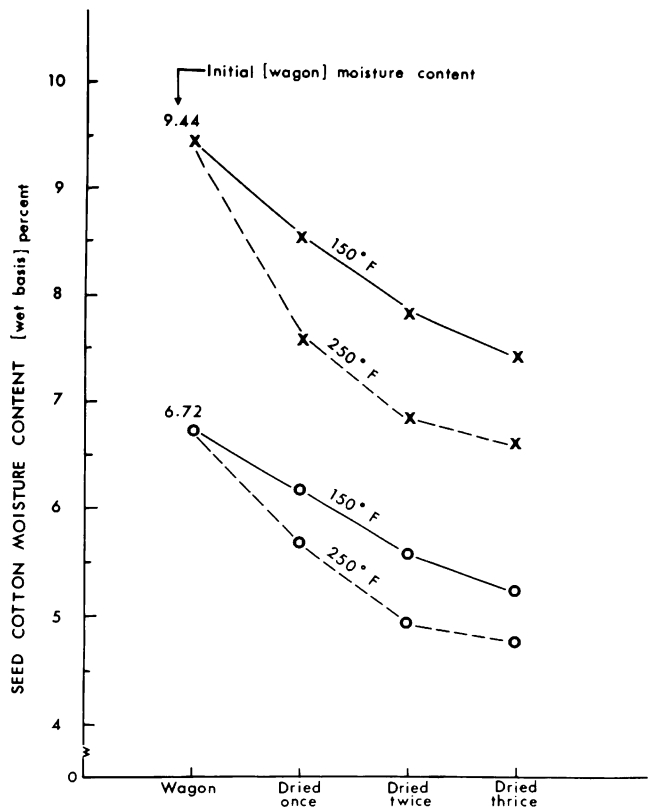
Figure 15.—Seed cotton moisture contents measured on the wagon and after being dried once, twice, and three times in an 18-shelf tower drier using two drying air temperatures and cottons of two different initial moisture contents.
