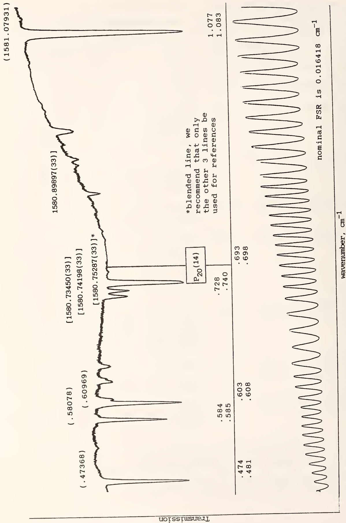
Fig. A-1. Nitrogen dioxide spectra in the vicinity of the P 20 (14) CO laser line at 1580.77335 cm -1 .
