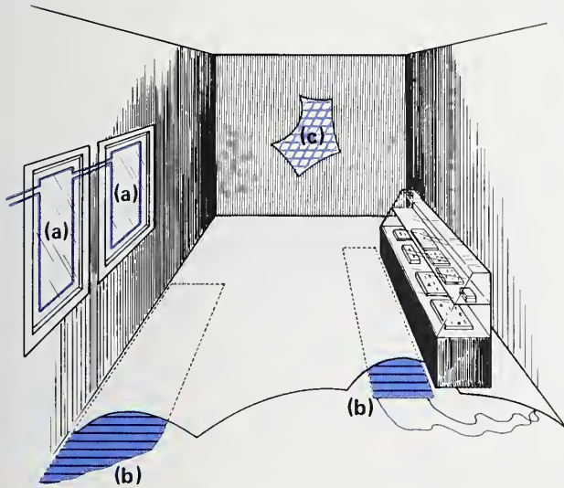
Metallic foil (a) breaks when the glass is broken; this triggers an alarm. Pressure mats (b) respond to pressure; they cause an alarm when stepped upon. Concealed wire screens or grids (c) respond to forced entry through walls, ceilings, doors, etc.
