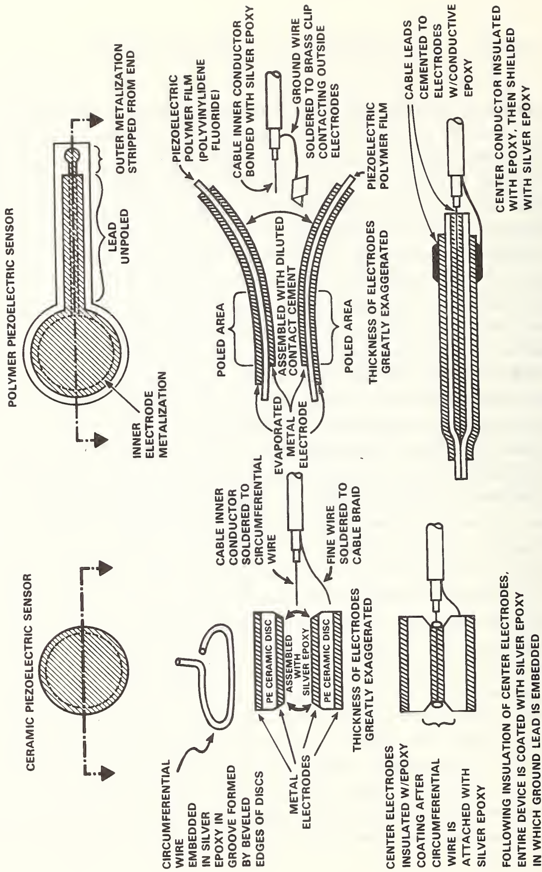
FIGURE A-1. Construction of piezoelectric sensors. Electrodes (metalization) shown shaded.
