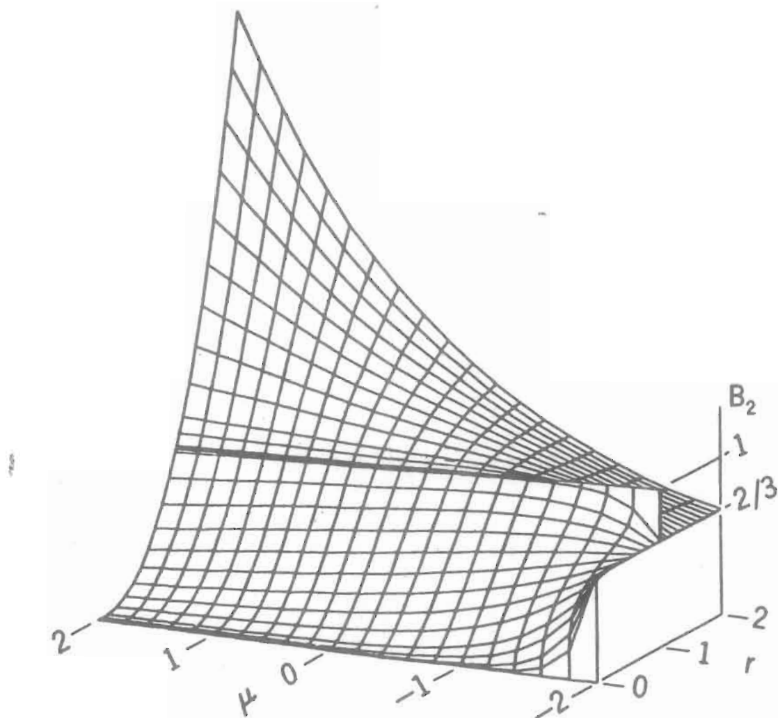
THE BIAS FUNCTION, B_2(r, \mu)
