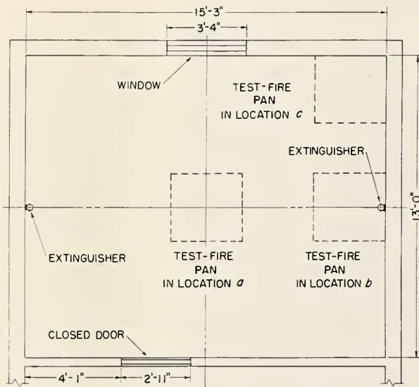
FIGURE 2. Plan for first series of trials of devices A to F as automatic extinguishers.
