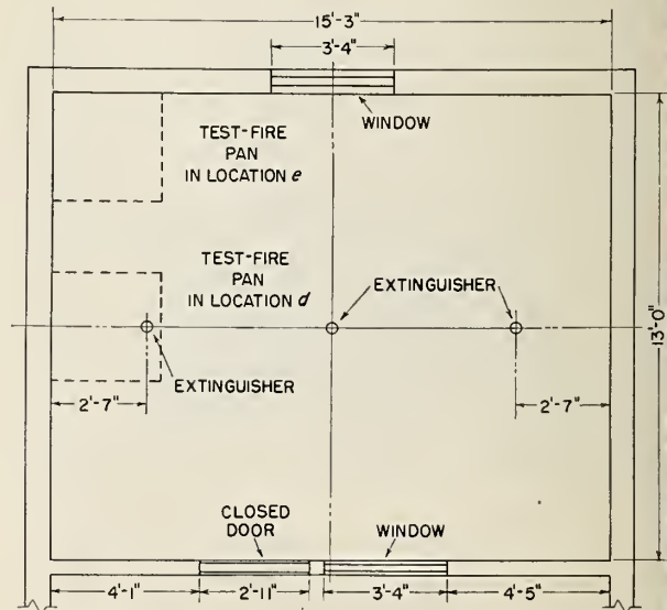
FIGURE 6. Plan for trials of automatic extinguisher G on oil fire on floor. Three extinguisher units used, 3-foot-square test-fire pan.
