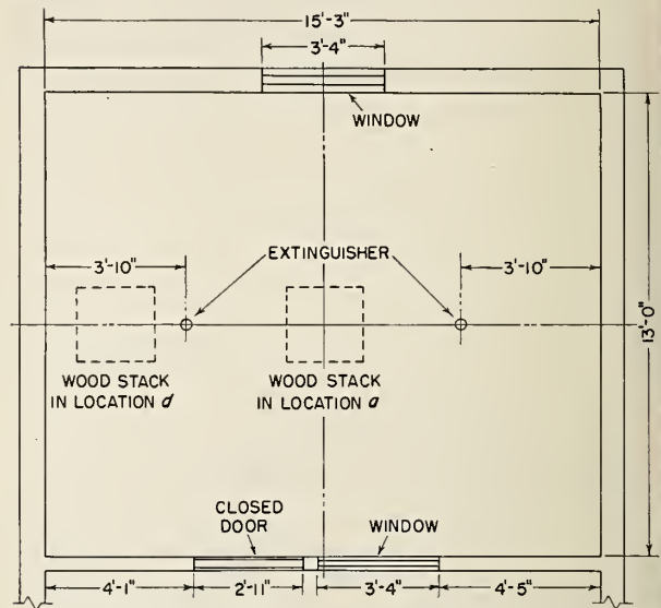
FIGURE 5. Plan for trials of automatic extinguisher G on wood fire. Two extinguisher units used.
