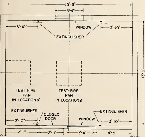
FIGURE 4. Plan for second series of trials of devices A to F as automatic extinguishers.
