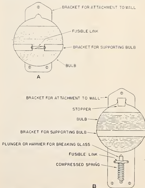
FIGURE 1. General character of two styles of the extinguishers tested. A, Drop-on-floor type; B, Spring-operated type.
