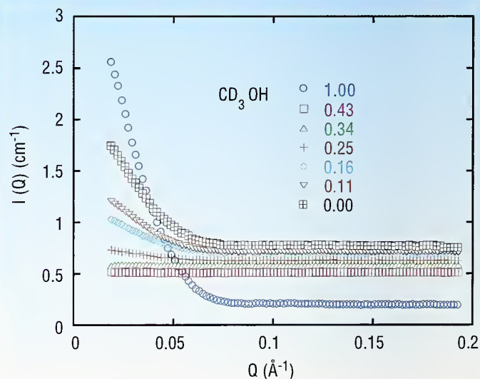
FIGURE 2. SANS from G8 dendrimer in CD 3 OH/CH 3 OH mixtures.
