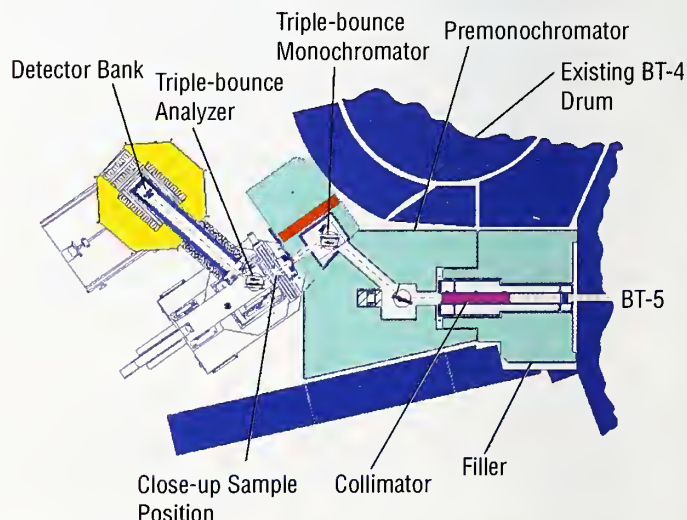
FIGURE 3. Schematic layout of the BT-5 perfect crystal diffractometer.
