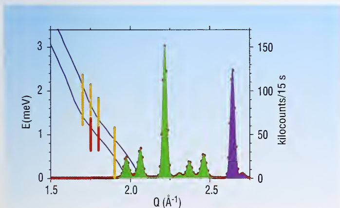
FIGURE 2. The dispersion along the growth direction ( c -axis) measured for the [\text{Dy}_{48}\text{Y}_{23}\text{350}] superlattice is plotted against the energy scale on the left side. It is compared to the measured dispersion in bulk dysprosium (solid lines) expected to originate from each of the superlattice magnetic Bragg peaks. (Only the negative Q branches from the two low Q Bragg peaks are shown). On the right side the diffraction scan for this sample showing the superlattice peaks is displayed. This film is so large that the sample diffraction peaks are as strong as the substrate peak shown in blue on the right.
