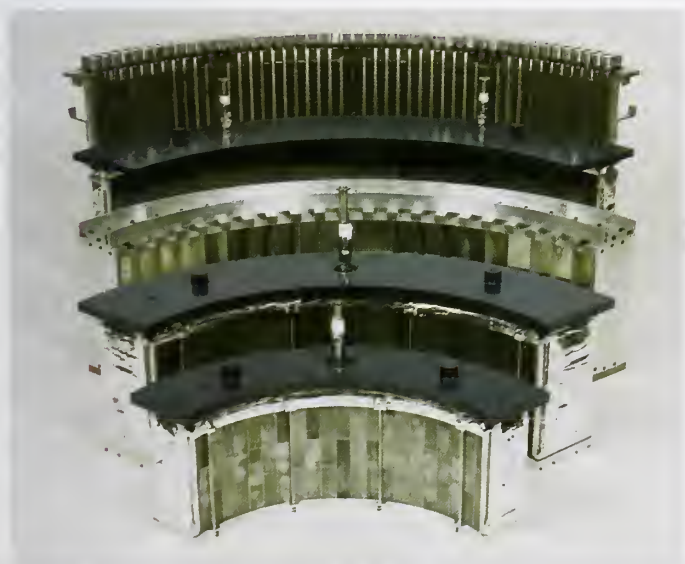
FIGURE 4. The FANS filter assembly. The first Be filter is in the foreground with the PG filter second and the final Be filter is in the background just before the detector bank. A radial collimator is visible in the middle of the assembly.
