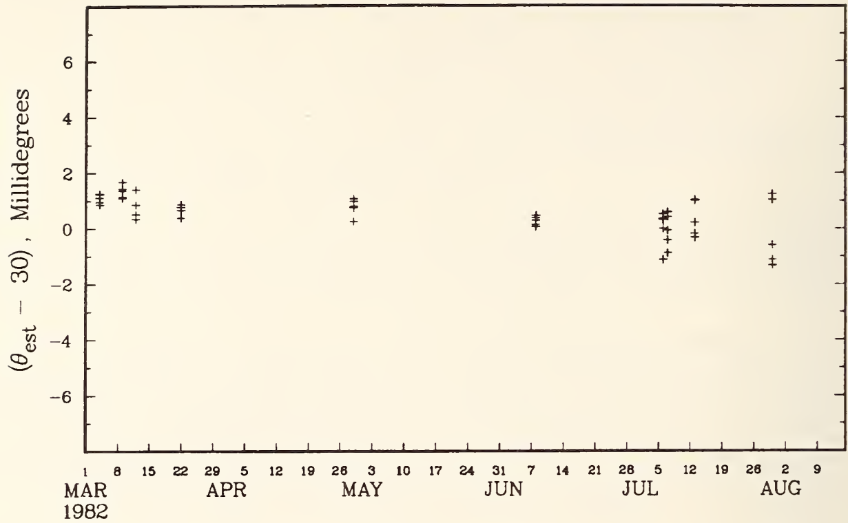
Figure 17-1B. Bearing angle offsets at 30 degrees.
