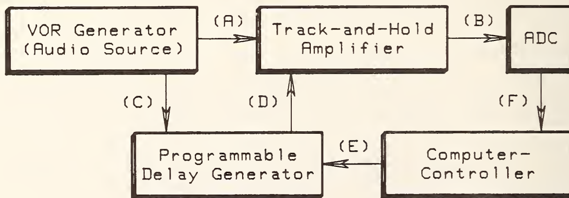
Figure 13-1. Simplified block diagram of the phasemeter.
