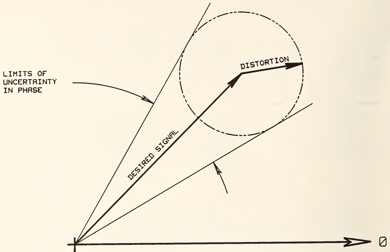
Figure 8-2. Relationship between amplitude distortion and phase uncertainty.
