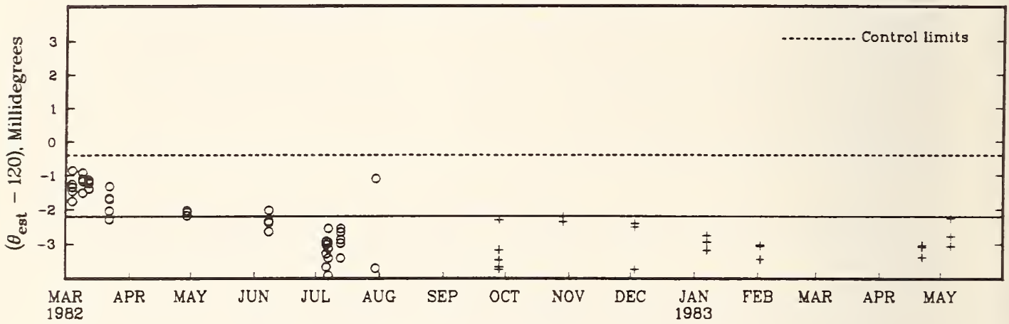
Figure 18-2C. Control chart of offsets at 120 degrees.
