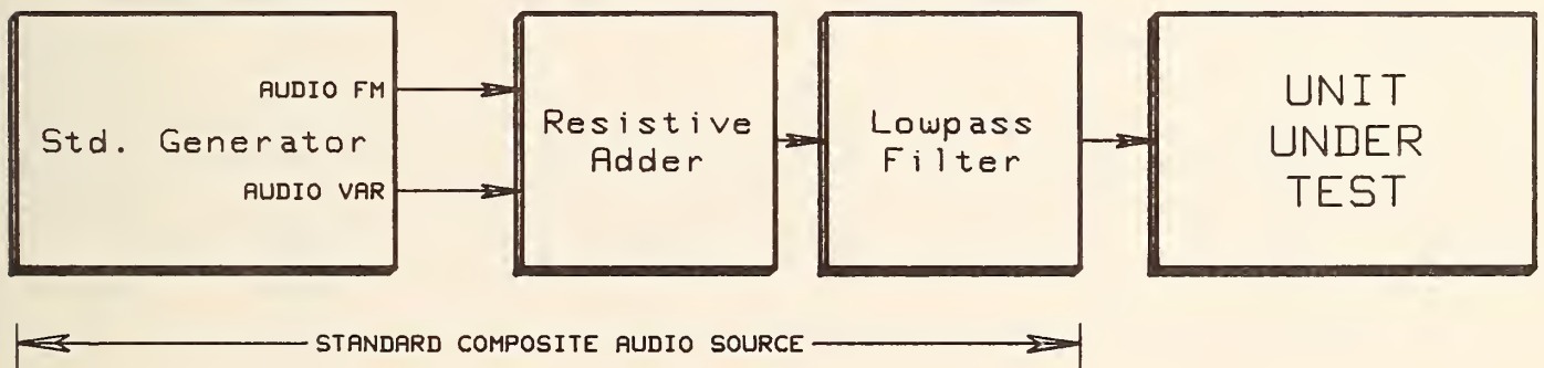
Figure 7-1. Connecting the standard VOR generator, adder, and filter to a unit under test.
