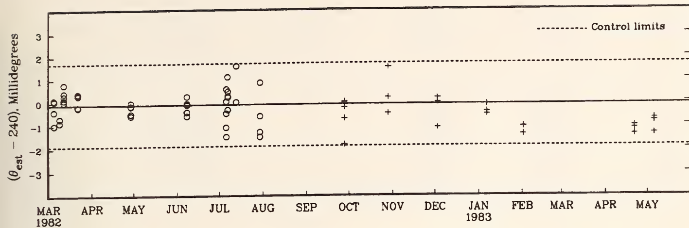
Figure 18-2E. Control chart of offsets at 240 degrees.
