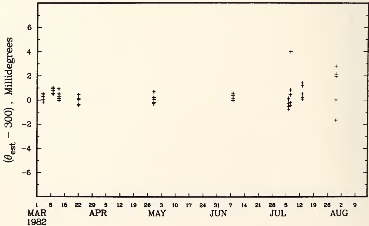
Figure 17-1K. Bearing angle offsets at 300 degrees.
