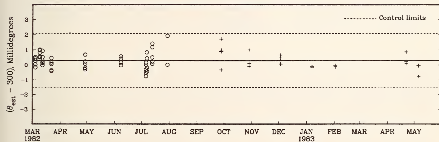
Figure 18-2F. Control chart of offsets at 300 degrees.
