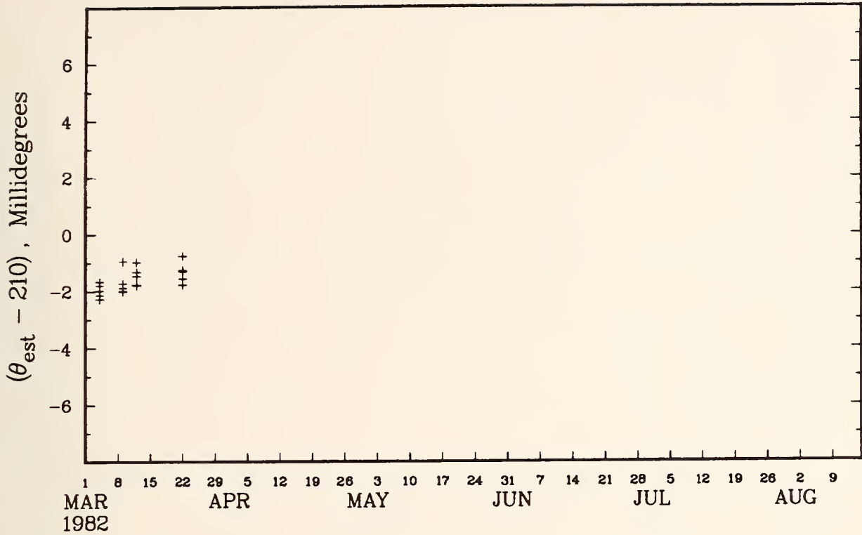
Figure 17-1H. Bearing angle offsets at 210 degrees.
