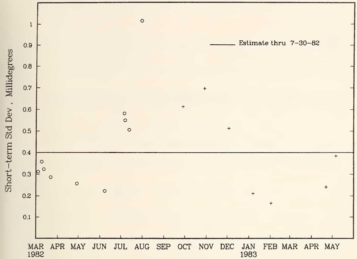
Figure 18-1. Control chart for short-term standard deviation.
