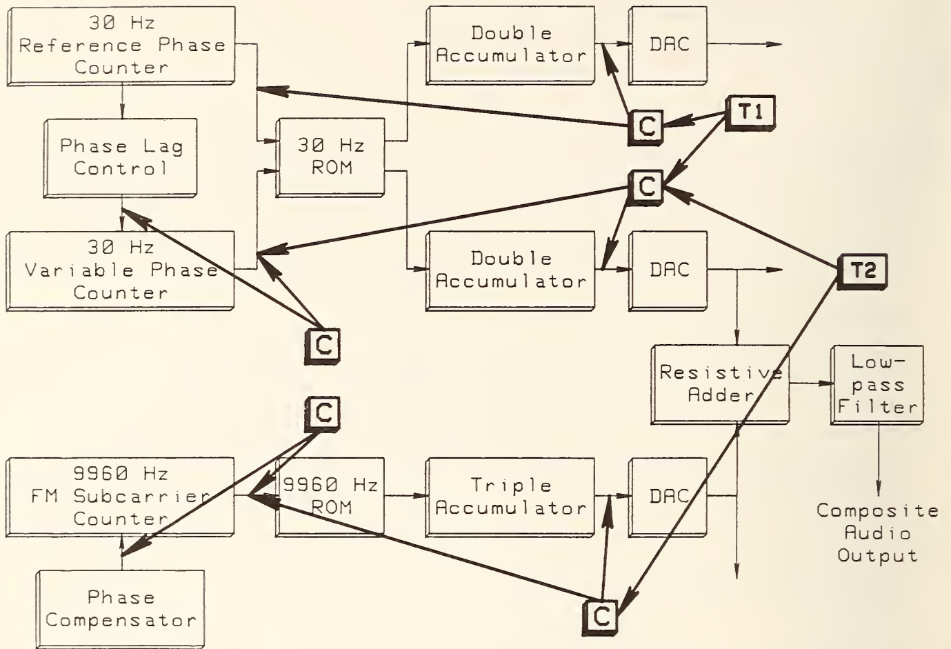
Figure 6-1. Error detection circuits. Digital comparisons are made between the pairs of digital signal paths as indicated by the heavy arrows. Clock is not shown.
