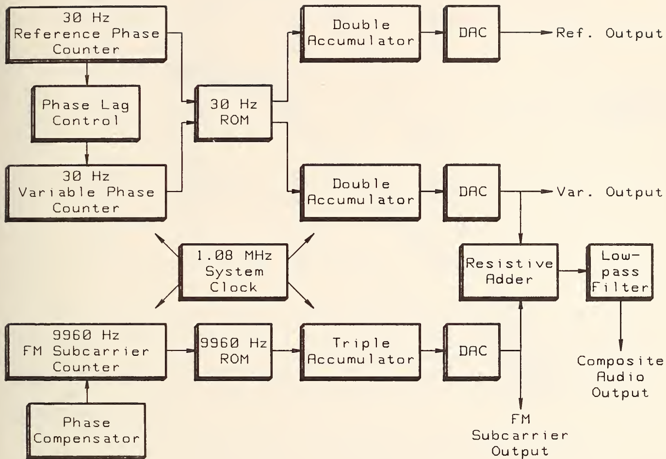
Figure 8-1. Overall generator block diagram.
