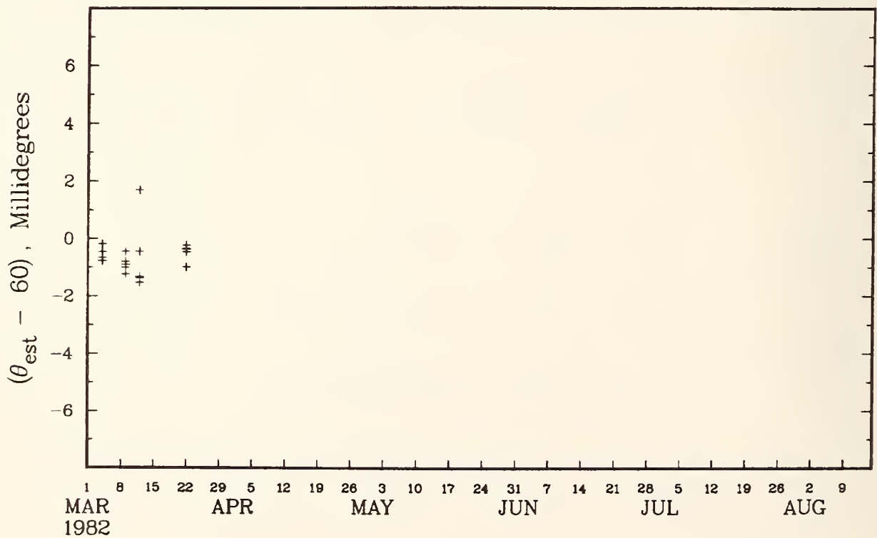
Figure 17-1C. Bearing angle offsets at 60 degrees.
