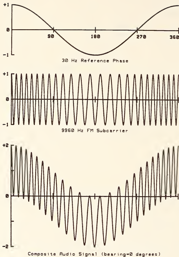
Figure 2-3. Simulated 30 Hz and 9960 Hz waveforms. Time is distorted for clarity.
