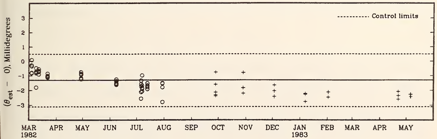
Figure 18-2A. Control chart of offsets at 0 degrees.
