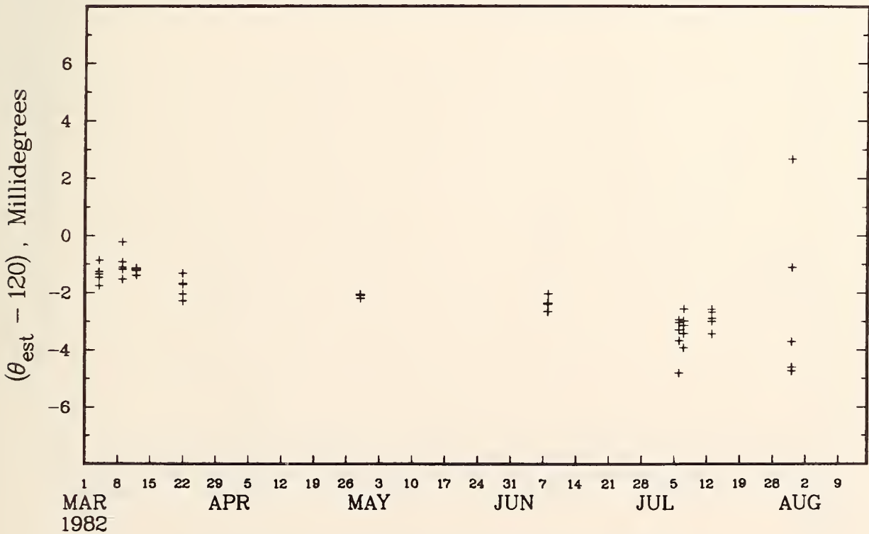
Figure 17-1E. Bearing angle offsets at 120 degrees.
