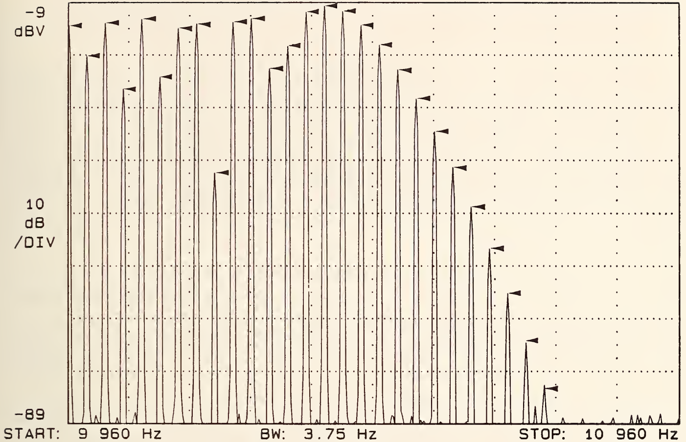
Figure 10-1. Partial 9960 Hz spectrum. Arrows indicate computed amplitude.
