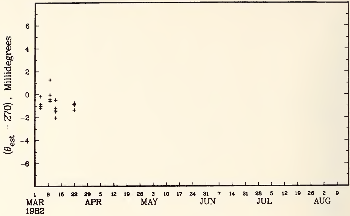
Figure 17-1J. Bearing angle offsets at 270 degrees.
