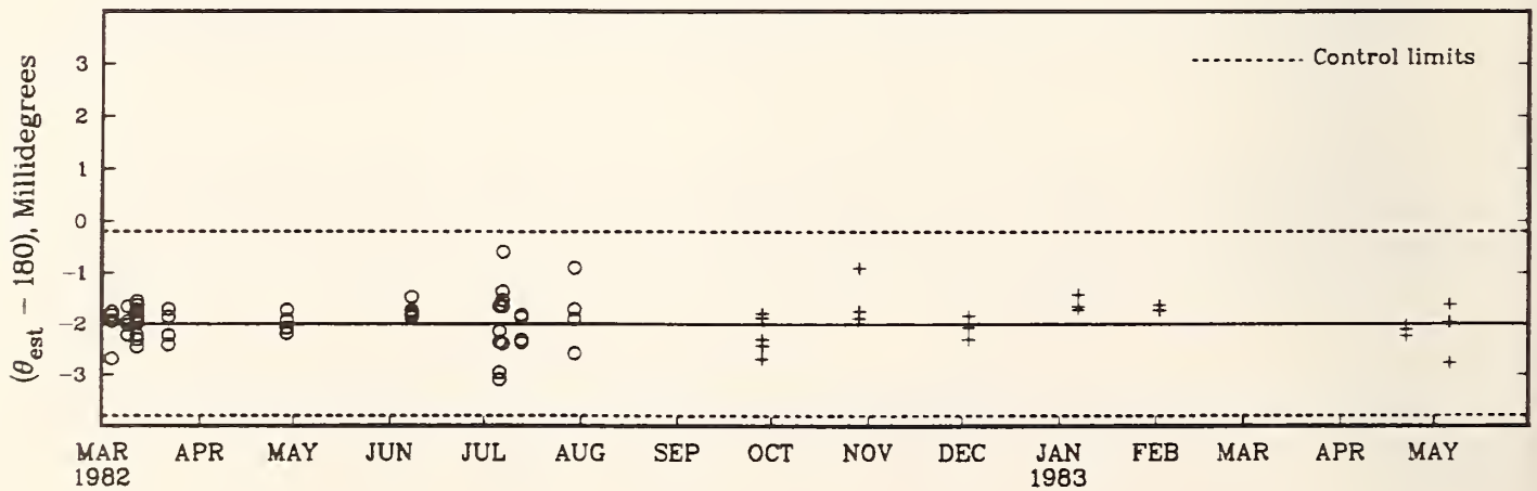
Figure 18-2D. Control chart of offsets at 180 degrees.
