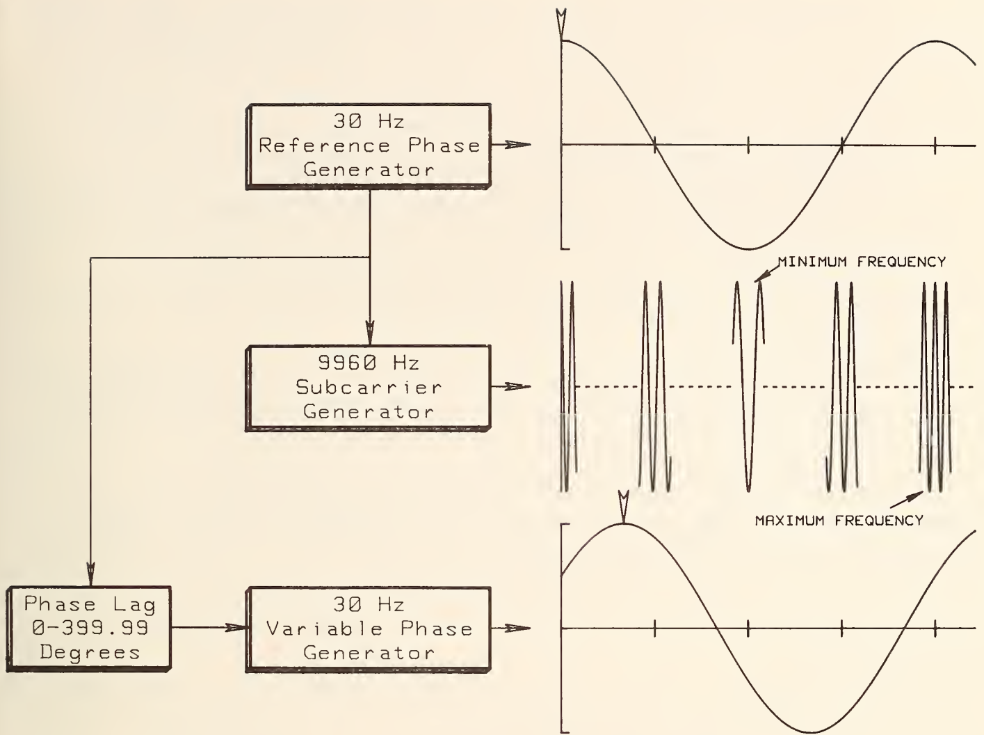
Figure 5-1. Simplified block diagram of generator.
