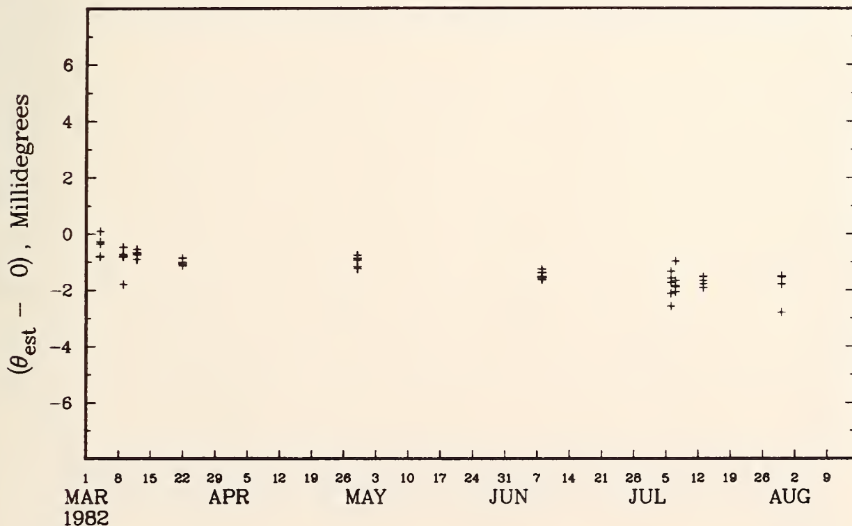
Figure 17-1A. Bearing angle offsets at 0 degrees.
