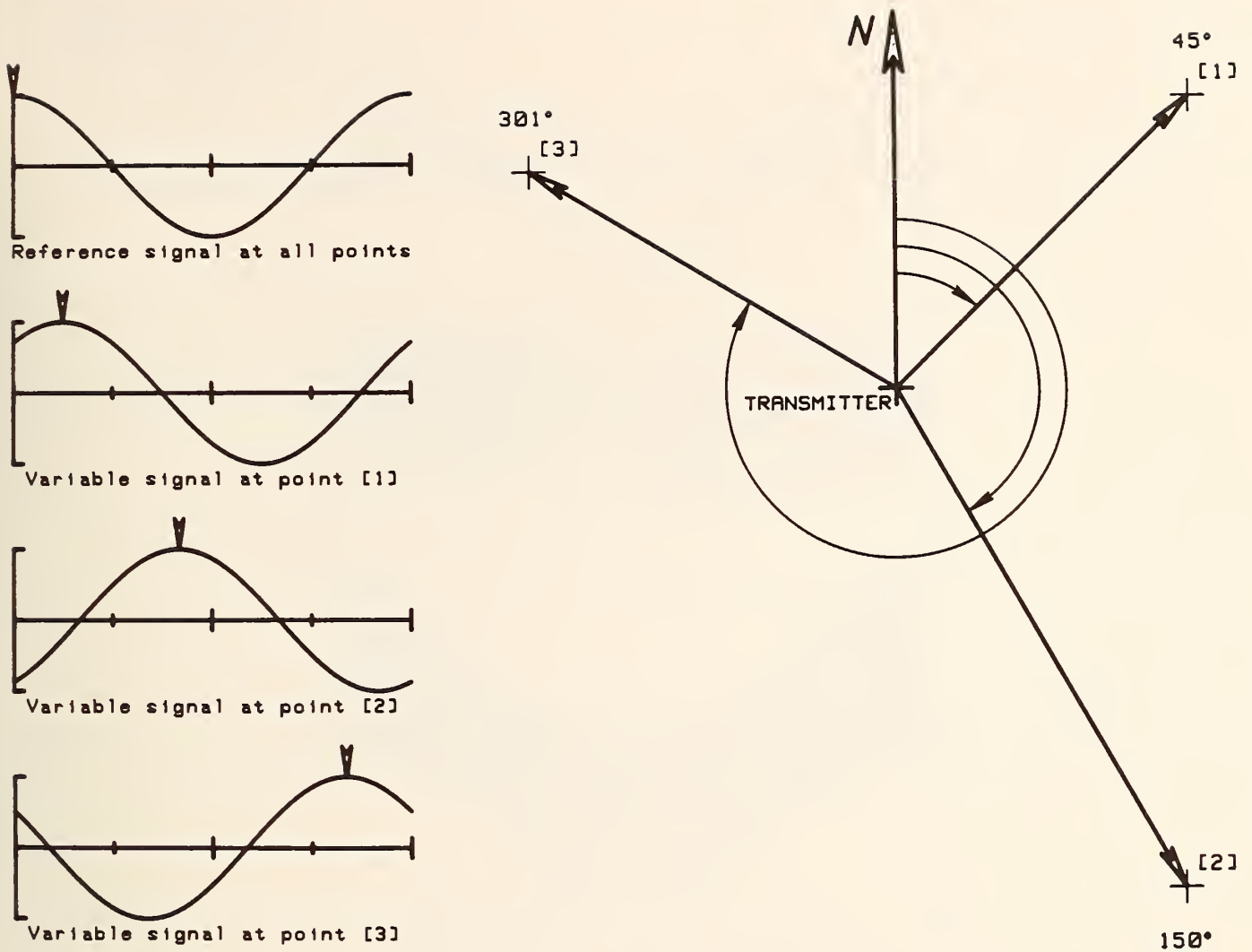
Figure 2-2. Reference and variable phase signals as received at three typical locations.
