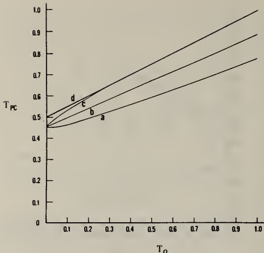
Threshold T_{PC} corresponding to edge location for coherence parameter R = 2 as a function of T_0 ( I_0/I_M ). Curve-to-curve parameter is optical phase difference \phi_0 : a) \pi , b) \pi/2 , c) 0. The 50% incoherent edge detection threshold is shown (curve d) for comparison.
