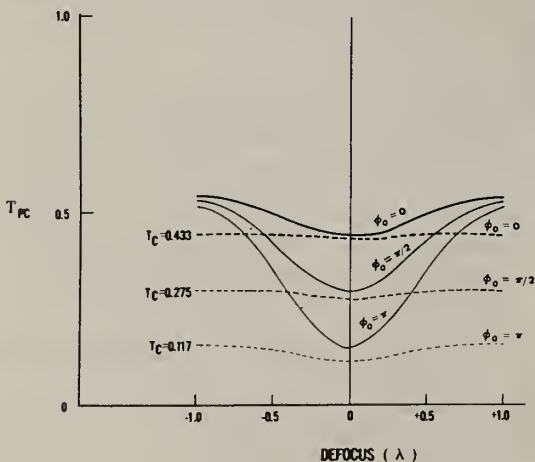
Variation of T_{PC} with defocus parameter a_2 for T_0 = 0.1 , for different R values: dashed lines R = 1/5 , solid lines R = 2/3 . The coherent edge detection threshold T_C is indicated in each case and is equivalent to the value of T_{PC} for zero defocus and R = 1/5 .
