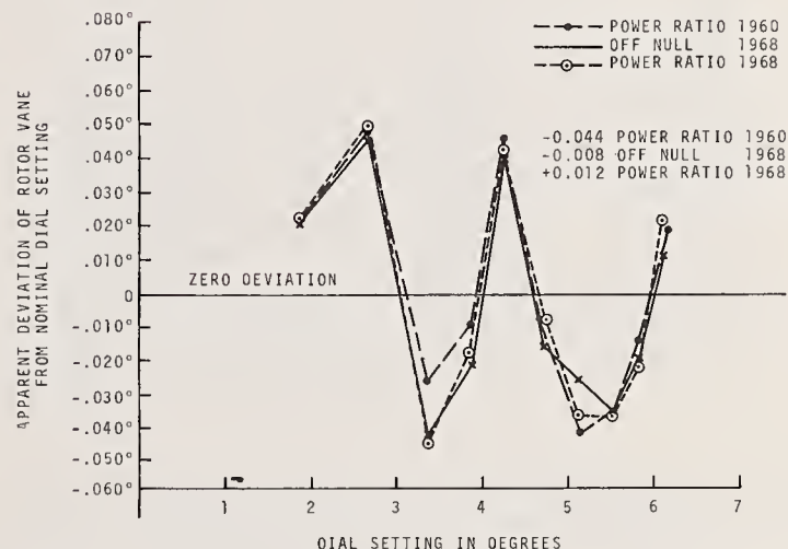
FIGURE 16. Apparent deviation of rotor vane in degrees from nominal at each dial setting in degrees.
