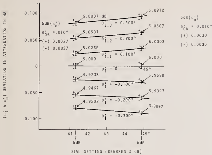
FIGURE 70. Deviations in attenuation from nominal in decibels versus dial setting in degrees and decibels (for 5 to 6 dB) when \theta_1' equal \pm 0.100 , \pm 0.200 , and \pm 0.300^\circ , and \theta_0' equal \pm 0.010^\circ .
