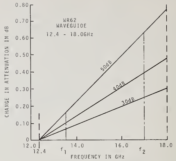
FIGURE 56. Limits of magnitude of one-sigma error in attenuation versus frequency in GHz for seven WR62 rotary-vane attenuators at 30, 40, and 50-dB dial settings.
