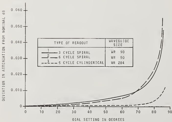
FIGURE 11. Graph of the deviation in attenuation from nominal versus dial setting in degrees which corresponds to a linear deviation of 0.020" for three rotary-vane attenuators.
