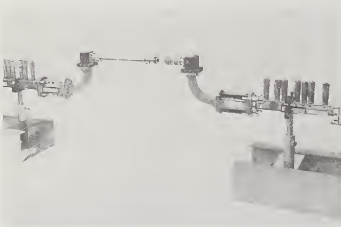
FIGURE 77. Photo of a fixed coaxial attenuator under test being inserted into the line at the coaxial insertion point.
