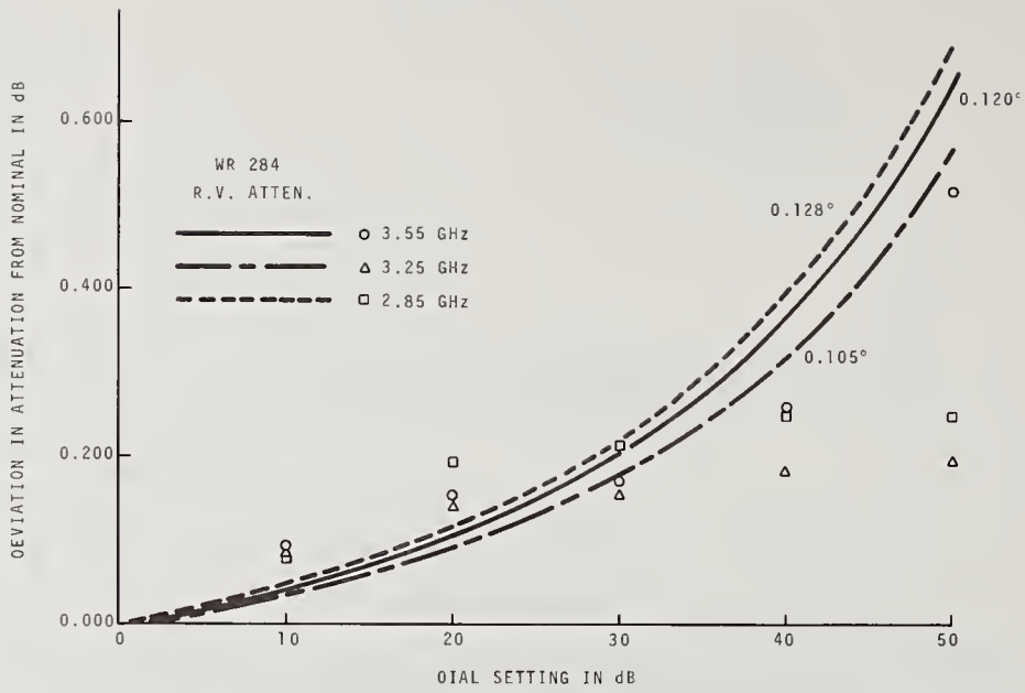
FIGURE 49. Deviation of attenuation for average vane-angle errors of 0.128, 0.105, and 0.120° versus dial setting in decibels at 2.85, 3.25, and 3.55 GHz.
