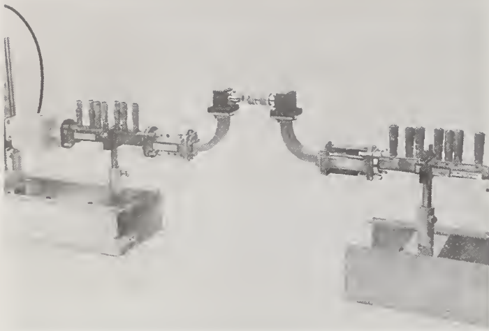
FIGURE 76. Photo of the rectangular waveguide with adapters to admit coaxial devices at the insertion point.
