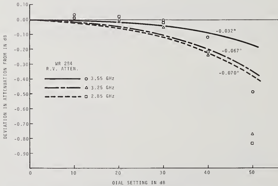
FIGURE 50. Deviation of attenuation for average vane-angle errors of -0.070, -0.067, and -0.032° versus dial setting in decibels at 2.85, 3.25, and 3.55 GHz.
