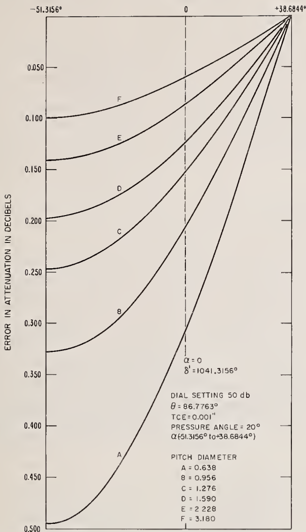
FIGURE 25. Errors in attenuation at the dial setting of 50 dB versus the angle \alpha for different pitch diameters.
