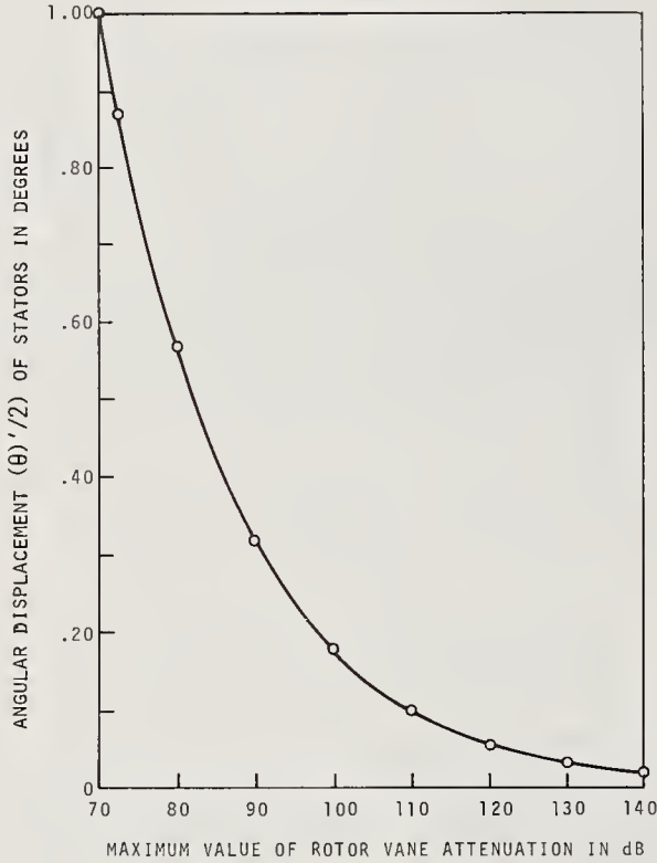
FIGURE 33. Estimated angular displacement of stators in degrees versus the maximum attenuation value of rotor vane in decibels for the compensation required to approach theoretical \cos^2 \theta law.
