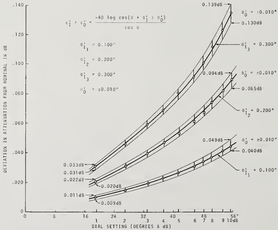
FIGURE 69. Deviations in attenuation from nominal in decibels versus dial setting in degrees and decibels for \theta'_1 equal 0.100, 0.200, and 0.300°, and \theta'_0 equal \pm 0.010 .
