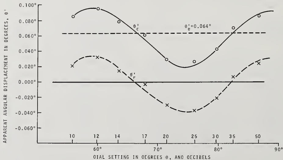
FIGURE 18. Graphs of the cyclic pattern of angular displacement curve, \theta'_c , with average vane-angle error of +0.064^\circ and \theta'_r with -0.064^\circ correction.
