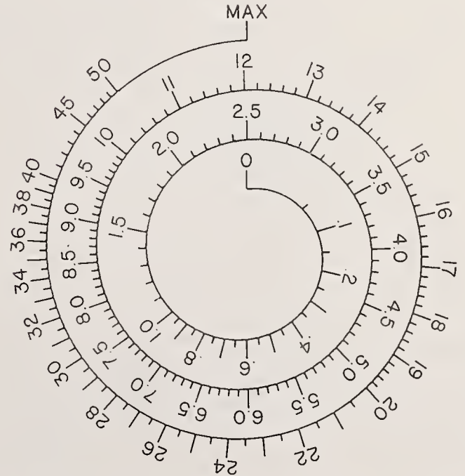
FIGURE 8. Rotary-vane attenuator dial readout in decibels—spiral—3 cycle.
