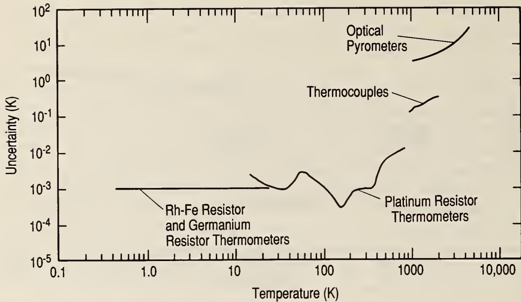
Figure 3. Uncertainties for NIST temperature calibrations.
