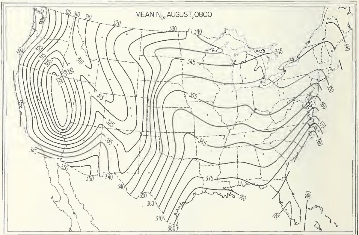
FIGURE 38. \bar{N}_o , August, 0800 local time.
