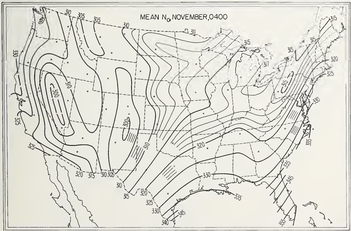
FIGURE 48. \bar{N}_o , November, 0400 local time.
