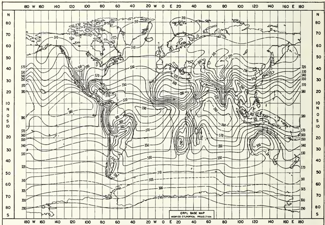
FIGURE 90. Yearly minimum \bar{N}_0 .
