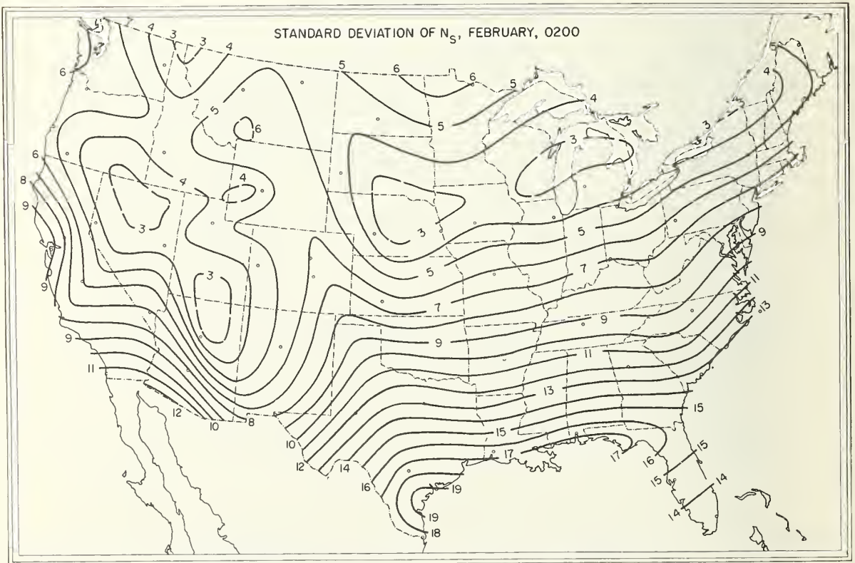
FIGURE 82. \sigma(N_s) : February, 0200 local time.
