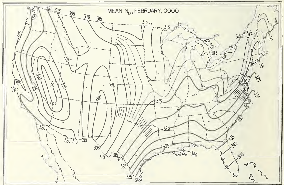
FIGURE 10. \bar{N}_0 , February, 0000 local time.
