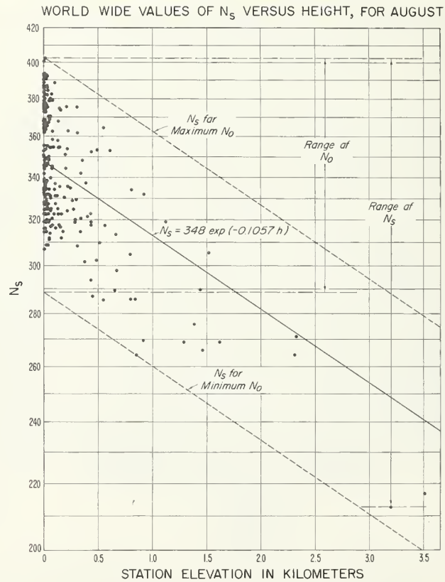
FIGURE 86. Worldwide \bar{N}_s versus height for August.
