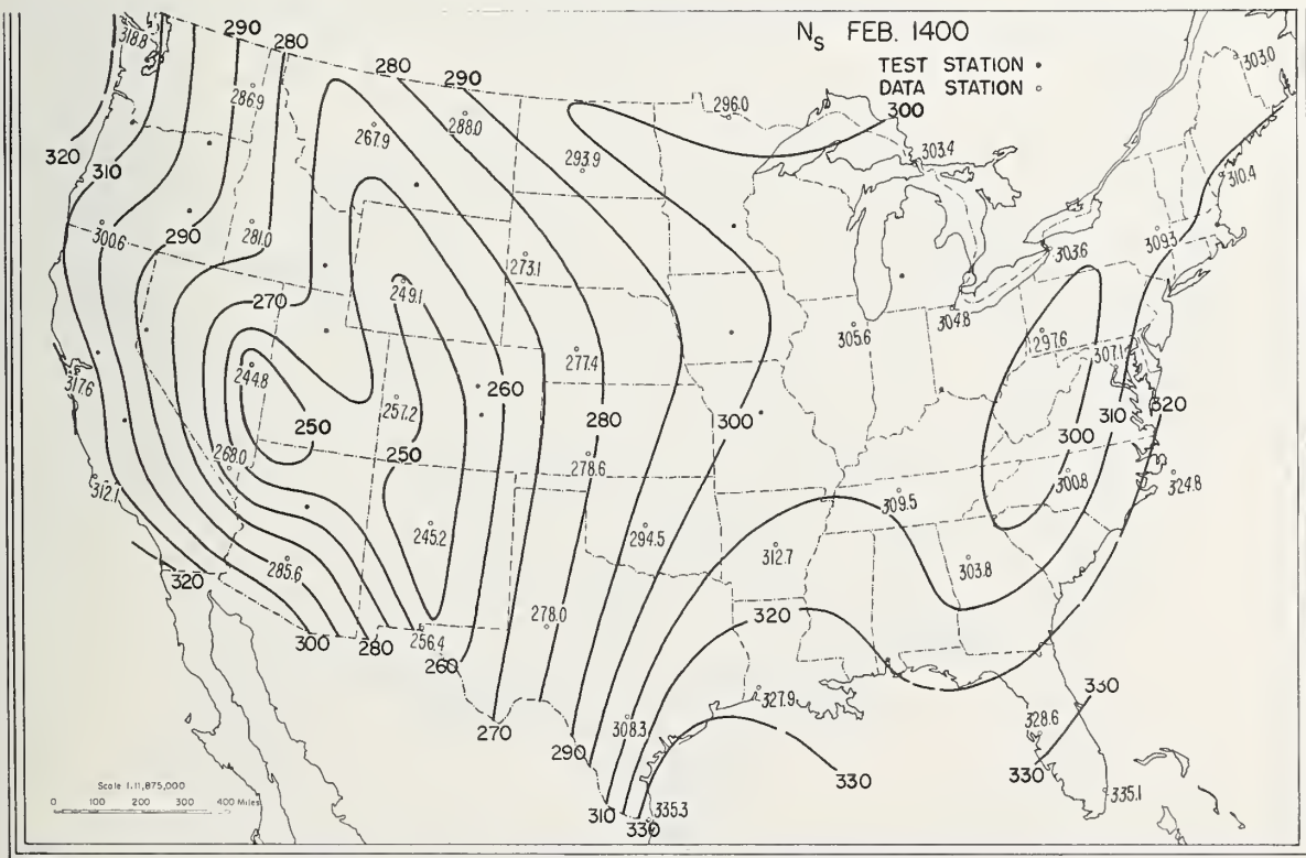
FIGURE 8. Mean N s : February 1400 (Test Map).
