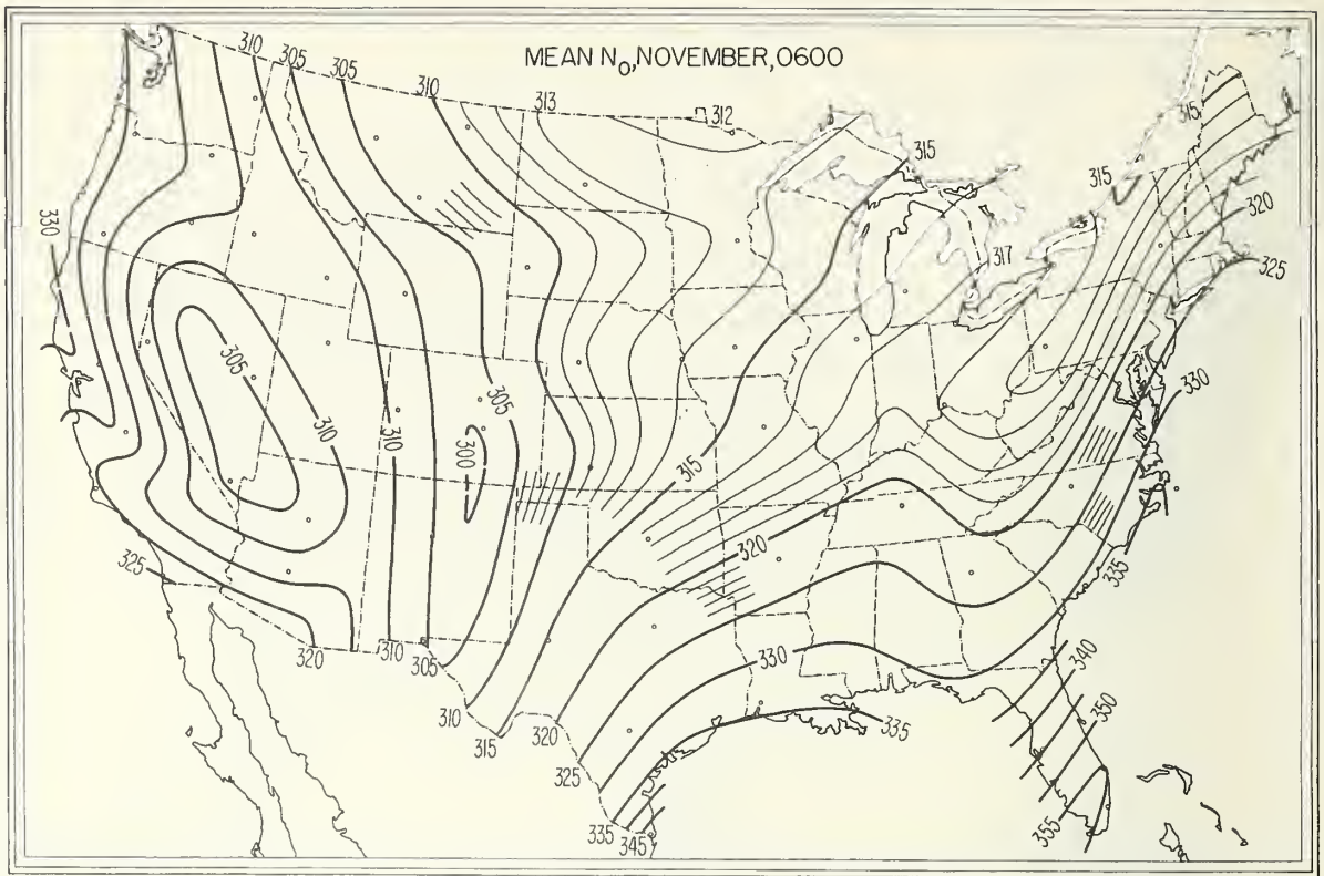
FIGURE 49. \bar{N}_o , November, 0600 local time.
