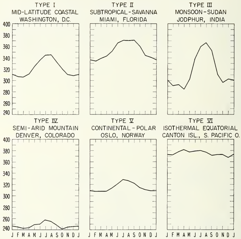
FIGURE 93. Annual cycles of N_2 by climatic types.
