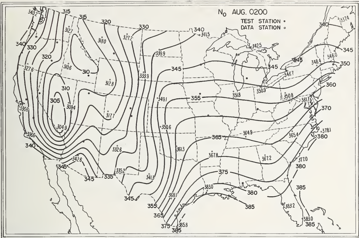
FIGURE 7. Mean N 0 : August 0200 (Test Map).
