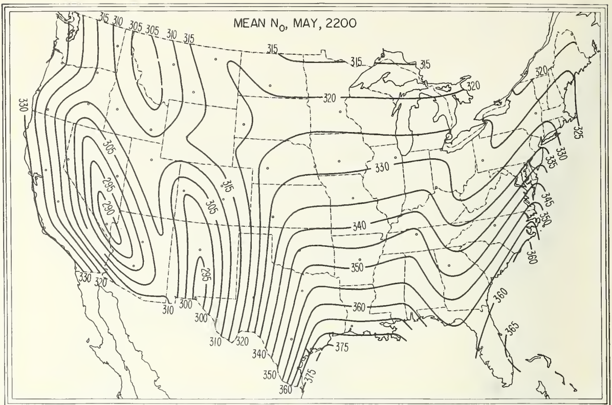
FIGURE 33. \bar{N}_o , May, 2200 local time.
