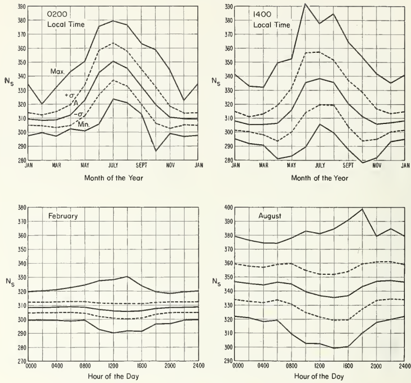
FIGURE 61. Annual and diurnal cycles of N_s : Joliet, Ill.
