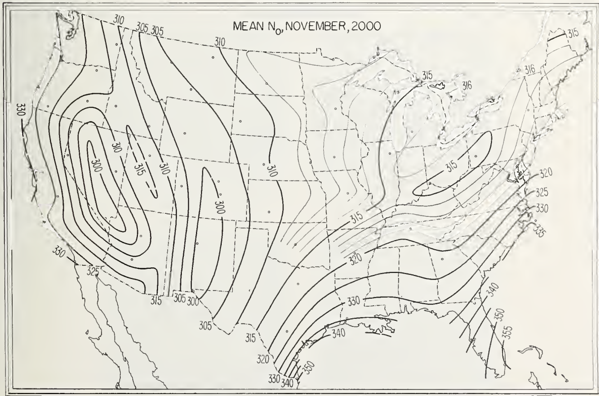
FIGURE 56. \bar{N}_p , November, 2000 local time.
