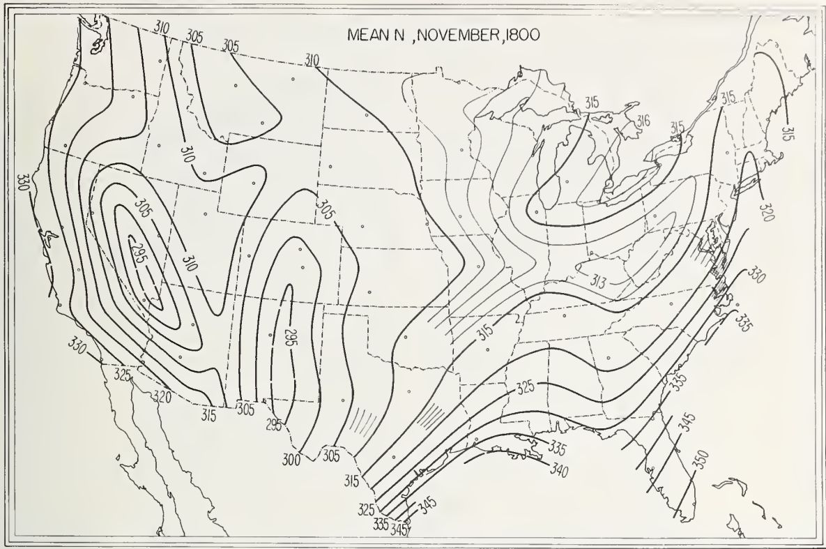
FIGURE 55. \bar{N}_p , November, 1800 local time.
