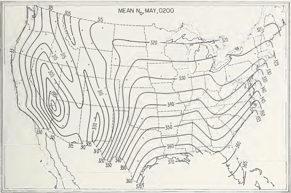
FIGURE 23. \bar{N}_o , May, 0200 local time.
