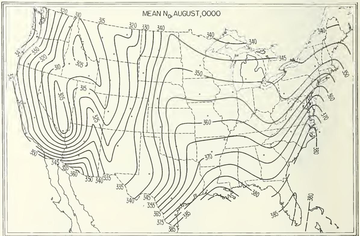
FIGURE 34. \bar{N}_o , August, 0000 local time.
