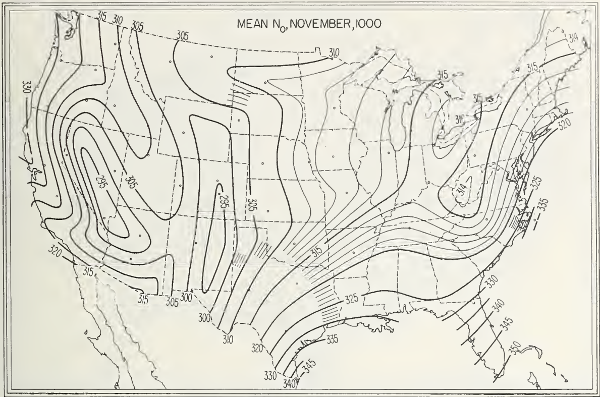
FIGURE 51. \bar{N}_o , November, 1000 local time.
