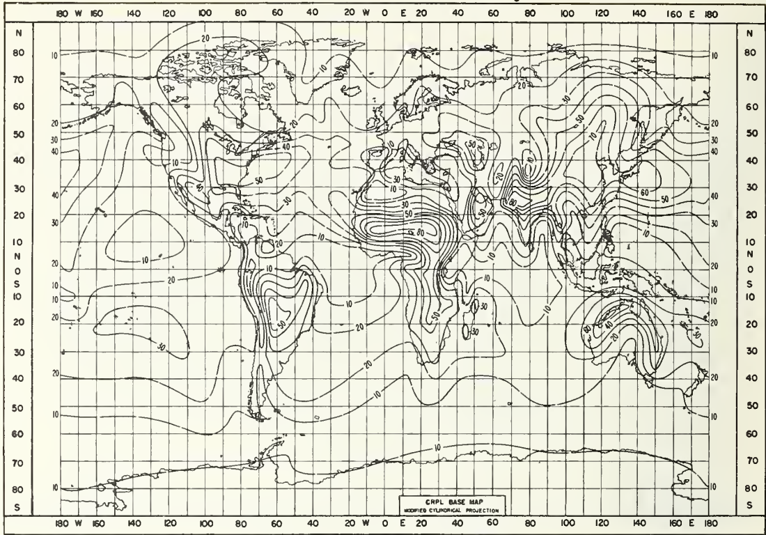
FIGURE 89. Annual range of \bar{N}_s .
