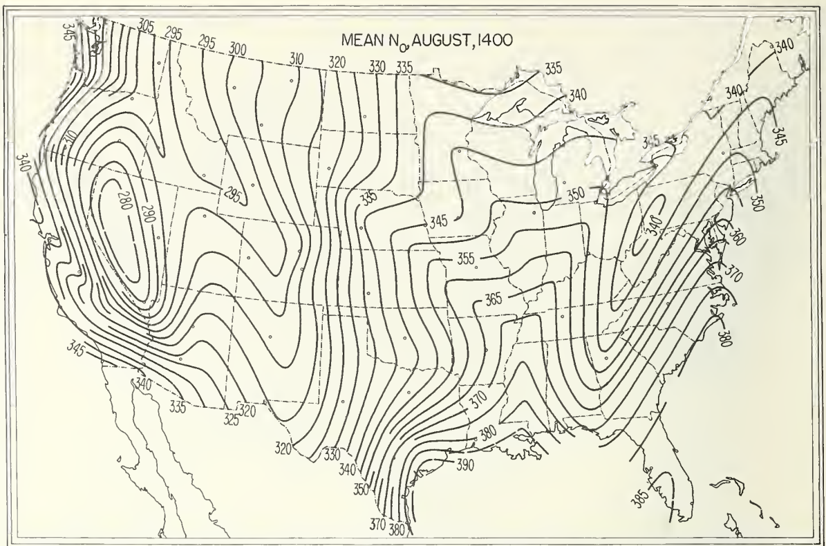
FIGURE 41. \bar{N}_o , August, 1400 local time.
