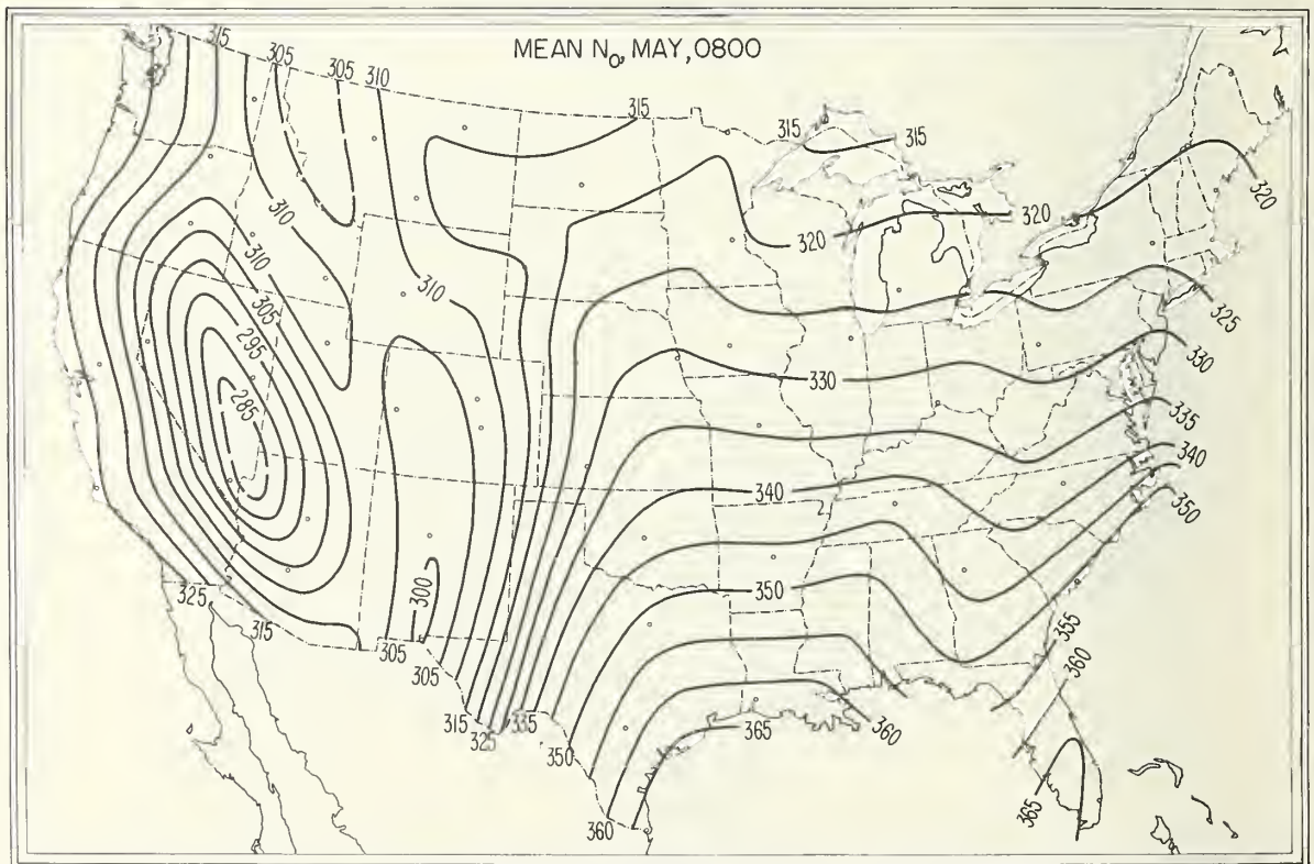
FIGURE 26. \bar{N}_o , May, 0800 local time.
