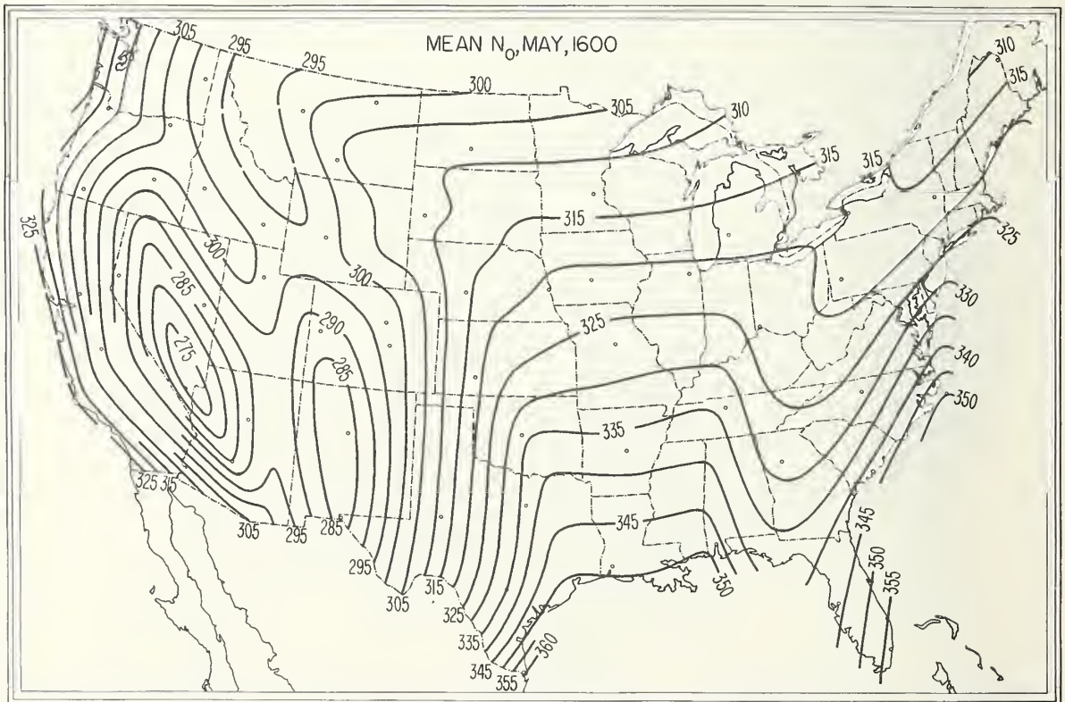
FIGURE 30. \bar{N}_p , May, 1600 local time.
