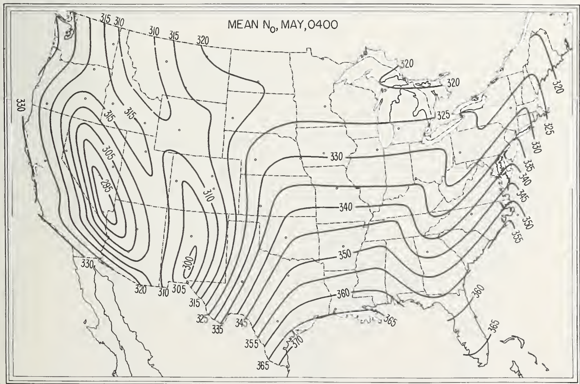
FIGURE 24. \bar{N}_o , May, 0400 local time.
