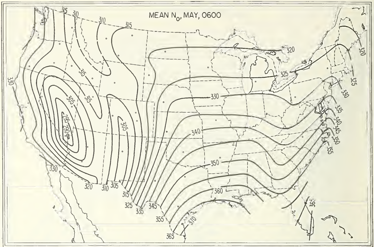
FIGURE 25. \bar{N}_o , May, 0600 local time.
