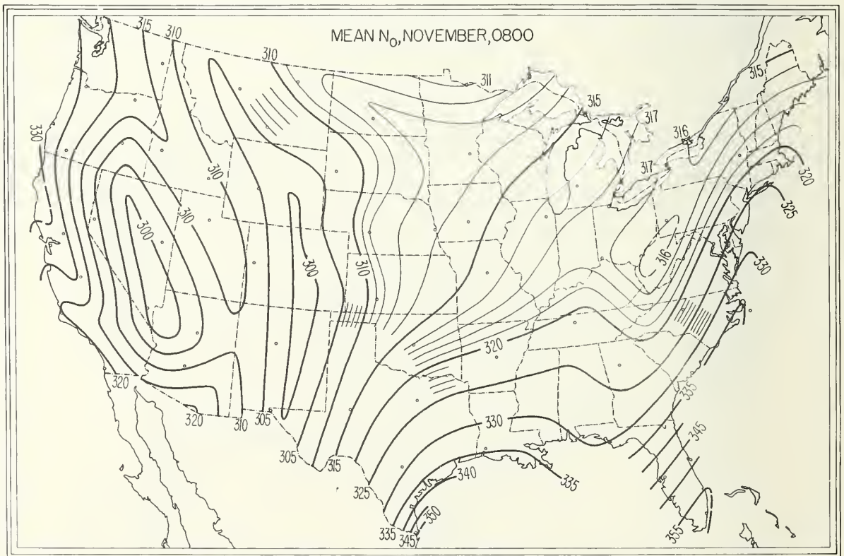
FIGURE 50. \bar{N}_o , November, 0800 local time.
