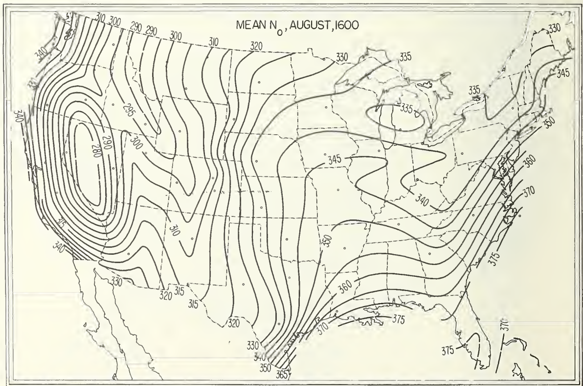
FIGURE 42. \bar{N}_o , August, 1600 local time.
