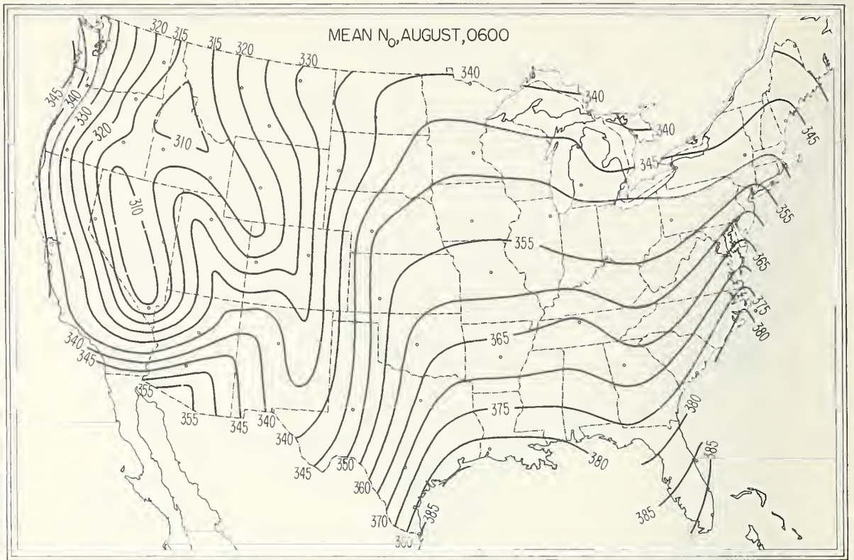
FIGURE 37. \bar{N}_o , August, 0600 local time.
