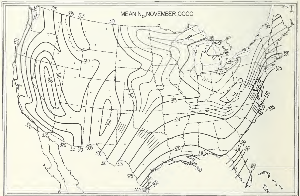
FIGURE 46. \bar{N}_o , November, 0000 local time.
