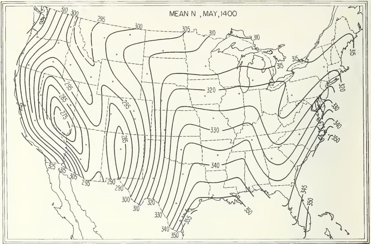
FIGURE 29. \bar{N}_p , May, 1400 local time.
