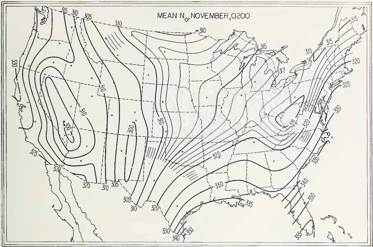
FIGURE 47. \bar{N}_o , November, 0200 local time.
