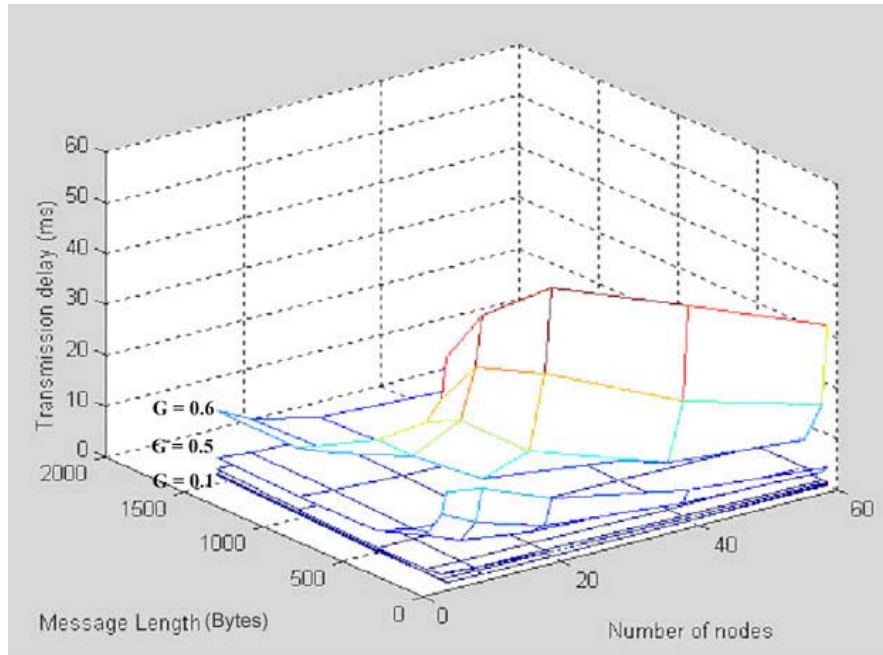
Figure 31. Transmission delay in Ethernet Networks.
