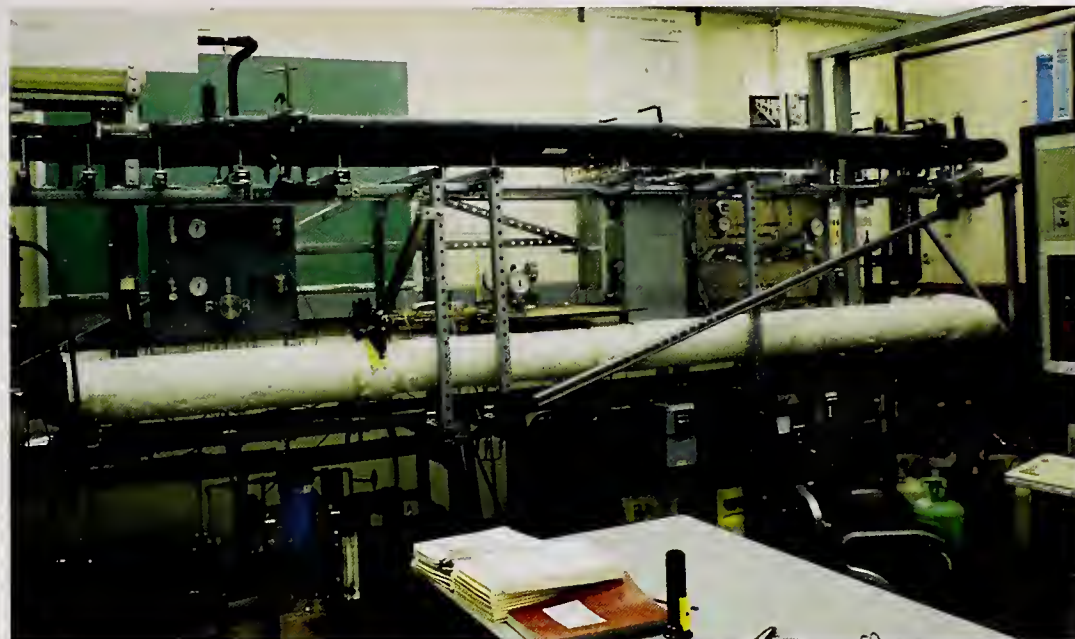
Instrumented and unique test rig measures the local convective condensation heat transfer coefficients of alternative refrigerants
