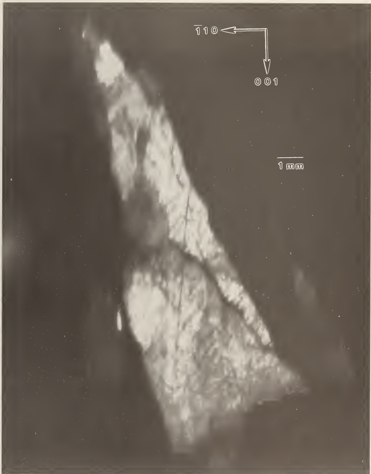
Figure 39. High-resolution (620) 8 keV diffraction image in Bragg geometry of approximately (220) surface of terrestrial PbSnTe crystal 108. The angle of incidence is 36 arc minutes smaller than that for figure 38; the growth direction is [001]. Lighter areas diffract more strongly.
