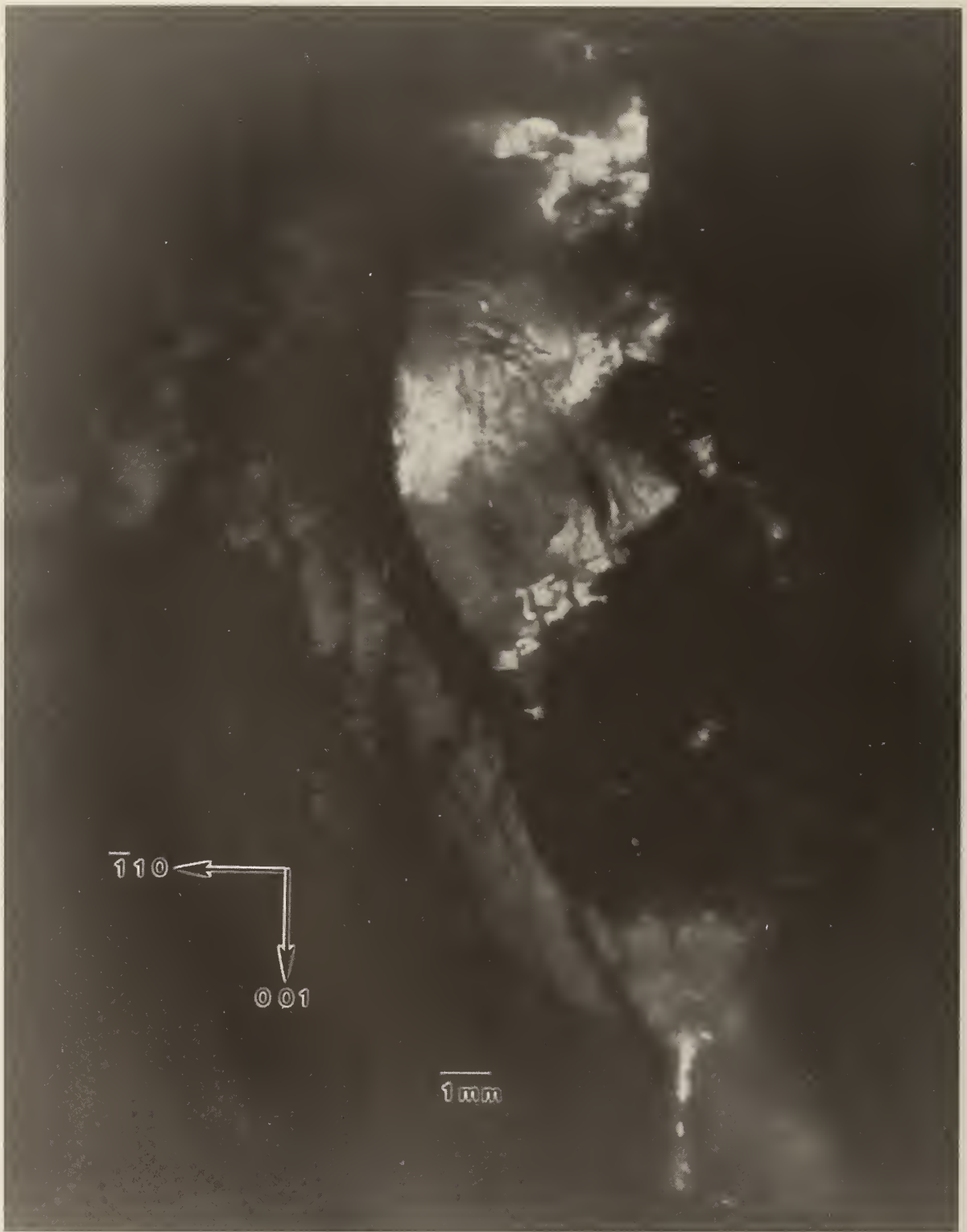
Figure 42. Second high-resolution (444) 8 keV diffraction image in Bragg geometry of approximately (220) surface of terrestrial PbSnTe crystal 108. The growth direction is [001]. Lighter areas diffract more strongly.
