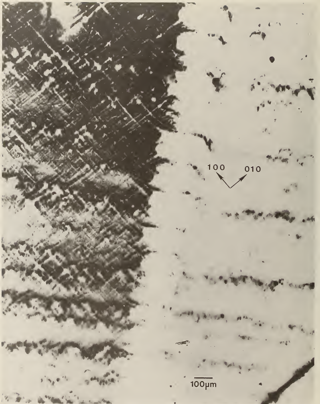
Figure 11. Enlargement of lower central portion of figure 2, (1 1 10) diffraction. This image is to be compared with the same crystal region imaged in (1 1 12) diffraction, figure 8. Darker areas diffract more strongly.
