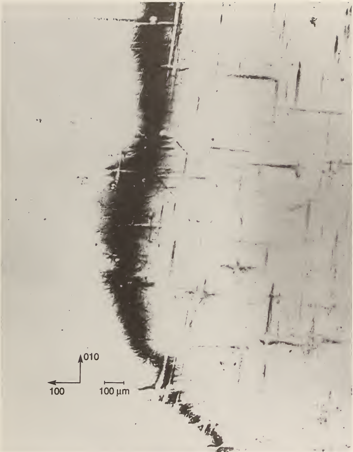
Figure 16. Enlargement of upper central portion of figure 3, (0 1 10) diffraction. The crystal region in this image is contiguous to the region imaged in (1 1 12) diffraction, figure 9, and in (1 1 10) diffraction, figure 12. Darker areas diffract more strongly.
