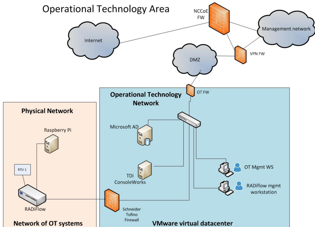
Figure 5-12 OT Network
