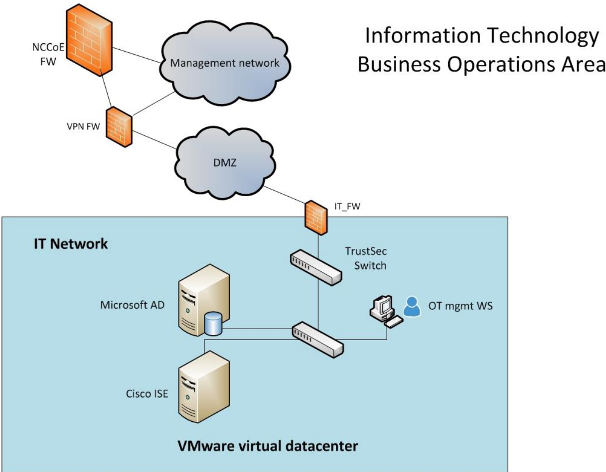
Figure 5-13 IT Network
