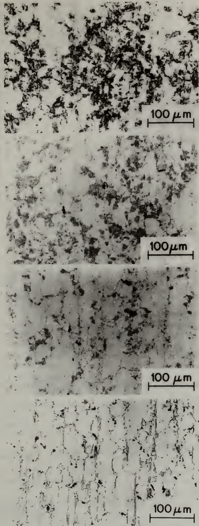
Fig. 61. Inconel 671 tested at 600 °C in oxidizing/sulfidizing/carburizing environment at 1 \times 10^{-6} /s. (Top to Bottom) Alpha-chromium phase present in alloy due to combined effects of temperature and strain. Progressing from maximum strain (fracture surface) to a smaller strain (near shoulder area of reduced section). 200 \times .
