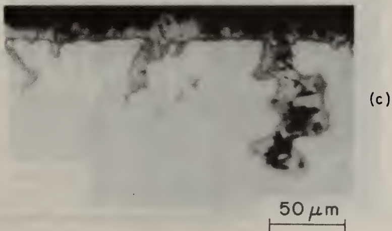
Fig. A-1. Type 310 specimen tested at 540 °C (1000 °F) at a strain rate of 10^{-6} /s in H 2 S plus steam. (a) SEM of specimen at region of fracture. (b) Photomicrograph of etched cross-section near fracture. (c) Photomicrograph of cracks in the unetched profile.
