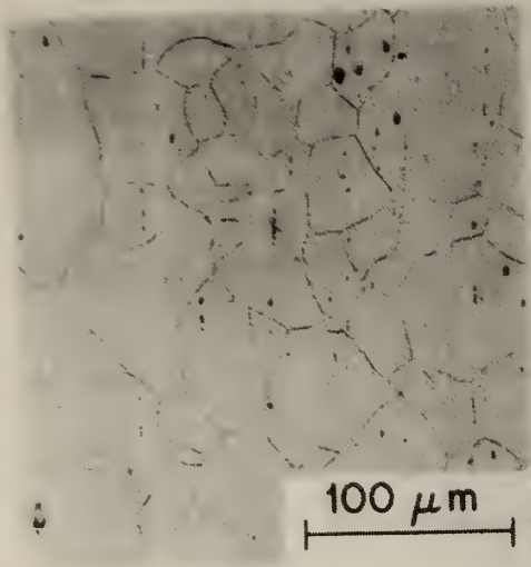
Type 309, 250 X
