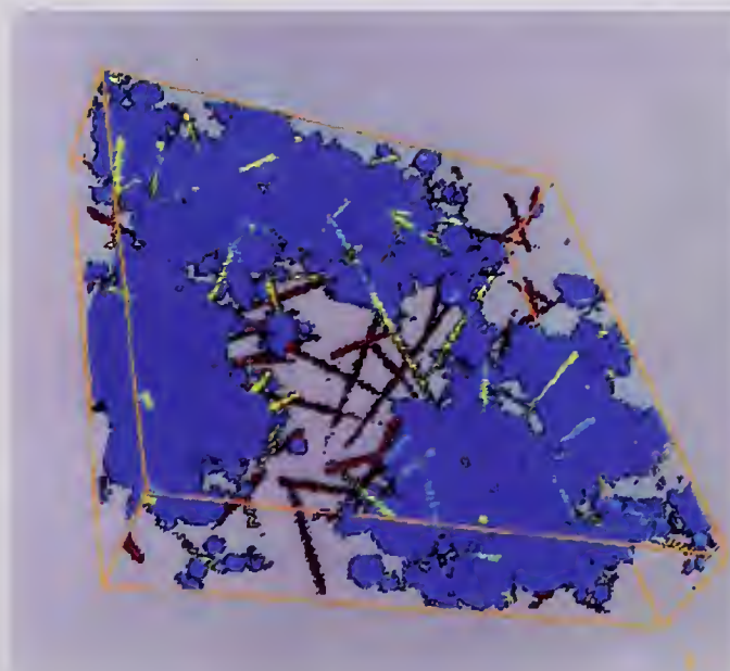
Illustration depicting the three-dimensional microstructure of a fiber-containing concrete. Aggregates with interconnected, percolated interfacial transition zone (ITZ) regions are blue. Fibers connecting these percolated aggregate clusters are yellow and remaining fibers are red.
