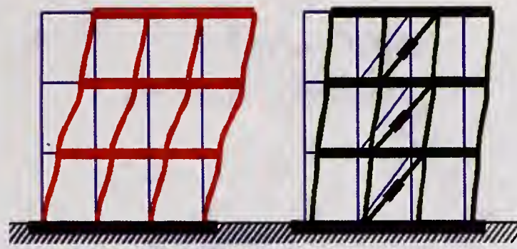
A computer simulation illustrates how structural dampers (right building) reduce inter-story drifts and minimize damage to the structure during strong earthquakes.
