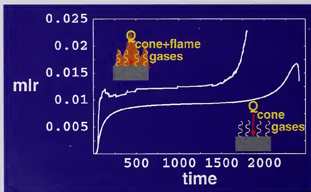
The Cone Calorimeter model is used to calculate the mass loss rate ( \text{kg}/\text{m}^2\text{s} ), or \text{mlr} , vs. \text{time}(\text{s}) for a burning polypropylene sample (upper plot). Radiative/convective feedback from the flame causes more rapid mass loss rate than for the pyrolyzing sample (lower plot) heated solely by incident radiation of 40 \text{ kW}/\text{m}^2 from the Cone heater.
