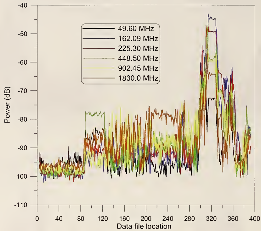
Figure 34. Signal strength measurements around the perimeter of the stadium for the transmitters located at fixed Site A and vertically polarized receiving antennas.
