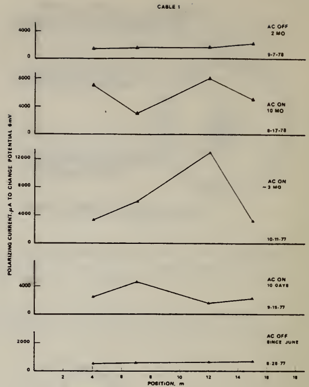
FIGURE 8 - The current required to polarize cable 1 6 mV at four positions and at different burial times.
