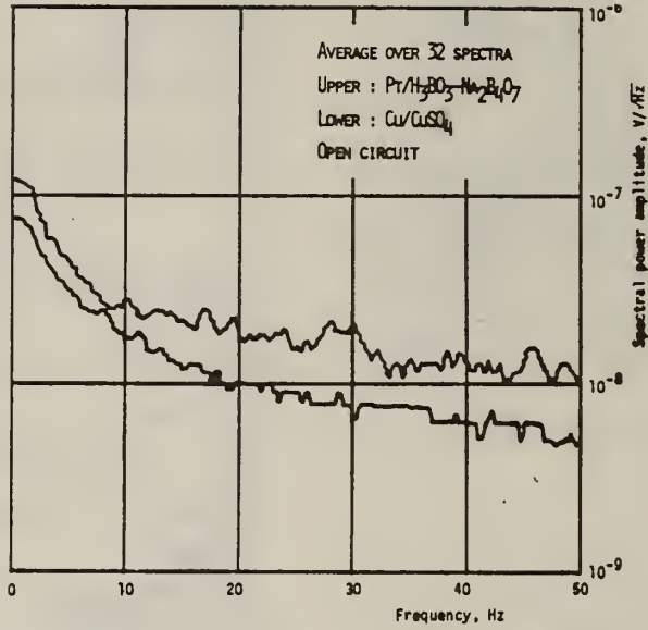
Fig. 20 Noise spectrum at open circuit. 1) Cu in CuSO_4 . 2) Pt in borate.
