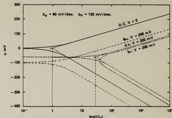
FIGURE 1 — Effect of a sinusoidal amplitude of 200 mV applied to an electrode with anodic Tafel slope ( b_a ) 60 mV/decade and cathodic slope ( b_c ) 120 mV/decade.
