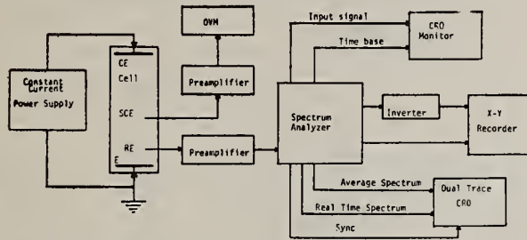
Fig. 2 Schematic circuit for noise measurements.
