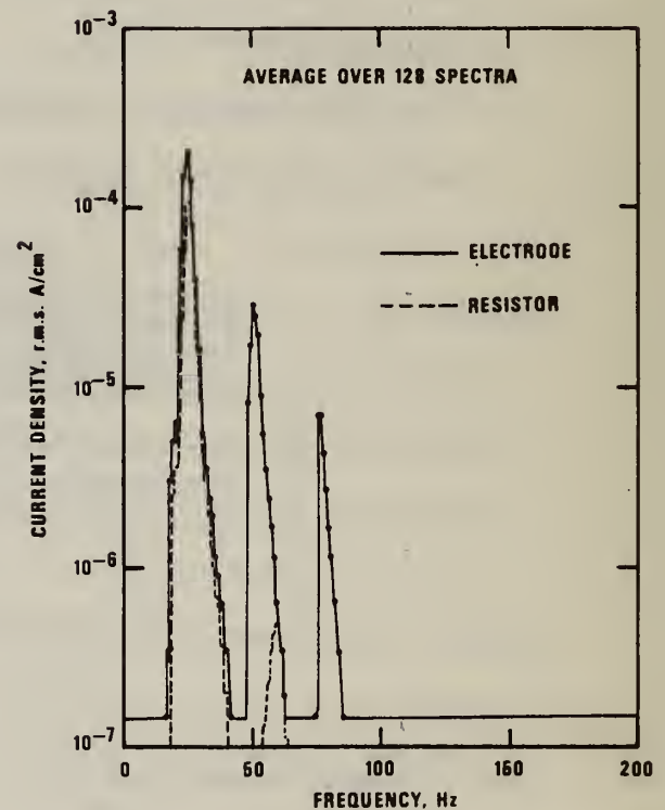
Fig. 5. Solid line: spectrum of current density for a Cu electrode in \text{H}_2\text{SO}_4 + \text{Na}_2\text{SO}_4 . E_0 = -506 mV vs. N.H.E., V = 50 mV, \nu = 25 Hz. Scale is log (r.m.s. \text{A}/\text{cm}^2 ) vs. Hz. Average over 128 spectra. Dotted line: spectrum of current through resistor. Scale is log (r.m.s. A) vs. Hz. Average over 128 spectra.
