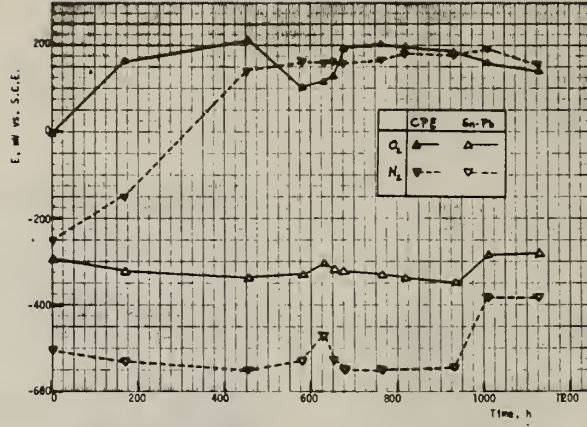
Fig. 19 Rest potential vs. time for CPE and Pb-Sn alloy in 2% Na_2SO_4 + 1% NaCl.
