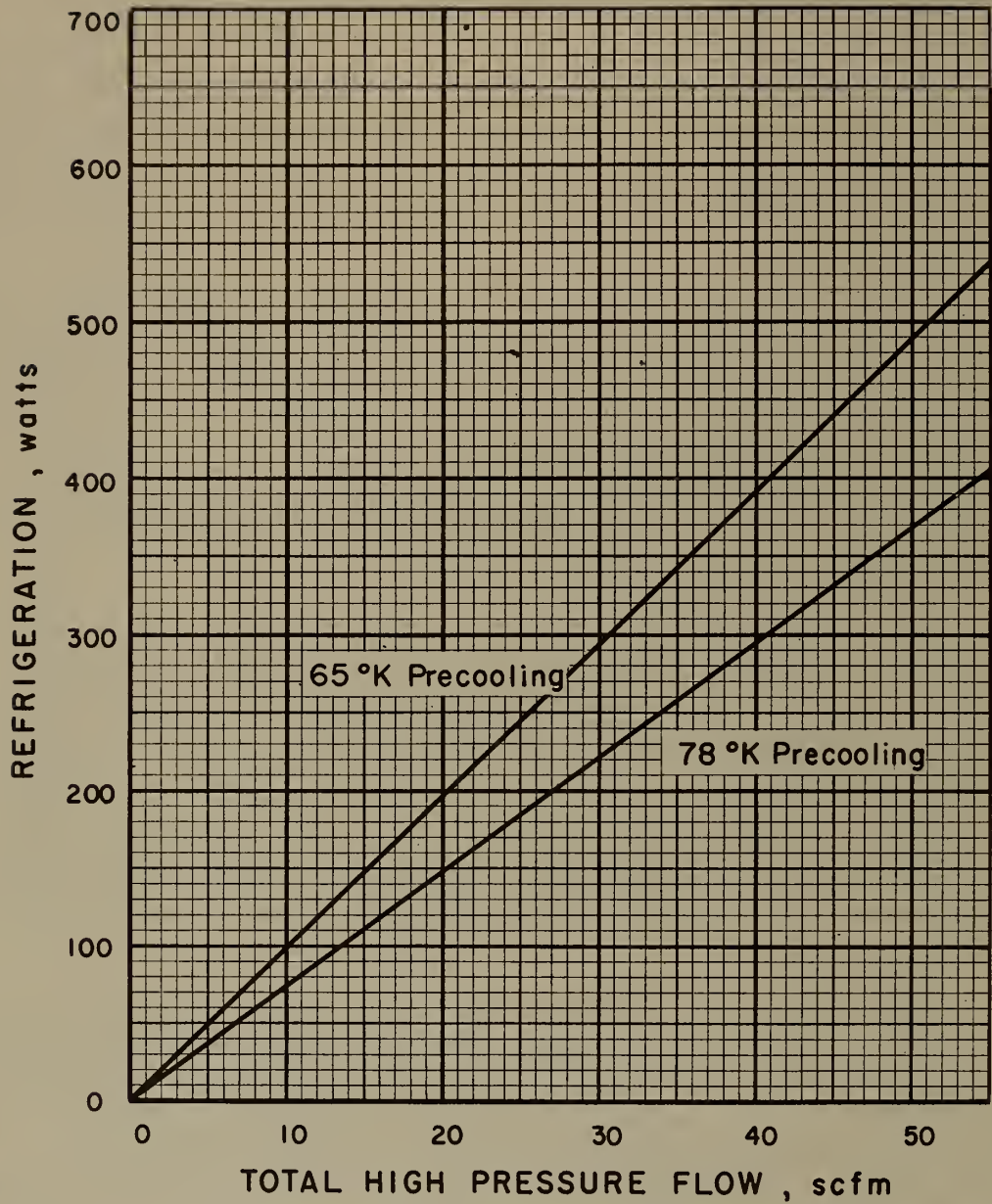
Figure 9. Theoretical Refrigeration
