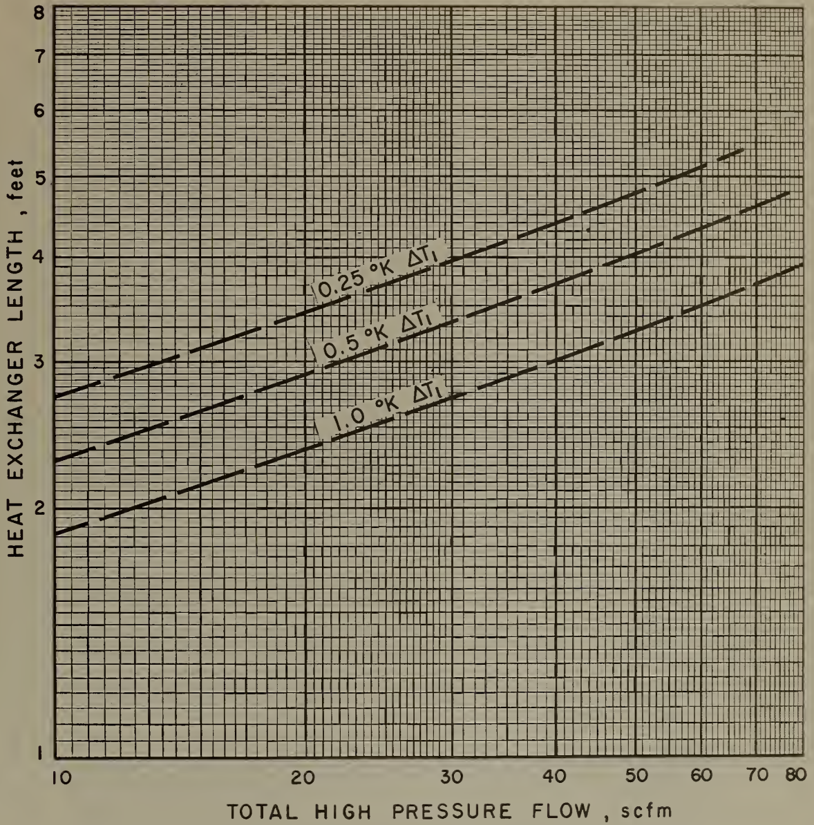
Figure 17. Final Heat Exchanger Length for 78^\circ\text{K} Precooled Refrigerator
