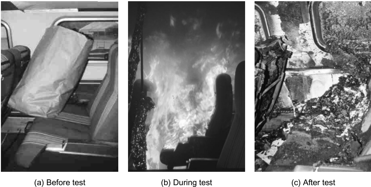
Figure 28. Amfleet I Test Car - Seating Area with Trash Bag Ignition
