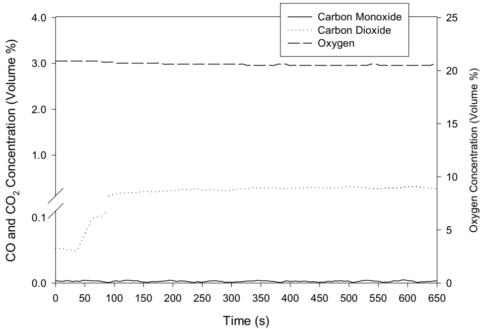
Figure B-129. Test 16 (Seat with TB 133 Burner), Gas Concentration Data
