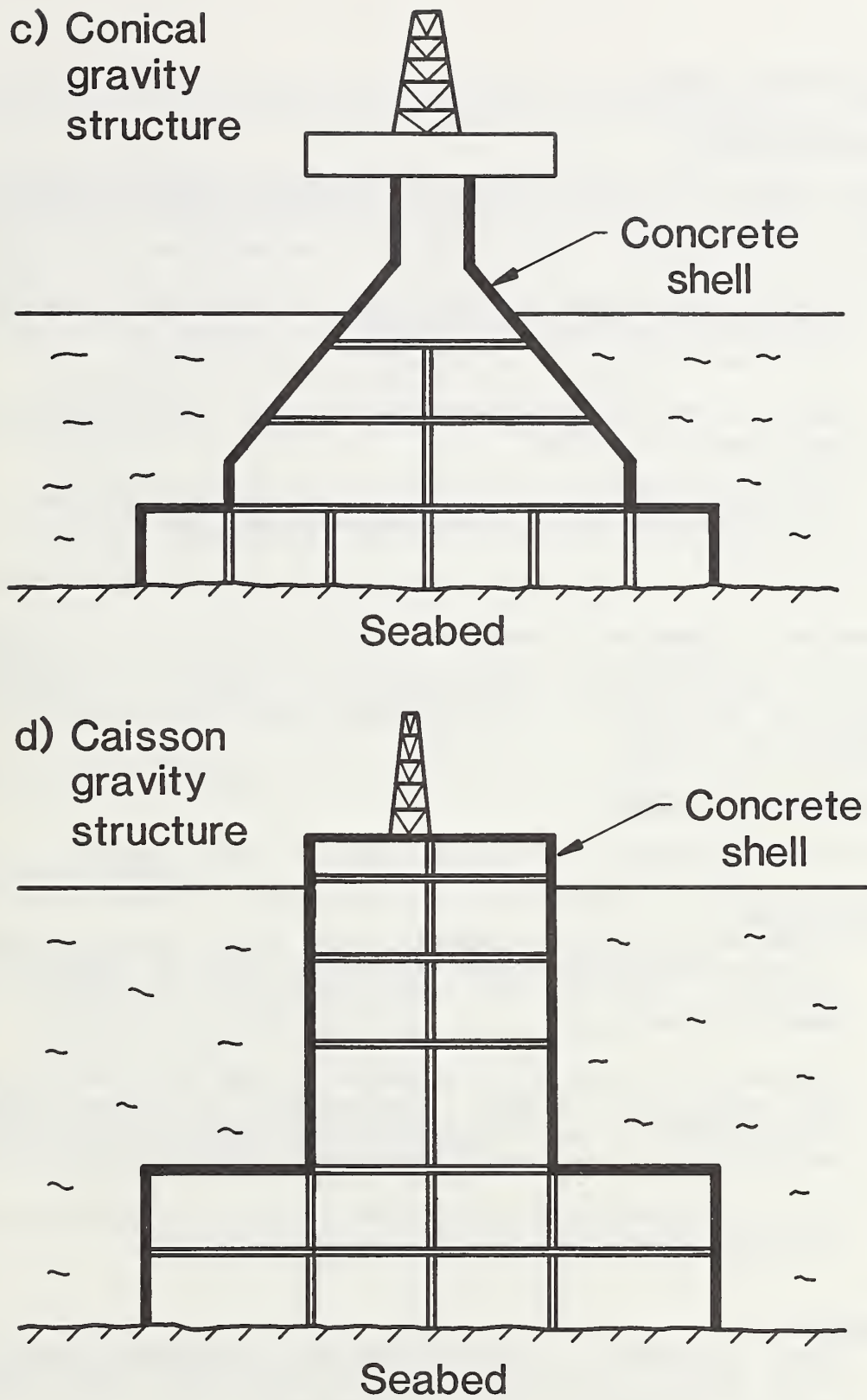
Figure 1 Generic types of offshore structures proposed for the Arctic
