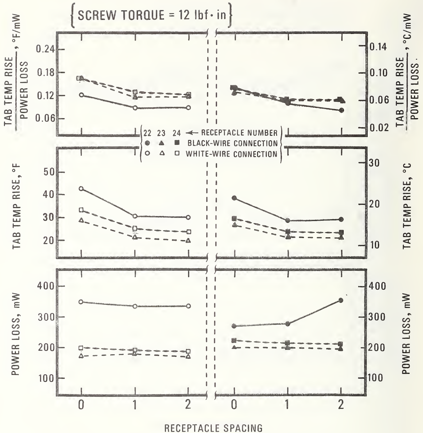
Figure 31. Values of the power loss, the tab temperature rise, and the ratio of the tab temperature rise to the power loss plotted as a function of the receptacle spacing for the black-wire and white-wire connections of conventional receptacles No. 22, 23, and 24. The terminal screws of the receptacles were tightened with a torque of 12 lbf·in. The values plotted are averages of values determined in tests employing a test voltage of 10 V(ac). The range of the values was less than the symbol heights, which are equivalent to about 15 mW, 2 °F, and 0.012 °F/mW for the power loss, the temperature rise, and the ratio, respectively.
