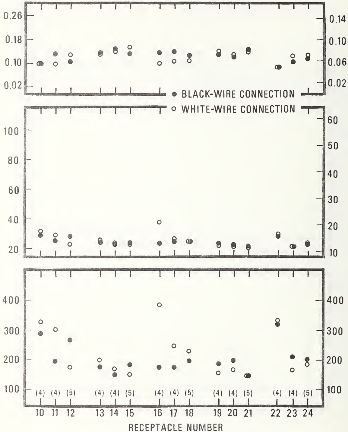
Figure 7. Values of the power loss, the tab temperature rise, and the ratio of the tab temperature rise to the power loss obtained for the black-wire and white-wire connections of the conventional receptacles during group receptacle tests: receptacles spaced two outlet boxes apart, terminal screws tightened with a torque of 16 lbf·in. The values plotted are averages of values determined in tests employing test voltages of 10 V(ac) and 115 V(ac). The figures in parentheses indicate the number of tests used in computing the averages. The range of the values was less than the symbol heights, which are equivalent to about 15 mW, 3 °F, and 0.015 °F/mW for the power loss, the temperature rise, and the ratio, respectively.
