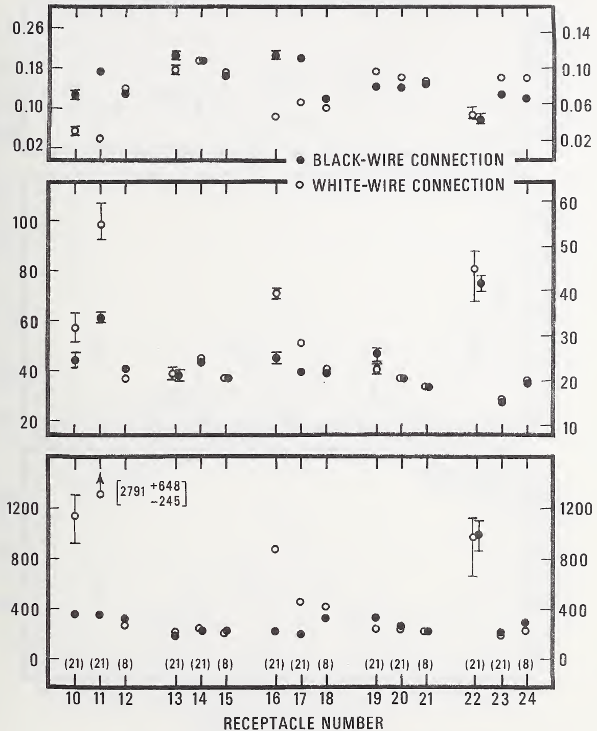
Figure 14. Values of the power loss, the tab temperature rise, and the ratio of the tab temperature rise to the power loss obtained for the black-wire and white-wire connections of the conventional receptacles during group receptacle tests: receptacles installed in adjacent outlet boxes, terminal screws tightened with a torque of 2 lbf·in. The values plotted are averages of values determined in tests employing test voltages of 10 V(dc), 10 V(ac), and 115 V(ac). The figures in parentheses indicate the number of tests used in computing the averages. The bars give the range of the values. The symbol heights are equivalent to about 60 mW, 3 °F, and 0.015 °F/mW for the power loss, the temperature rise, and the ratio, respectively.
