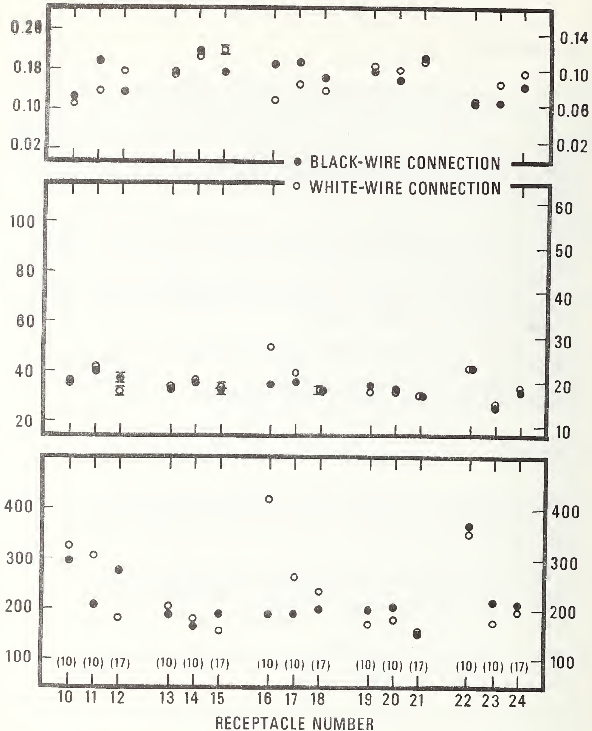
Figure 5. Values of the power loss, the tab temperature rise, and the ratio of the tab temperature rise to the power loss obtained for the black-wire and white-wire connections of the conventional receptacles during group receptacle tests: receptacles installed in adjacent outlet boxes, terminal screws tightened with a torque of 16 lbf·in. The values plotted are averages of values determined in tests employing test voltages of 10 V(dc), 10 V(ac), and 115 V(ac). The figures in parentheses indicate the number of tests used in computing the averages. The bars give the range of the values. The symbol heights are equivalent to about 15 mW, 3 °F, and 0.015 °F/mW for the power loss, the temperature rise, and the ratio, respectively.
