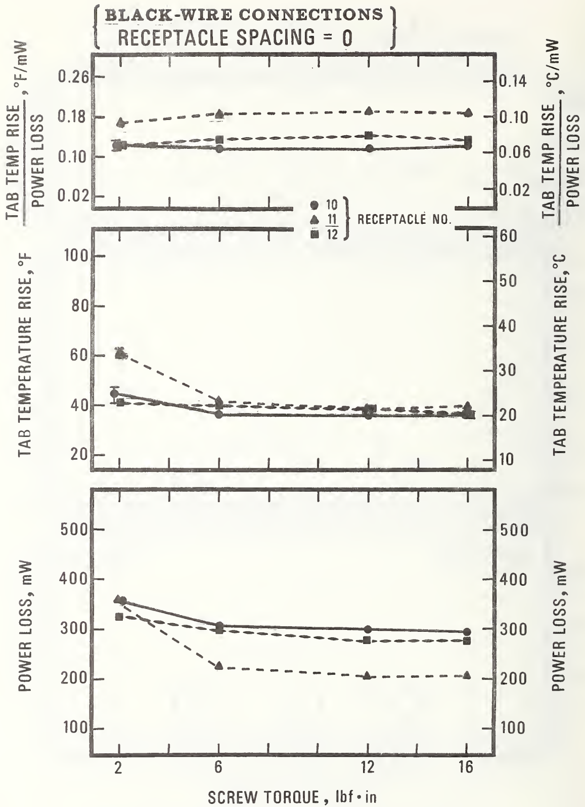
Figure 17. Values of the power loss, the tab temperature rise, and the ratio of the tab temperature rise to the power loss plotted as a function of the terminal screw torque for the black-wire connections of conventional receptacles No. 10, 11, and 12. The receptacles were installed in adjacent outlet boxes. The values plotted are averages of values determined in tests employing test voltages of 10 V(dc), 10 V(ac), and 115 V(ac). The bars give the range of the values.
