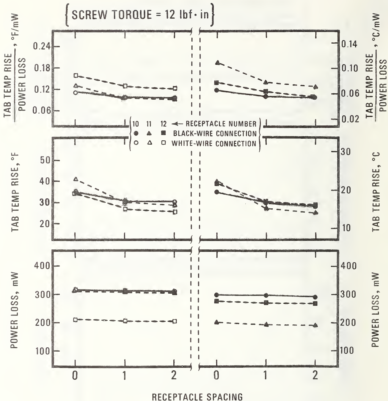
Figure 27. Values of the power loss, the tab temperature rise, and the ratio of the tab temperature rise to the power loss plotted as a function of the receptacle spacing for the black-wire and white-wire connections of conventional receptacles No. 10, 11, and 12. The terminal screws of the receptacles were tightened with a torque of 12 lbf·in. The values plotted are averages of values determined in tests employing a test voltage of 10 V(ac). The range of the values was less than the symbol height, which are equivalent to about 15 mW, 2 °F, and 0.012 °F/mW for the power loss, the temperature rise, and the ratio, respectively.
