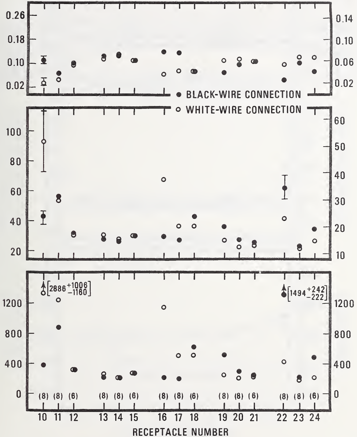
Figure 16. Values of the power loss, the tab temperature rise, and the ratio of the tab temperature rise to the power loss obtained for the black-wire and white-wire connections of the conventional receptacles during group receptacle tests: receptacles spaced two outlet boxes apart, terminal screws tightened with a torque of 2 lbf·in. The values plotted are averages of values determined in tests employing test voltages of 10 V(ac) and 115 V(ac). The figures in parentheses indicate the number of tests used in computing the averages. The bars give the range of the values. The symbol heights are equivalent to about 60 mW, 3 °F, and 0.015 °F/mW for the power loss, the temperature rise, and the ratio, respectively.
