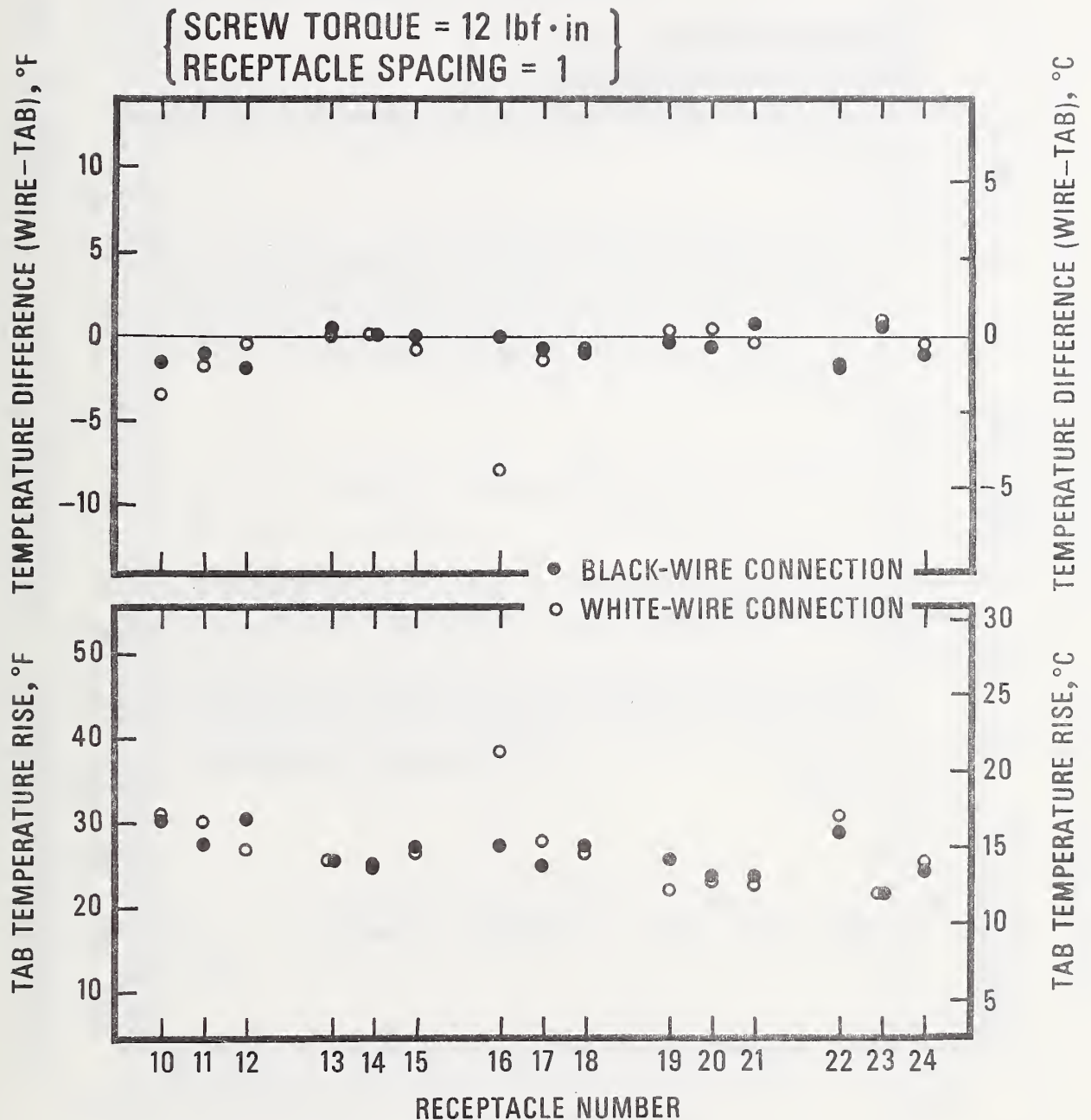
Figure 32. The tab temperature rise and the difference between the wire temperature and the tab temperature for the black-wire and white-wire connections of the conventional receptacles: receptacles spaced one outlet box apart, terminal screws tightened with a torque of 12·lbf in. The difference was calculated from the averages of values determined during three consecutive tests in which the test voltage was 10 V(ac). The 99% confidence limits for the difference between the averages are less than the symbol heights, which are equivalent to about 0.8 °F for the difference and about 1.5 °F for the tab temperature rise.
