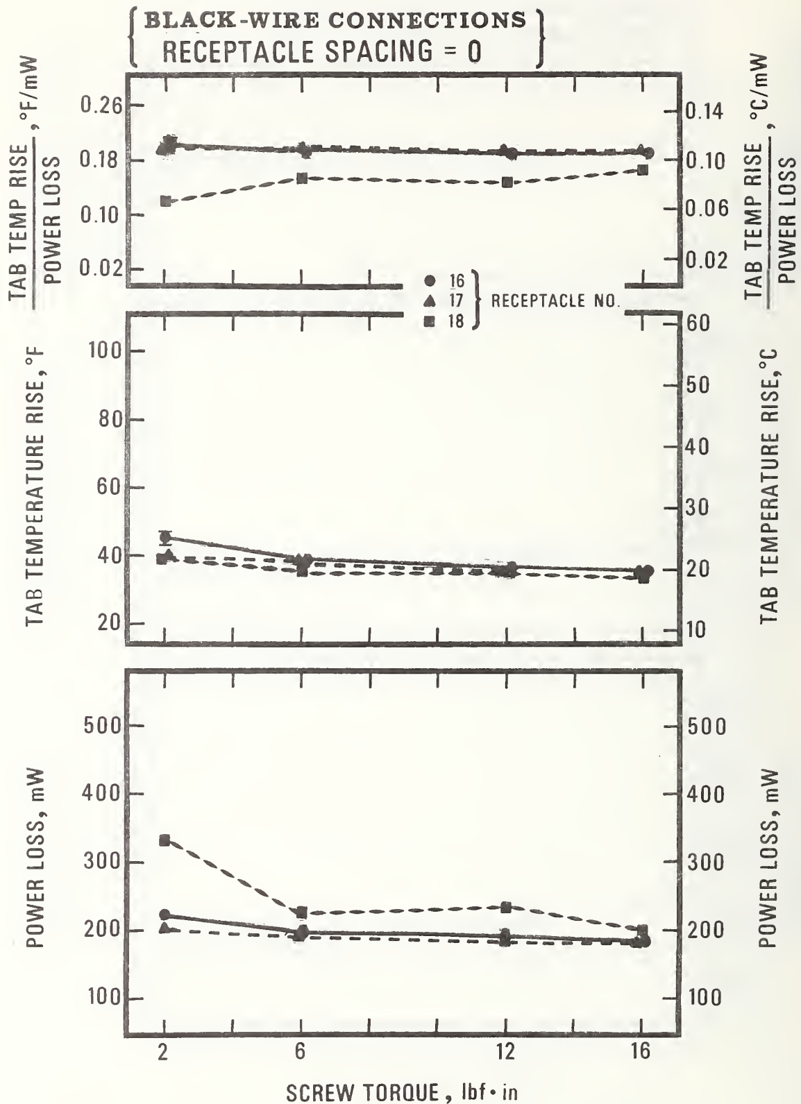
Figure 21. Values of the power, the tab temperature rise, and the ratio of the tab temperature rise to the power loss plotted as a function of the terminal screw torque for the black-wire connections of conventional receptacles No. 16, 17, and 18. The receptacles were installed in adjacent outlet boxes. The values plotted are averages of values determined in tests employing test voltages of 10 V(dc), 10 V(ac), and 115 V(ac). The bars give the range of the values.
