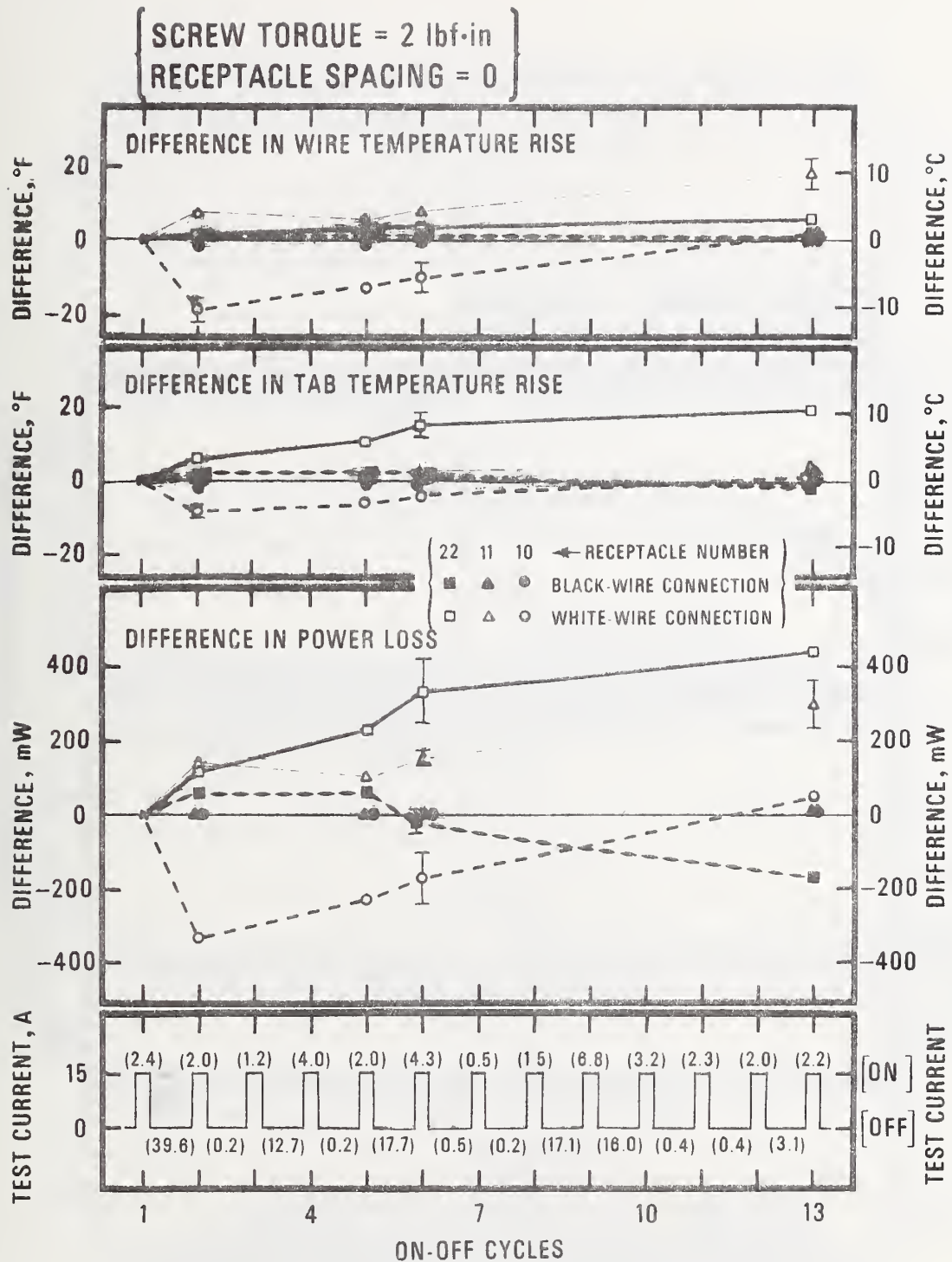
Figure 36. Change in the power loss, the tab temperature rise, and the wire temperature rise for the black-wire and white-wire connections of conventional receptacles No. 10, 11, and 22 as a function of the number of on-off cycles of the test current. The receptacles were installed in adjacent outlet boxes and their terminal screws were tightened with a torque of 2 lbf·in. The test voltage was 115 V(ac) for the values plotted. Difference equals average value during indicated cycle minus average value during first cycle. The bars give the 95% confidence limits for the difference. The figures in parentheses give the time, in hours, that the test current was on and off during each cycle.
