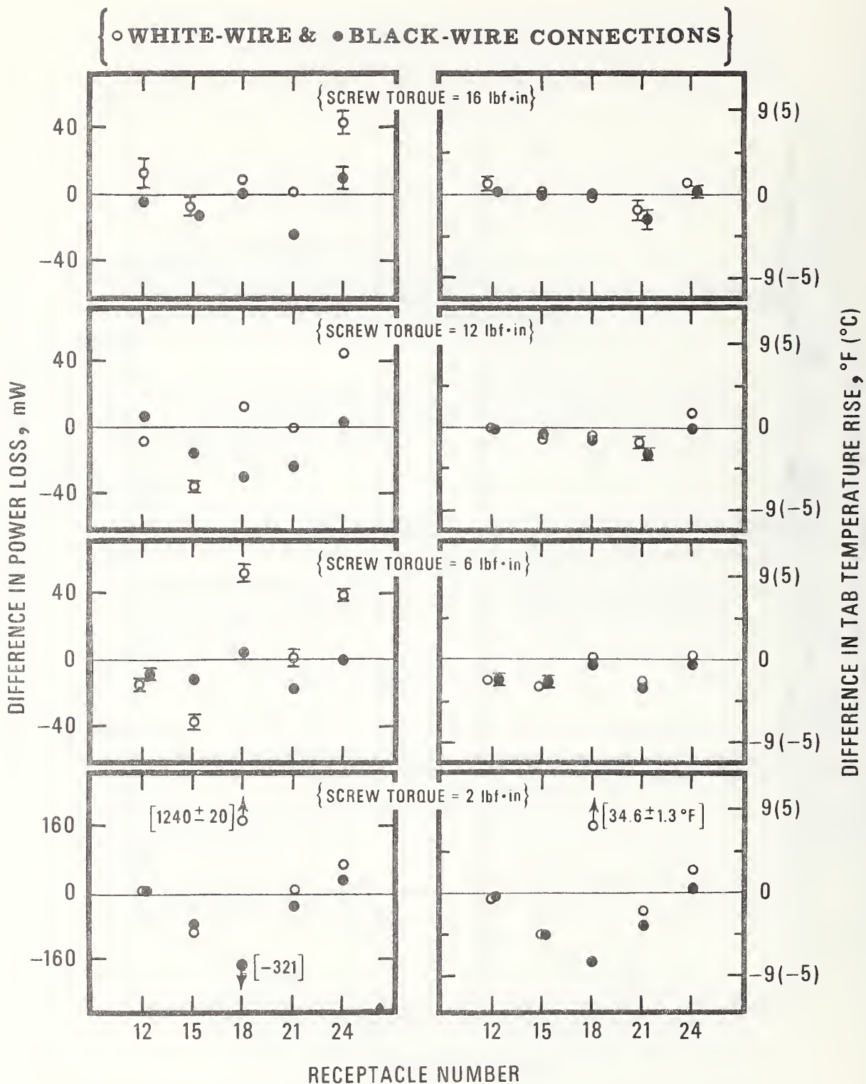
Figure 39. Difference between the values of power loss and tab temperature rise obtained in individual receptacle tests and those obtained in group receptacle tests conducted with the receptacles spaced two outlet boxes apart. Difference equals average of values obtained in individual receptacle tests using a test voltage of 115 V(ac) minus average of values obtained in group receptacle tests using a test voltage of 115 V(ac). Bars give the 95% confidence limits for the difference between the averages.
