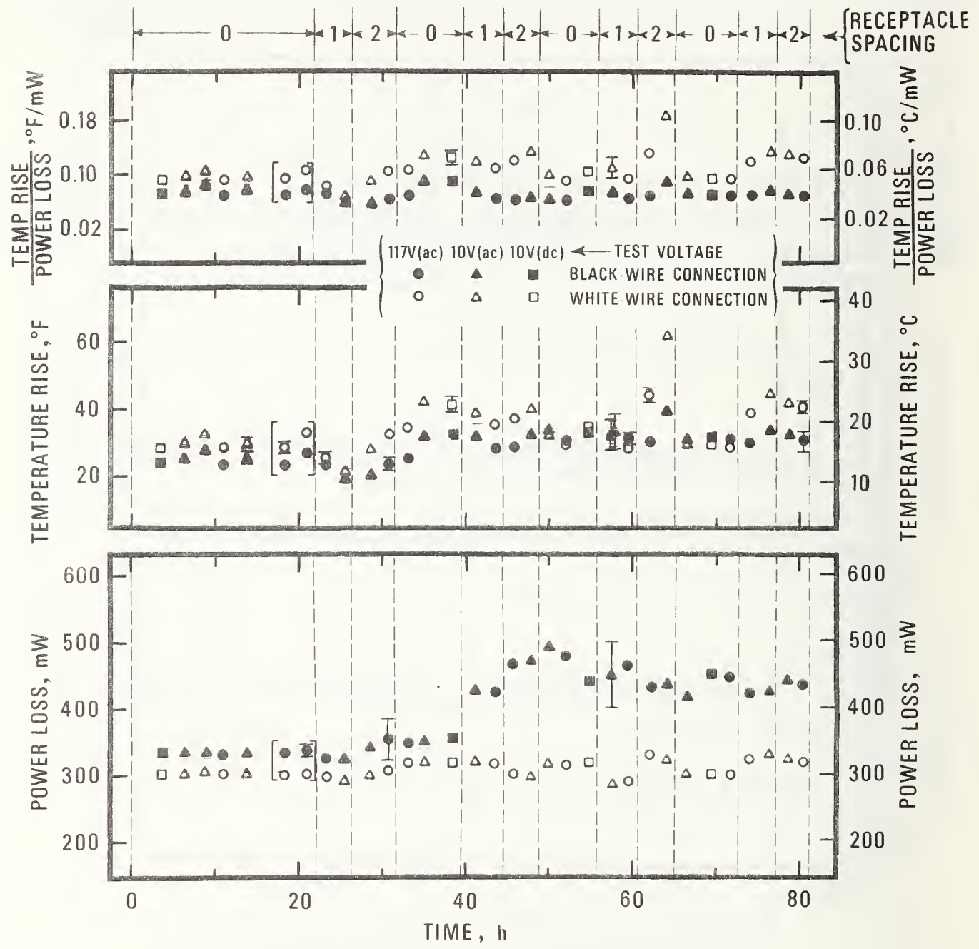
Figure 41. Values of the power loss, the temperature rise, and the ratio of the temperature rise to the power loss for the black-wire and white-wire connections of split-beam receptacle No. 8 plotted as a function of the time that test circuit was energized. Each of the data points represents the average of values obtained in several (2 to 4) tests. The bars give the 95% confidence limits for the averages. The symbol heights are equivalent to about 15 mW, 3 °F, and 0.015 °F/mW for the power loss, the temperature rise, and the ratio, respectively.
