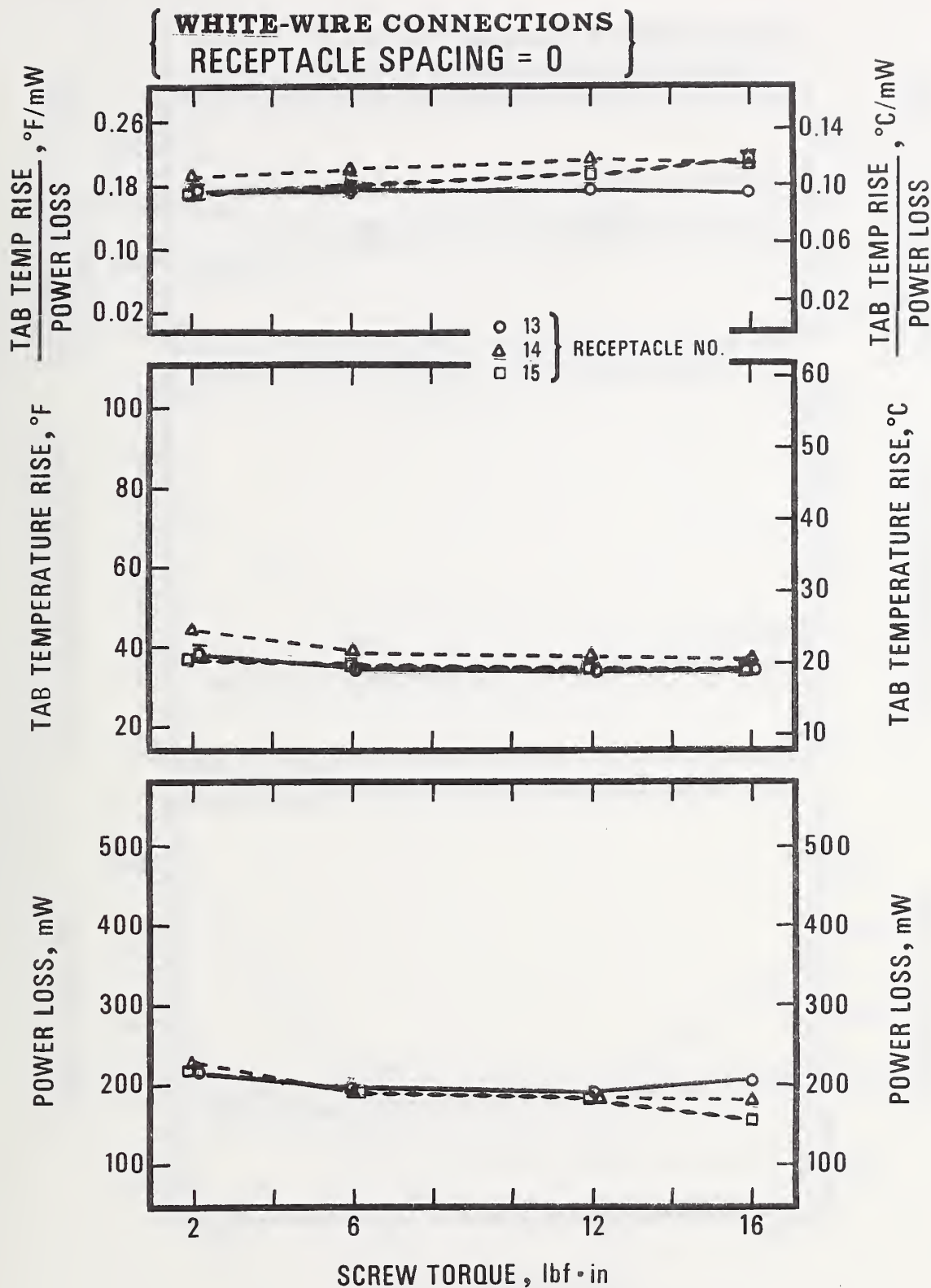
Figure 20. Values of the power loss, the tab temperature rise, and the ratio of the tab temperature rise to the power loss plotted as a function of the terminal screw torque for the white-wire connections of conventional receptacles No. 13, 14, and 15. The receptacles were installed in adjacent outlet boxes. The values plotted are averages of values determined in tests employing test voltages of 10 V(dc), 10 V(ac), and 115 V(ac). The bars give the range of the values.
