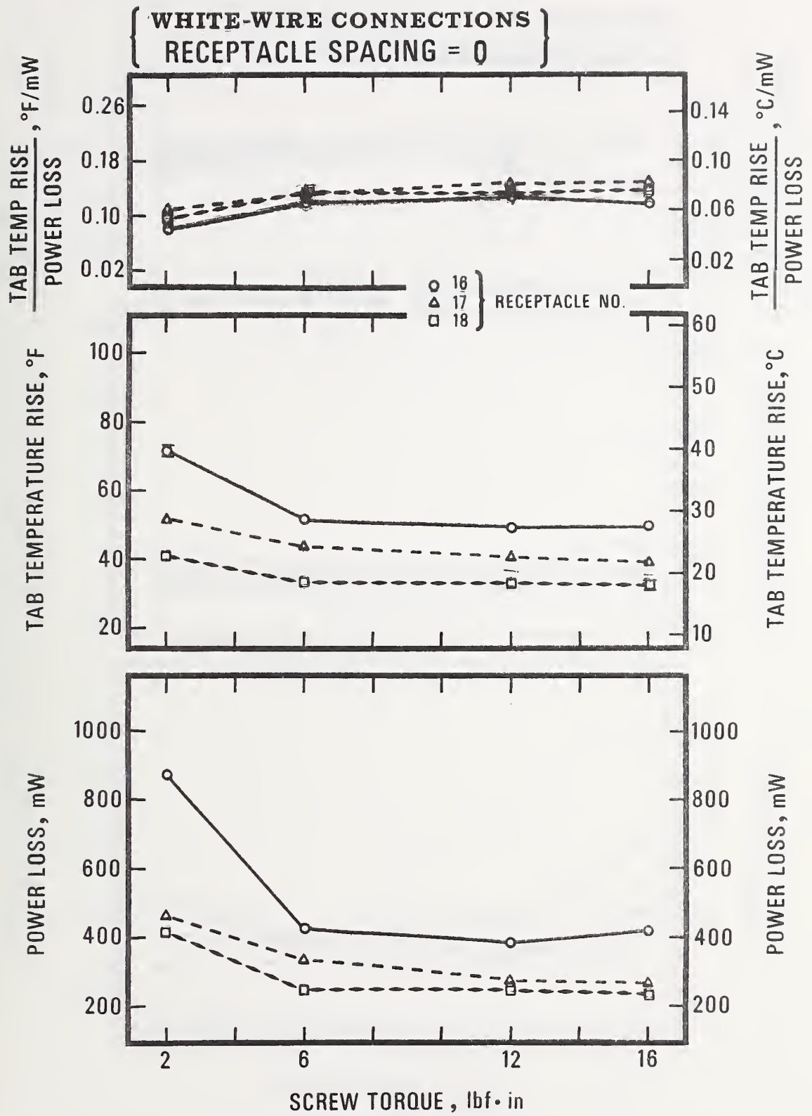
Figure 22. Values of the power loss, the tab temperature rise, and the ratio of the tab temperature rise to the power loss plotted as a function of the terminal screw torque for the white-wire connections of conventional receptacles No. 16, 17, and 18. The receptacles were installed in adjacent outlet boxes. The values plotted are averages of values determined in tests employing test voltages of 10 V(dc), 10 V(ac), and 115 V(ac). The bars give the range of the values.
