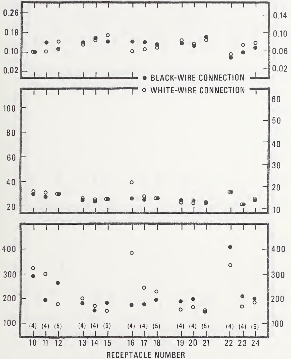
Figure 6. Values of the power loss, the tab temperature rise, and the ratio of the tab temperature rise to the power loss obtained for the black-wire and white-wire connections of the conventional receptacles during group receptacle tests: receptacles spaced one outlet box apart, terminal screws tightened with a torque of 16 lbf · in. The values plotted are averages of values determined in tests employing test voltages of 10 V(ac) and 115 V(ac). The figures in parentheses indicate the number of tests used in computing the averages. The range of the values was less than the symbol heights, which are equivalent to about 15 mW, 3 °F, and 0.015 °F/mW for the power loss, the temperature rise, and the ratio, respectively.
