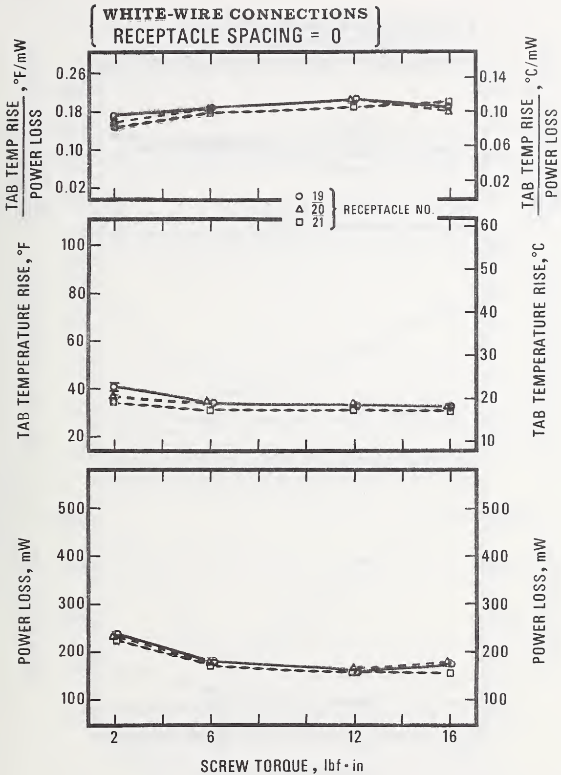
Figure 24. Values of the power loss, the tab temperature rise, and the ratio of the tab temperature rise to the power loss plotted as a function of the terminal screw torque for the white-wire connections of conventional receptacles No. 19, 20, and 21. The receptacles were installed in adjacent outlet boxes. The values plotted are averages of values determined in tests employing test voltages of 10 V(dc), 10 V(ac), and 115 V(ac). The bars give the range of the values.
