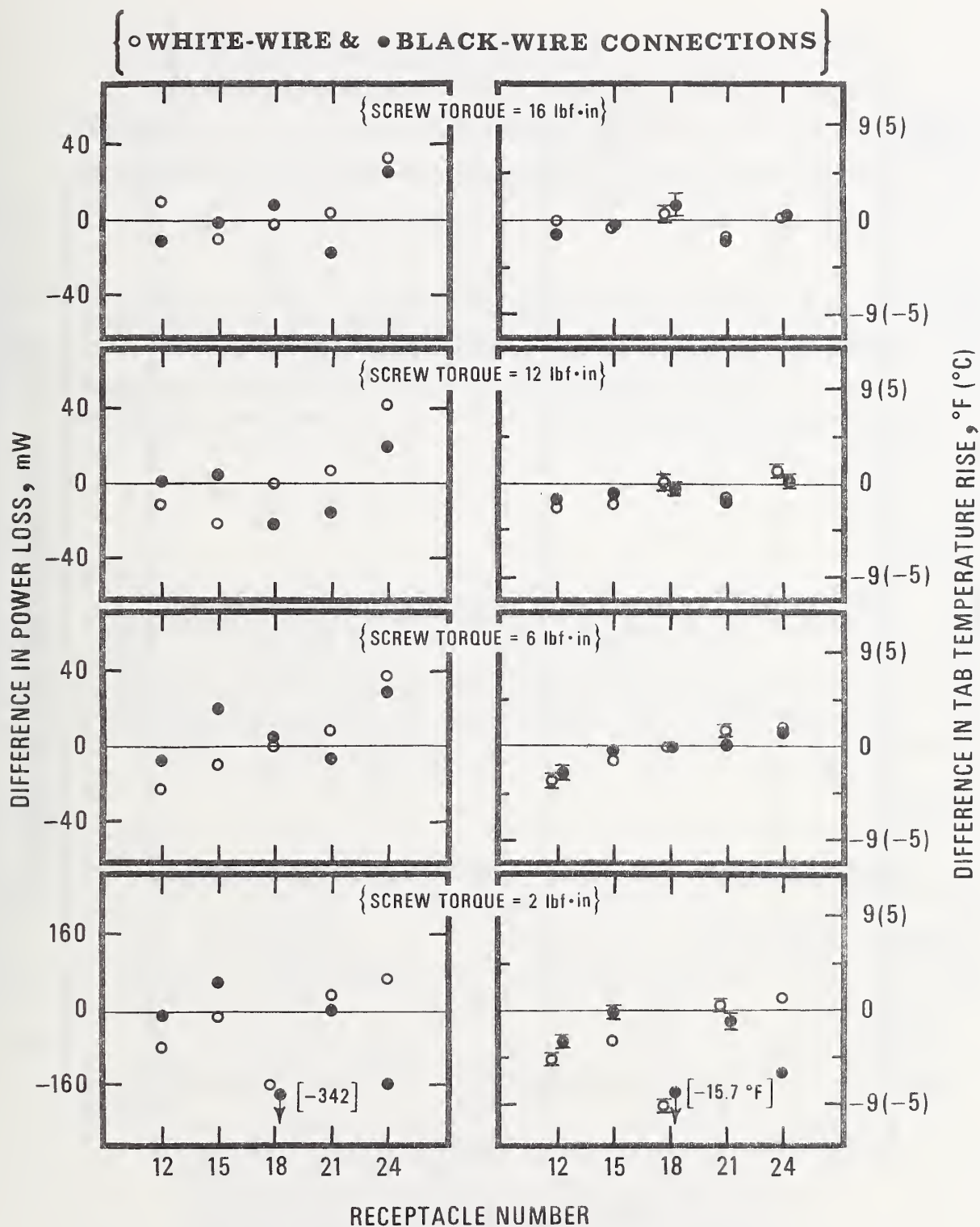
Figure 38. Difference between the values of power loss and tab temperature rise obtained in individual receptacle tests and those obtained in group receptacle tests conducted with the receptacles spaced two outlet boxes apart. Difference equals average of values obtained in individual receptacle tests using a test voltage of 10 V(ac) minus average of values obtained in group receptacle tests using a test voltage of 10 V(ac). Bars give the 95% confidence limits for the difference between the averages.
