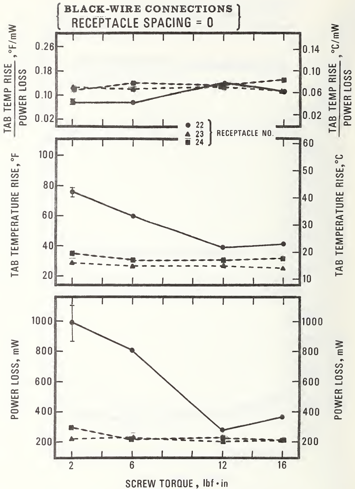
Figure 25. Values of the power loss, the tab temperature rise, and the ratio of the tab temperature rise to the power loss plotted as a function of the terminal screw torque for the black-wire connections of conventional receptacles No. 22, 23, and 24. The receptacles were installed in adjacent outlet boxes. The values plotted are averages of values determined in tests employing test voltages of 10 V(dc), 10 V(ac), and 115 V(ac). The bars give the range of the values.
