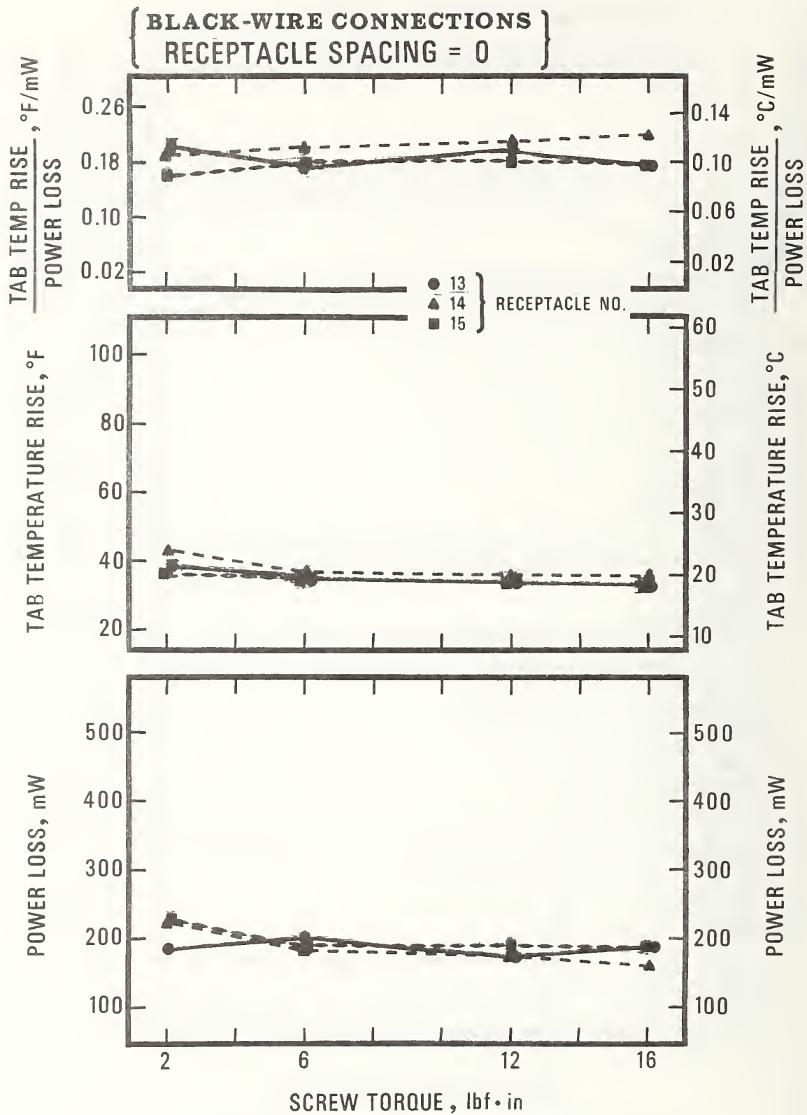
Figure 19. Values of the power loss, the tab temperature rise, and the ratio of the tab temperature rise to the power loss plotted as a function of the terminal screw torque for the black-wire connections of conventional receptacles No. 13, 14, and 15. The receptacles were installed in adjacent outlet boxes. The values plotted are averages of values determined in tests employing test voltages of 10 V(dc), 10 V(ac), and 115 V(ac). The bars give the range of the values.
