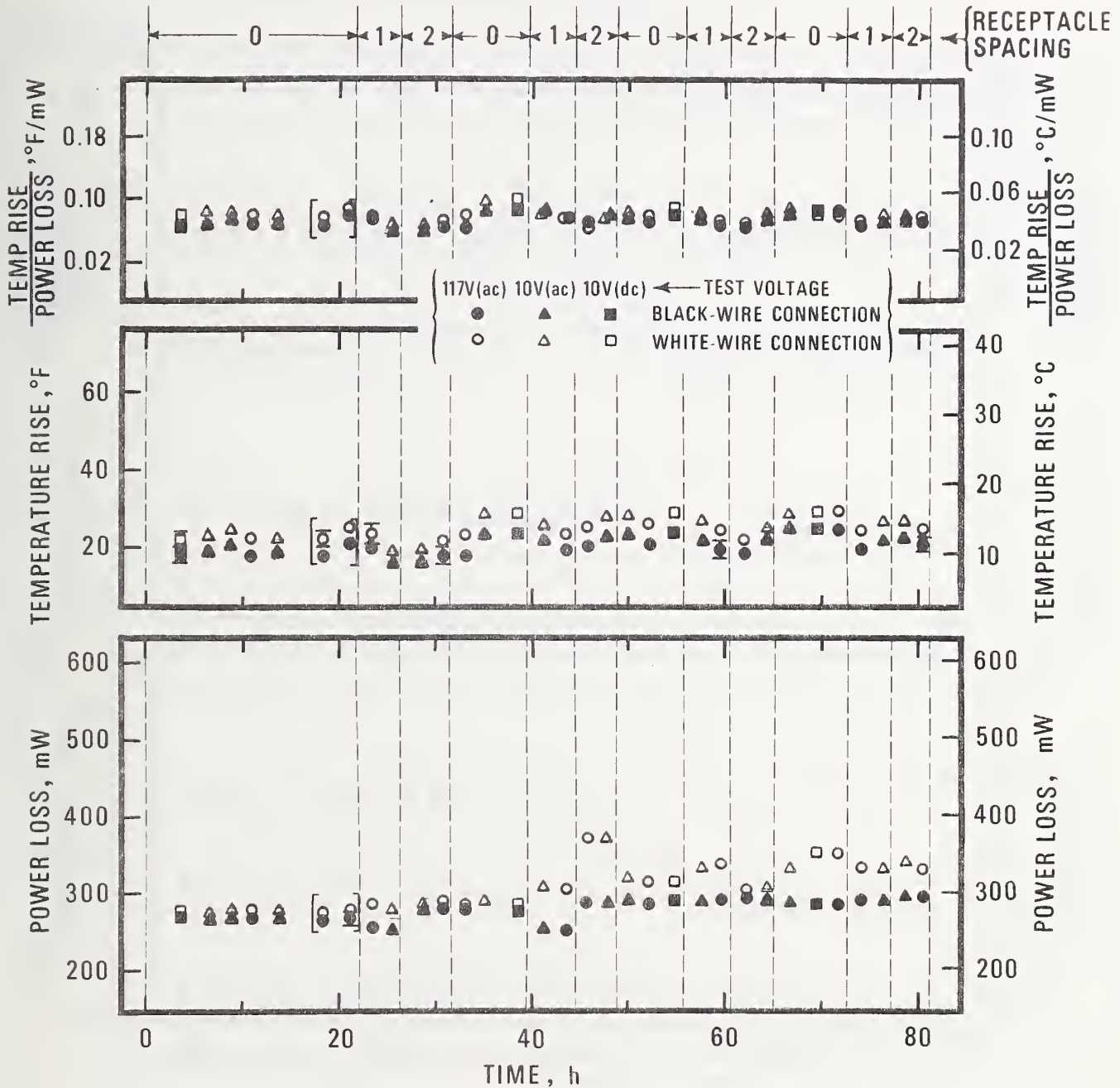
Figure 40. Values of the power loss, the temperature rise, and the ratio of the temperature rise to the power loss for the black-wire and white-wire connections of split-beam receptacle No. 7 plotted as a function of the time that test circuit was energized. Each of the data points represents the average of values obtained in several (2 to 4) tests. The bars give the 95% confidence limits for the averages. The symbol heights are equivalent to about 15 mW, 3 °F, and 0.015 °F/mW for the power loss, the temperature rise, and the ratio, respectively.
