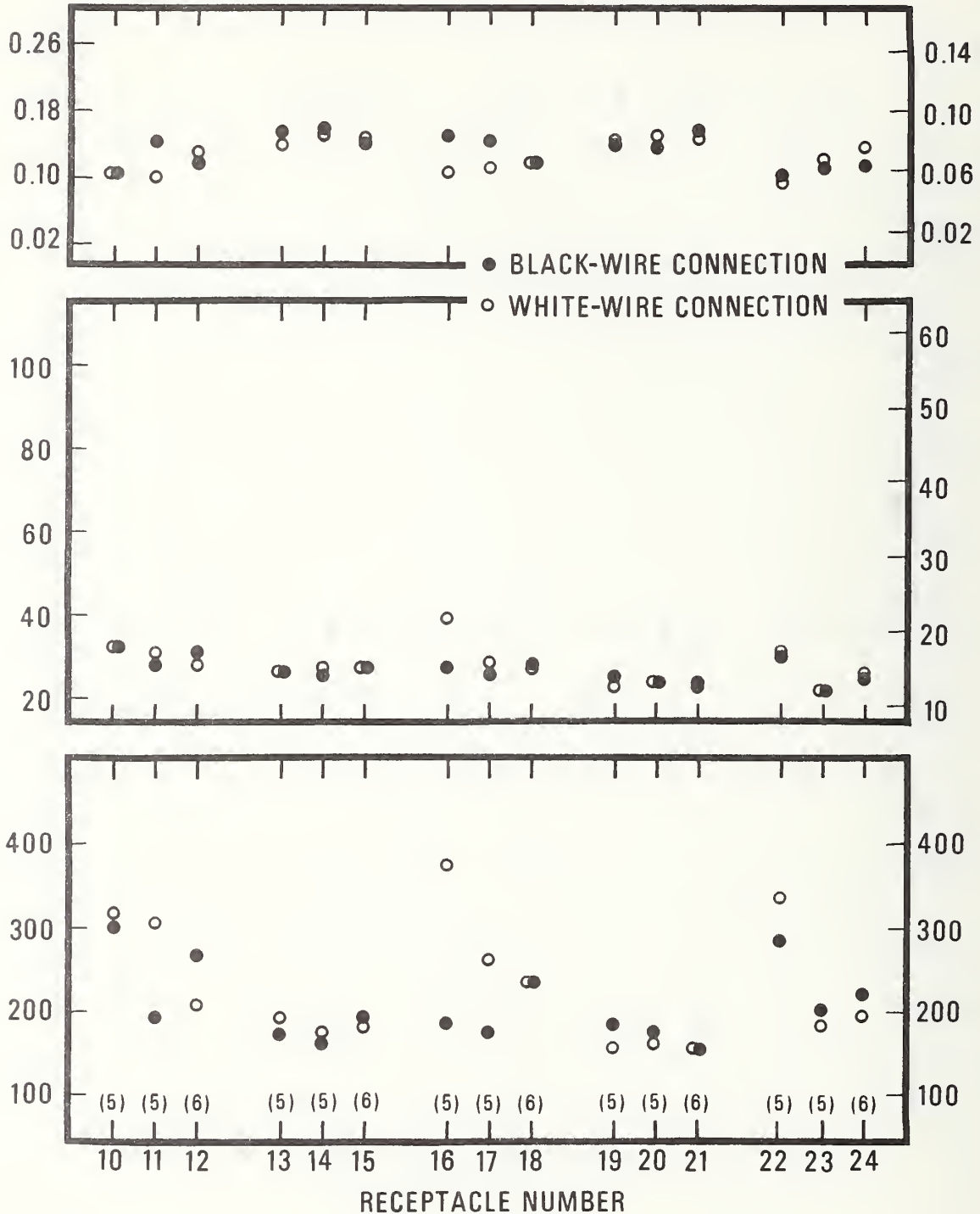
Figure 9. Values of the power loss, the tab temperature rise, and the ratio of the tab temperature rise to the power loss obtained for the black-wire and white-wire connections of the conventional receptacles during group receptacle tests: receptacles spaced one outlet box apart, terminal screws tightened with a torque of 12 lbf·in. The values plotted are averages of values determined in tests employing test voltages of 10 V(ac) and 115 V(ac). The figures in parentheses indicate the number of tests used in computing the averages. The range of the values was less than the symbol heights, which are equivalent to about 15 mW, 3 °F, and 0.015 °F/mW for the power loss, the temperature rise, and the ratio, respectively.
