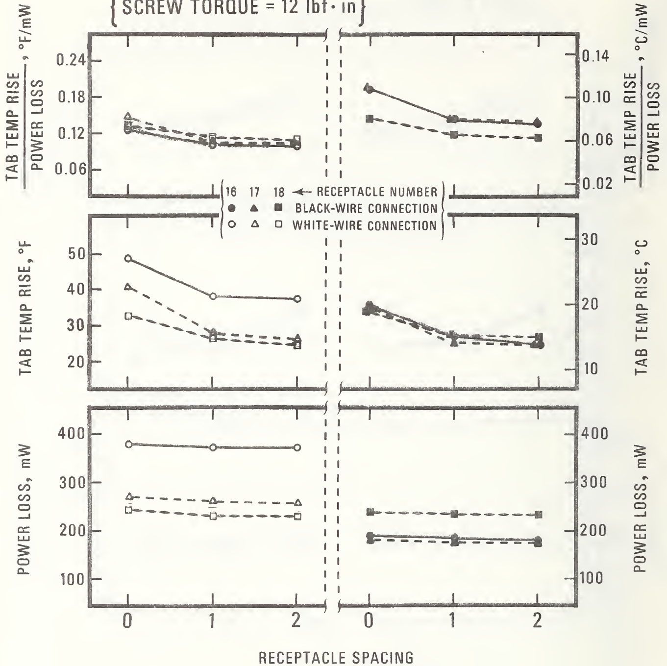
Figure 29. Values of the power loss, the tab temperature rise, and the ratio of the tab temperature rise to the power loss plotted as a function of the receptacle spacing for the black-wire and white-wire connections of conventional receptacles No. 16, 17, and 18. The terminal screws of the receptacles were tightened with a torque of 12 lbf·in. The values plotted are averages of values determined in tests employing a test voltage of 10 V(ac). The range of the values was less than the symbol heights, which are equivalent to about 15 mW, 2 °F, and 0.012 °F/mW for the power loss, the temperature rise, and the ratio, respectively.
