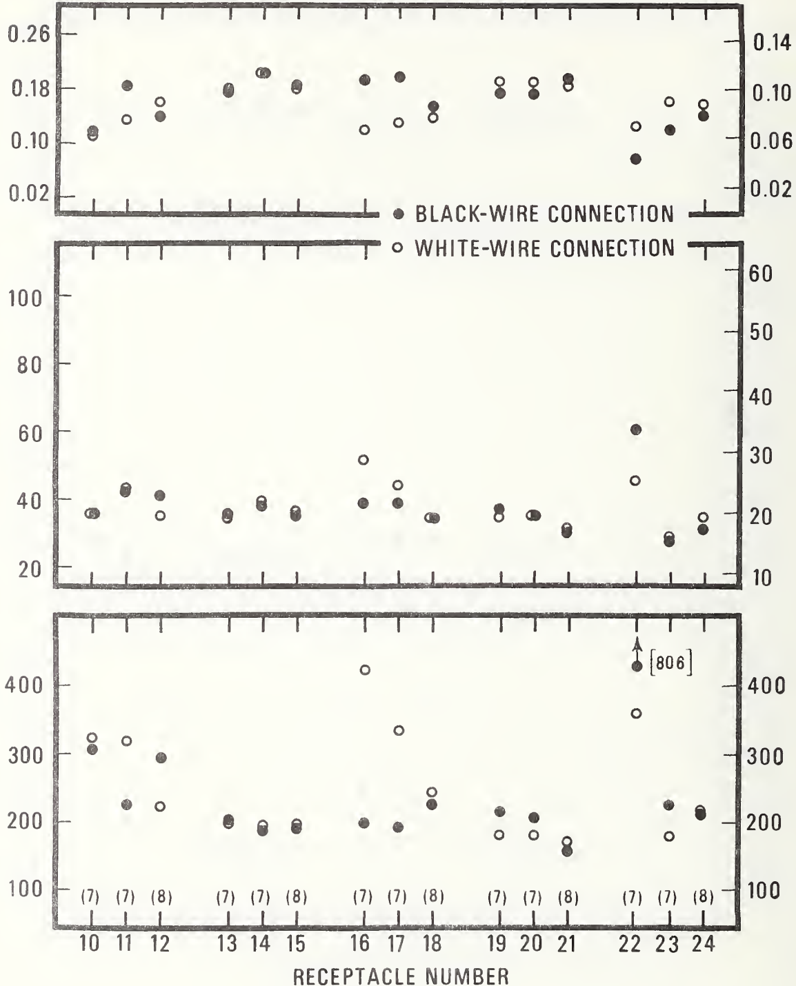
Figure 11. Values of the power loss, the tab temperature rise, and the ratio of the tab temperature rise to the power loss obtained for the black-wire and white-wire connections of the conventional receptacles during group receptacle tests: receptacles installed in adjacent outlet boxes, terminal screws tightened with a torque of 6 lbf·in. The values plotted are averages of values determined in tests employing test voltages of 10 V(dc), 10 V(ac), and 115 V(ac). The figures in parentheses indicate the number of tests used in computing the averages. The range of the values was less than the symbol heights, which are equivalent to about 15 mW, 3°F, and 0.015 °F/mW for the power loss, the temperature rise, and the ratio, respectively.
