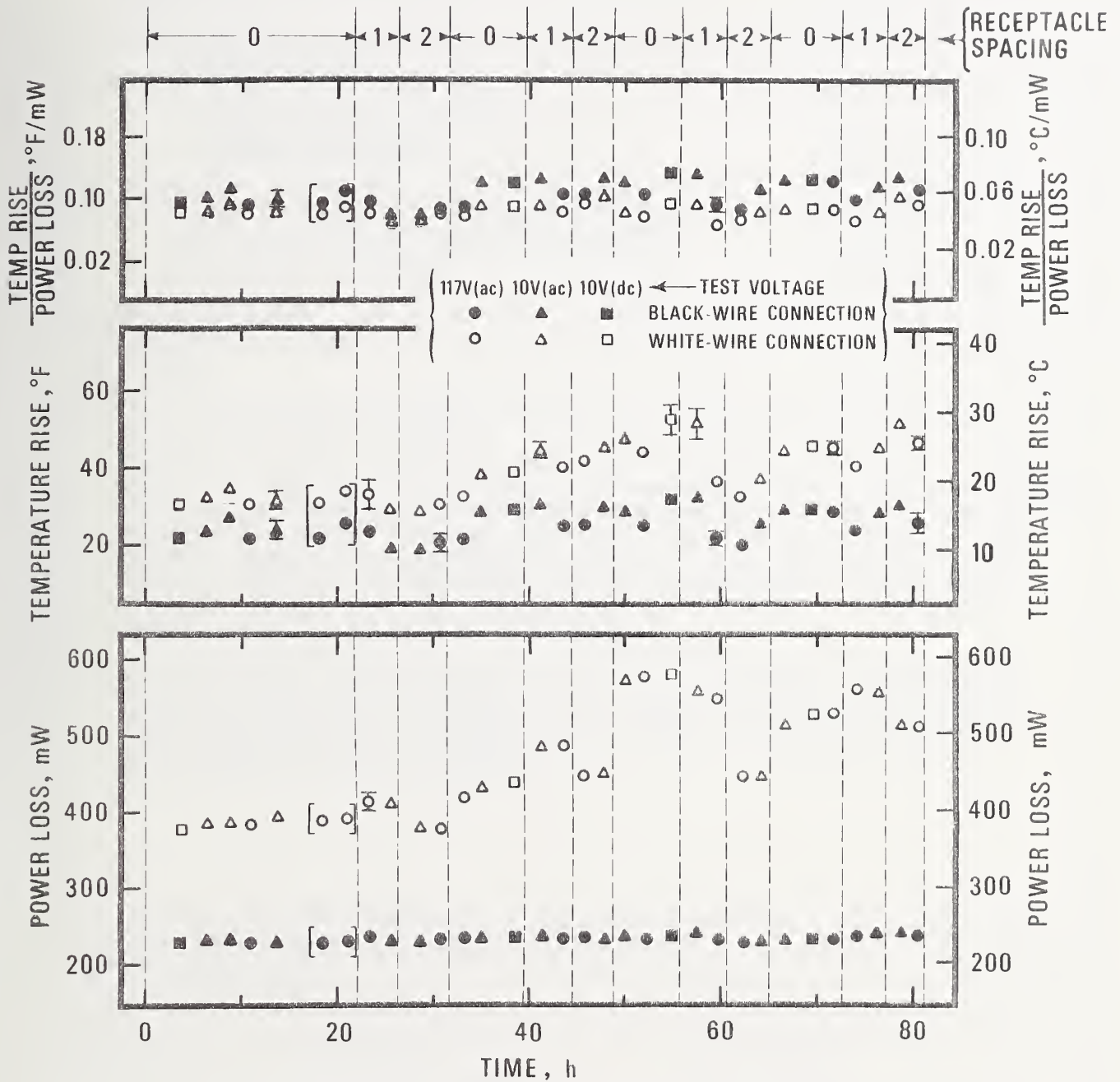
Figure 42. Values of the power loss, the temperature rise, and the ratio of the temperature rise to the power loss for the black-wire and white-wire connections of split-beam receptacle No. 9 plotted as a function of the time that test circuit was energized. Each of the data points represents the average of values obtained in several (2 to 4) tests. The bars give the 95% confidence limits for the averages. The symbol heights are equivalent to about 15 mW, 3°F, and 0.015 °F/mW for the power loss, the temperature rise, and the ratio, respectively.
