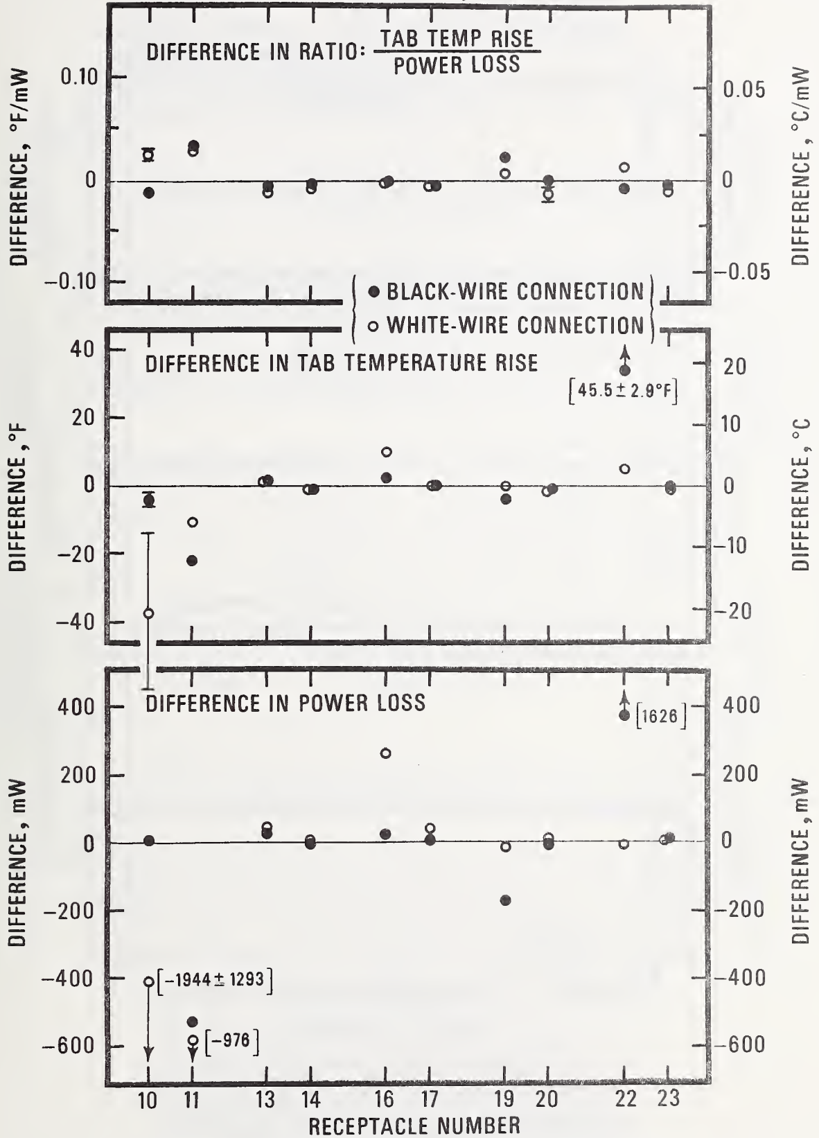
Figure 34. Change in the power loss, the tab temperature rise, and the ratio of the tab temperature rise to the power loss for the black-wire and white-wire connections of the conventional receptacles in Group 1 due to retightening the terminal screws with a torque of 2 lbf · in. Difference equals average of values obtained in tests 79, 80, and 81 minus average of values obtained in tests 69 and 70. The receptacles were spaced two outlet boxes apart, and the test voltage was 10 V(ac) for each of the tests. The bars give the 95% confidence limits for the difference between the averages.
