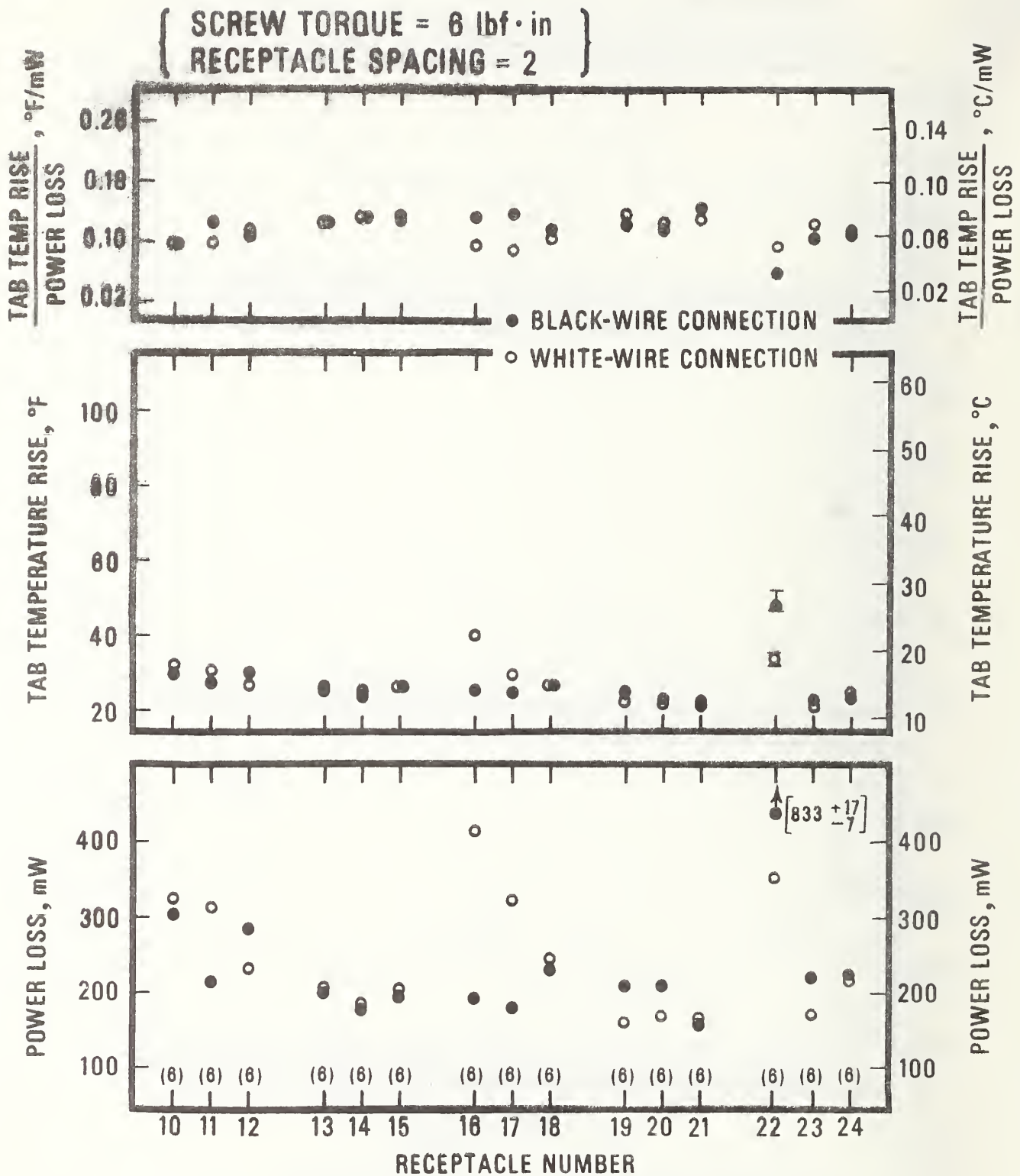
Figure 13. Values of the power loss, the tab temperature rise, and the ratio of the tab temperature rise to the power loss obtained for the black-wire and white-wire connections of the conventional receptacles during group receptacle tests: receptacles spaced two outlet boxes apart, terminal screws tightened with a torque of 6 lbf·in. The values plotted are averages of values determined in tests employing test voltages of 10 V(ac) and 115 V(ac). The figures in parentheses indicate the number of tests used in computing the averages. The bars give the range of the values. The symbol heights are equivalent to about 15 mW, 3 °F, and 0.015 °F/mW for the power loss, the temperature rise, and the ratio, respectively.
