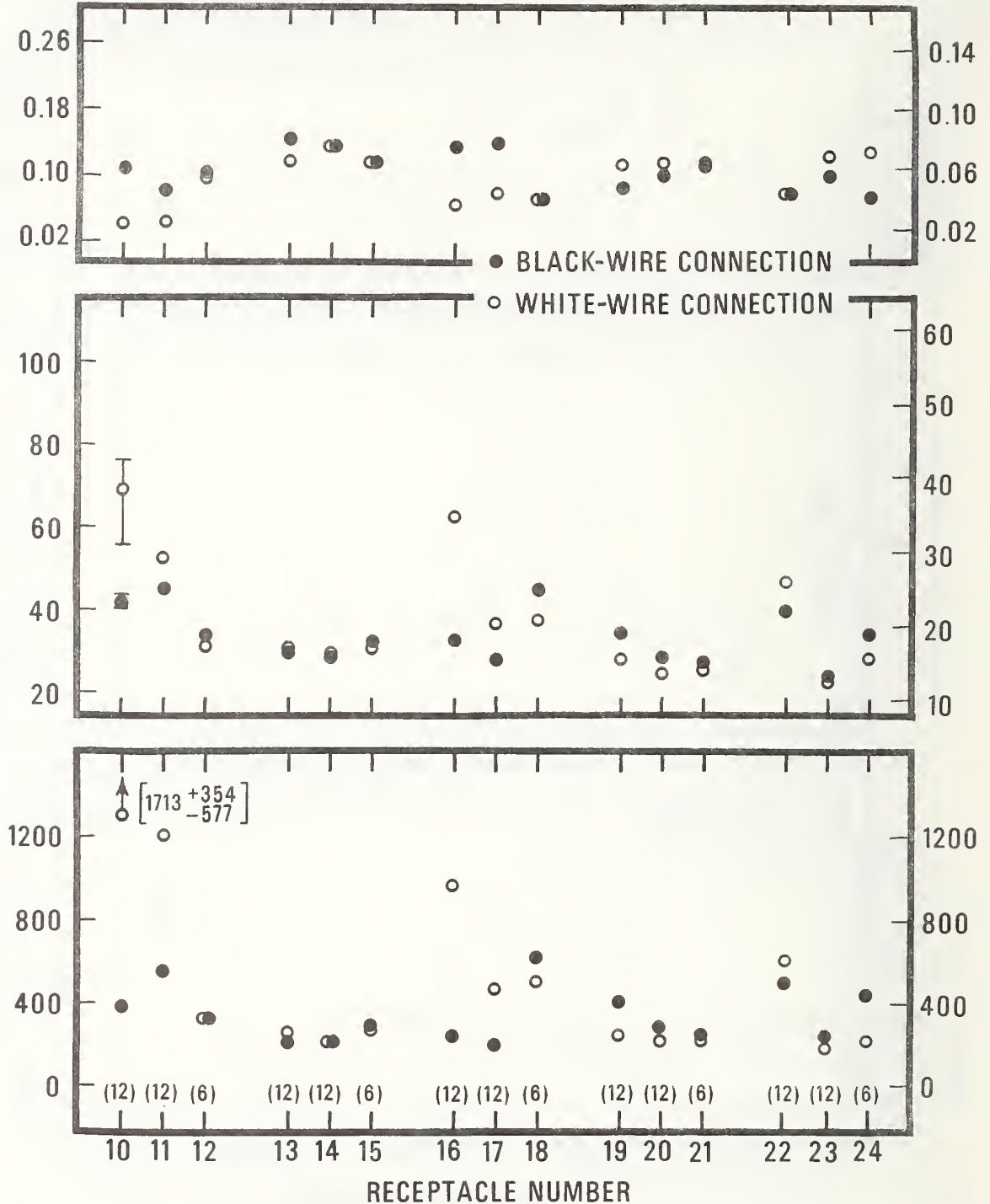
Figure 15. Values of the power loss, the tab temperature rise, and the ratio of the tab temperature rise to the power loss obtained for the black-wire and white-wire connections of the conventional receptacles during group receptacle tests: receptacles spaced one outlet box apart, terminal screws tightened with a torque of 2 lbf·in. The values plotted are averages of values determined in tests employing test voltages of 10 V(ac) and 115 V(ac). The figures in parentheses indicate the number of tests used in computing the averages. The bars give the range of the values. The symbol heights are equivalent to about 60 mW, 3 °F, and 0.015 °F/mW for the power loss, the temperature rise, and the ratio, respectively.
