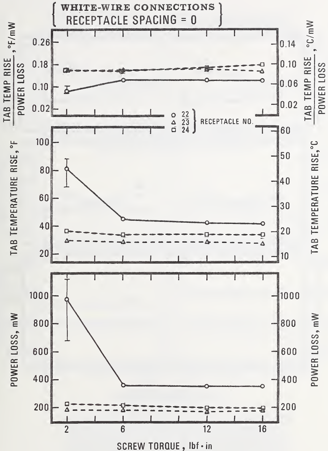
Figure 26. Values of the power loss, the tab temperature rise, and the ratio of the tab temperature rise to the power loss plotted as a function of the terminal screw torque for the white-wire connections of conventional receptacles No. 22, 23, and 24. The receptacles were installed in adjacent outlet boxes. The values plotted are averages of values determined in tests employing test voltages of 10 V(dc), 10 V(ac), and 115 V(ac). The bars give the range of the values.
