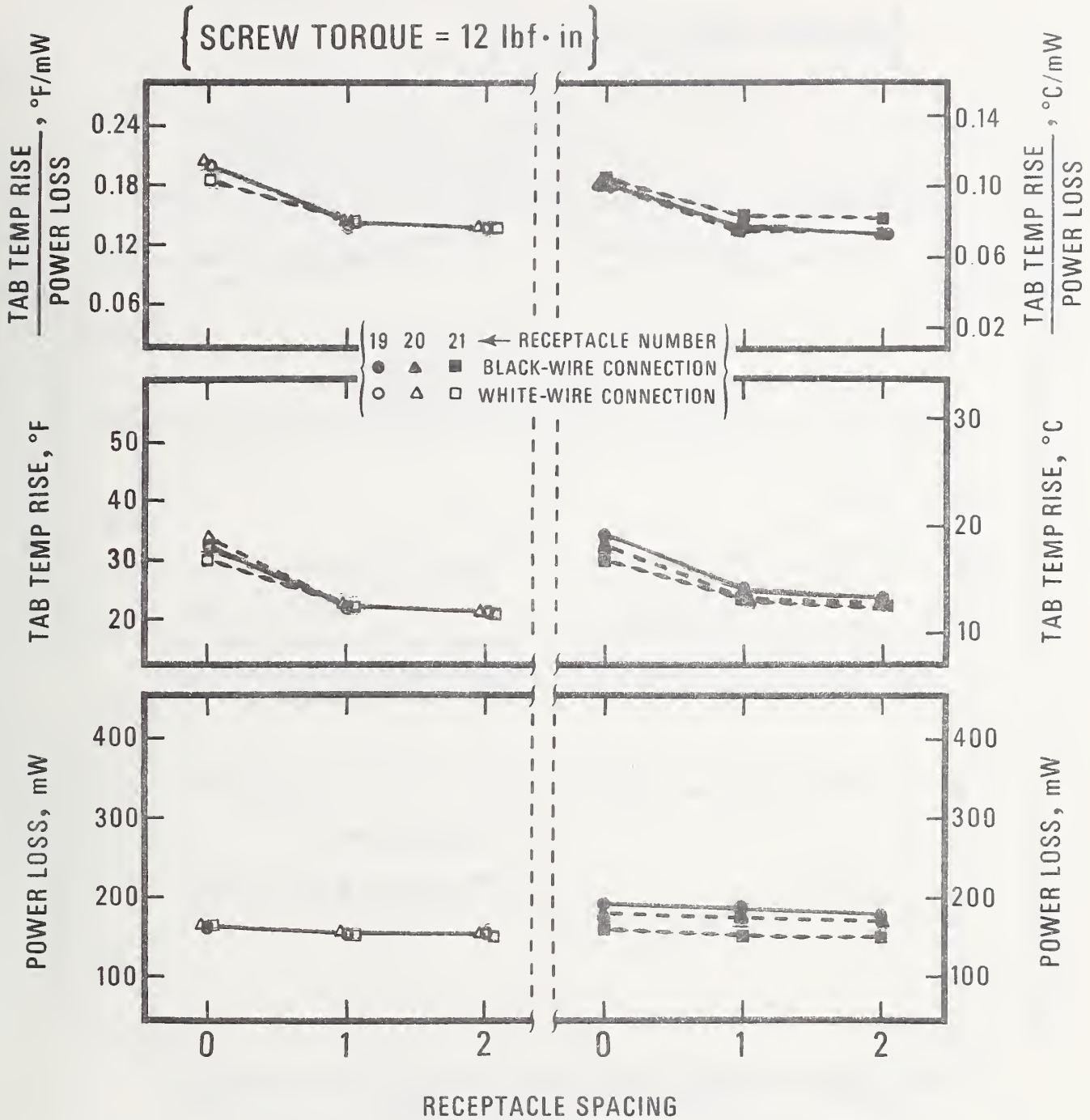
Figure 30. Values of the power loss, the tab temperature rise, and the ratio of the tab temperature rise to the power loss plotted as a function of the receptacle spacing for the black-wire and white-wire connections of conventional receptacles No. 19, 20, and 21. The terminal screws of the receptacles were tightened with a torque of 12 lbf·in. The values plotted are averages of values determined in tests employing a test voltage of 10 V(ac). The range of the values was less than the symbol heights, which are equivalent to about 15 mW, 2 °F, and 0.012 ° F/mW for the power loss, the temperature rise, and the ratio, respectively.
