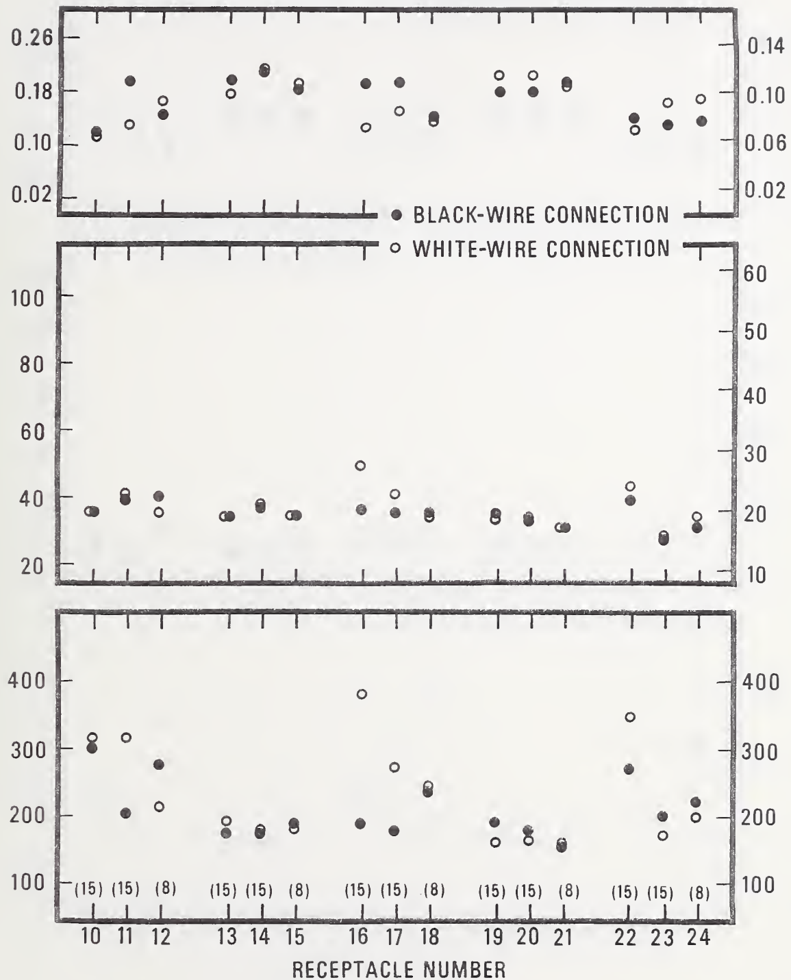
Figure 8. Values of the power loss, the tab temperature rise, and the ratio of the tab temperature rise to the power loss obtained for the black-wire and white-wire connections of the conventional receptacles during group receptacle tests: receptacles installed in adjacent outlet boxes, terminal screws tightened with a torque of 12 lbf·in. The values plotted are averages of values determined in tests employing test voltages of 10 V(dc), 10 V(ac), and 115 V(ac). The figures in parentheses indicate the number of tests used in computing the averages. The range of the values was less than the symbol heights, which are equivalent to about 15 mW, 3 °F, and 0.015 °F/mW for the power loss, the temperature rise, and the ratio, respectively.
