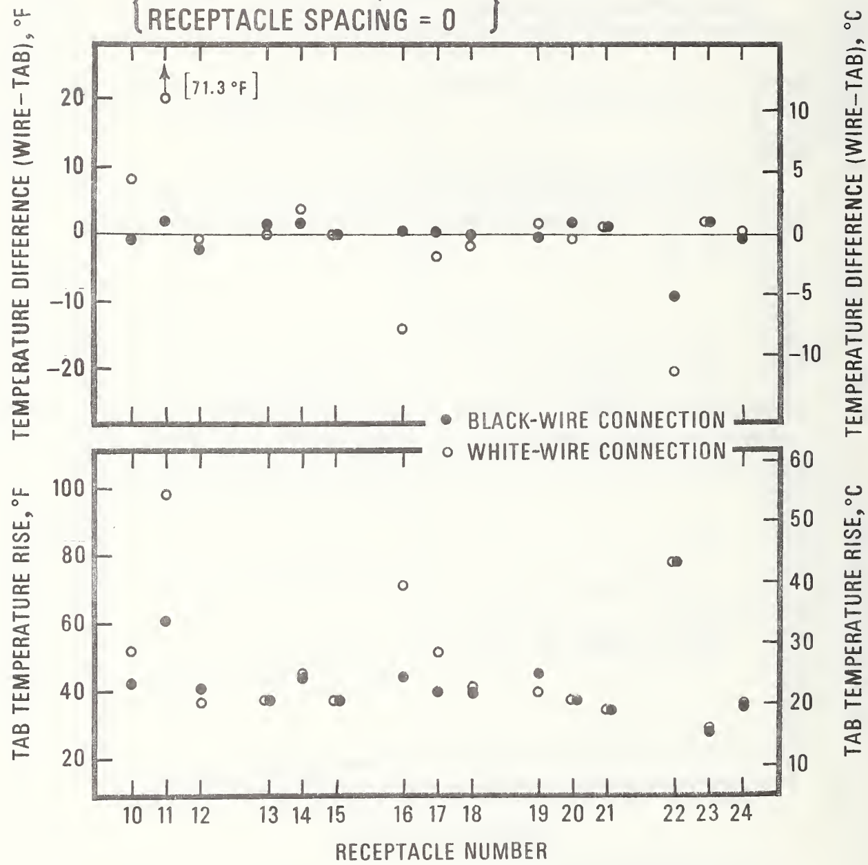
Figure 33. The tab temperature rise and the difference between the wire temperature and the tab temperature for the black-wire and white-wire connections of the conventional receptacles: receptacles installed in adjacent outlet boxes, terminal screws tightened with a torque of 2 lbf in. The difference was calculated from the averages of values determined during three consecutive tests in which the test voltage was 10 V(ac). The 99% confidence limits for the difference between the averages are less than the symbol heights, which are equivalent to about 1.5 °F for the difference and about 3 °F for the tab temperature rise.
