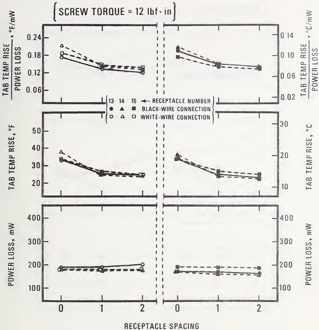
Figure 28. Values of the power loss, the tab temperature rise, and the ratio of the tab temperature rise to the power loss plotted as a function of the receptacle spacing for the black-wire and white-wire connections of conventional receptacles No. 13, 14, and 15. The terminal screws of the receptacles were tightened with a torque of 12 lbf·in. The values plotted are averages of values determined in tests employing a test voltage of 10 V(ac). The range of the values was less than the symbol heights, which are equivalent to about 15 mW, 2 °F, and 0.012 °F/mW for the power loss, the temperature rise, and the ratio, respectively.
