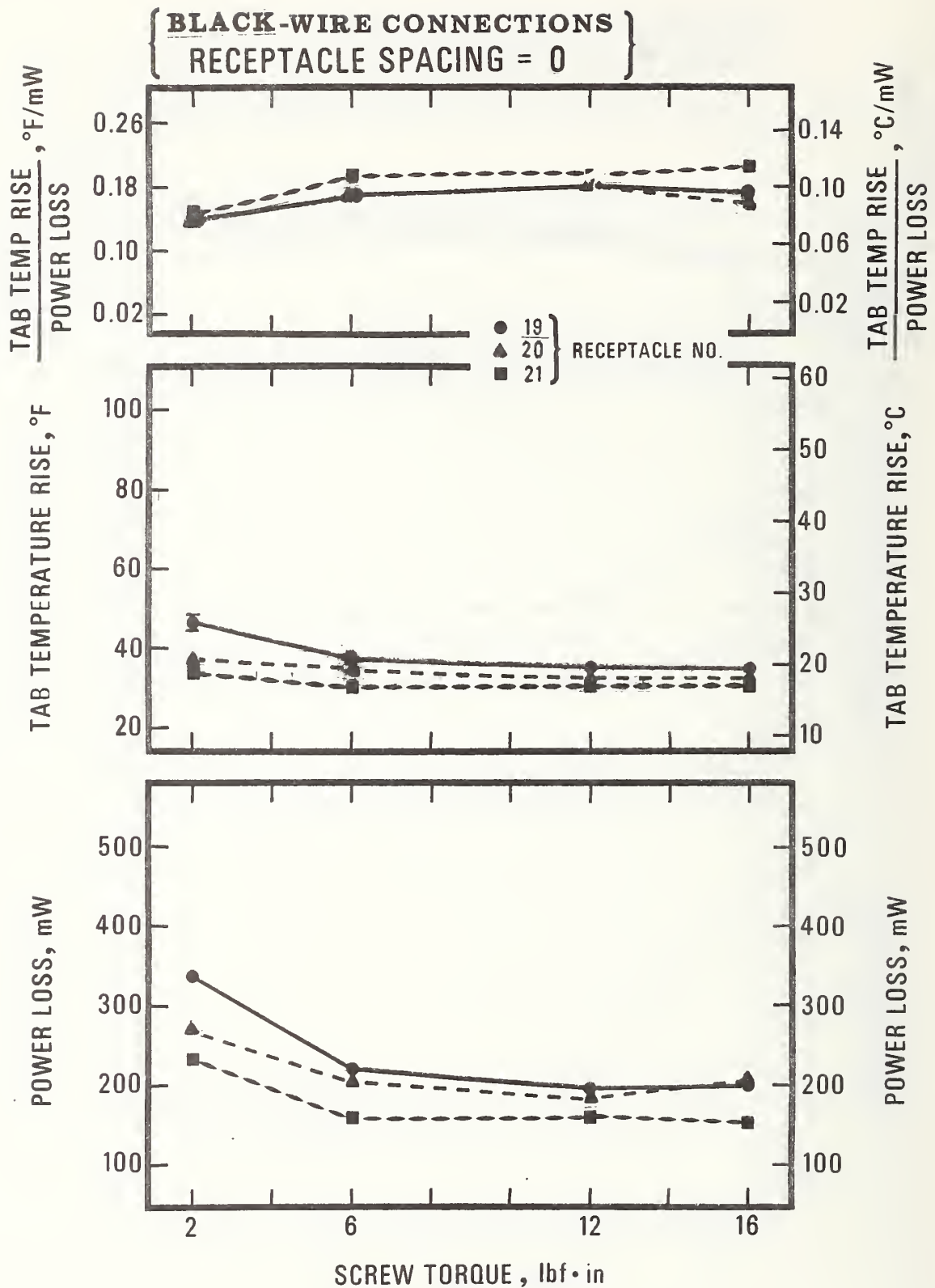
Figure 23. Values of the power loss, the tab temperature rise, and the ratio of the tab temperature rise to the power loss plotted as a function of the terminal screw torque for the black-wire connections of conventional receptacles No. 19, 20, and 21. The receptacles were installed in adjacent outlet boxes. The values plotted are averages of values determined in tests employing test voltages of 10 V(dc), 10 V(ac), and 115 V(ac). The bars give the range of the values.
