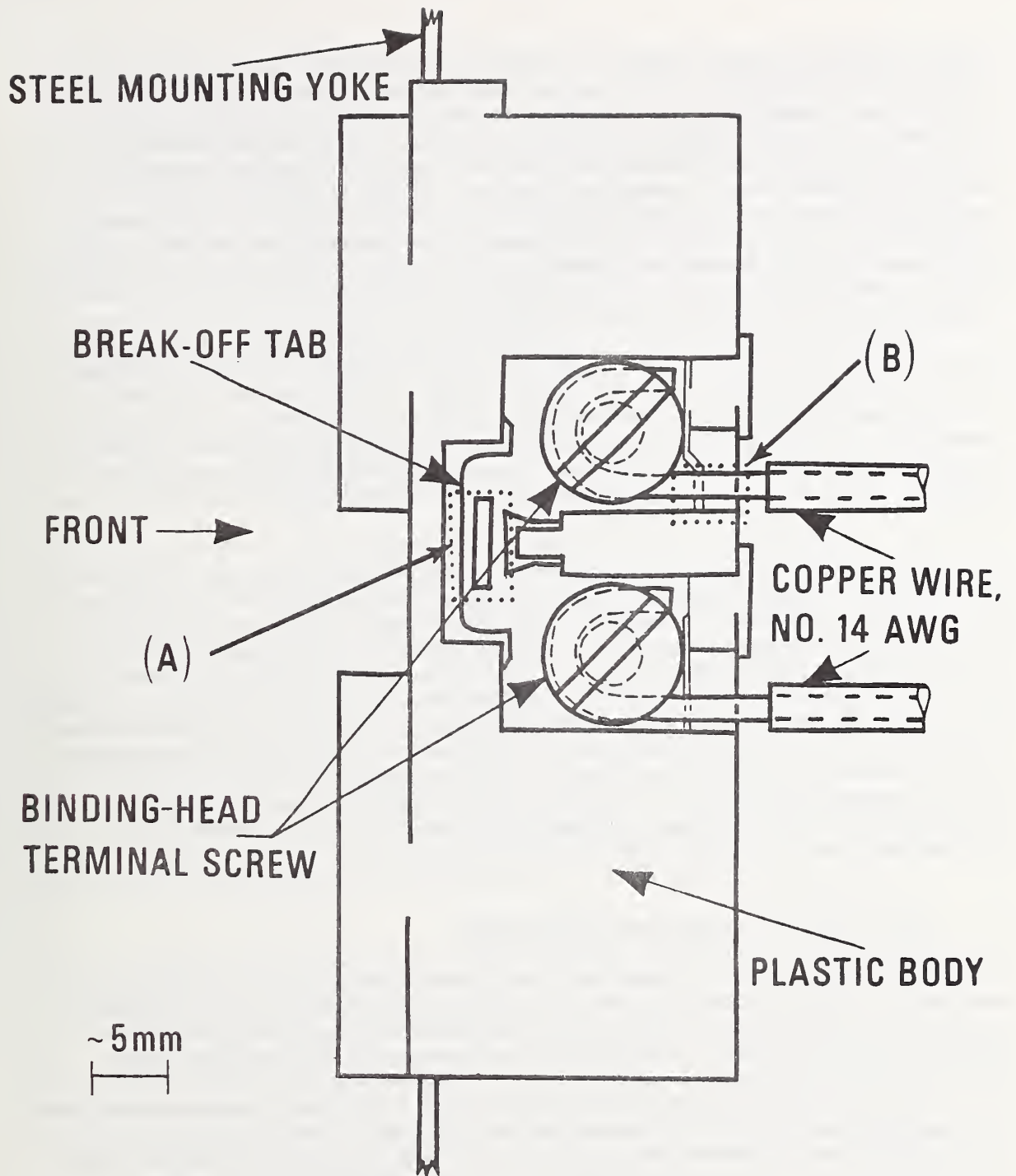
Figure 2. Side view of a conventional receptacle showing electrical connections to black-wire terminal and showing locations where thermocouple measuring junctions were attached for measuring (A) the tab temperature and (B) the wire temperature.
