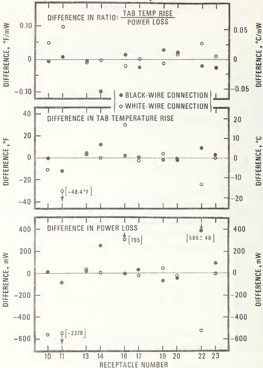
Figure 35. Change in the power loss, the tab temperature rise, and the ratio or the tab temperature rise to the power loss for the black-wire and white-wire connections of the conventional receptacles in Group 1 due to retightening the terminal screws with a torque of 2 lbf · in. Difference equals average of values obtained in tests 202, 203, 204, 205, and 206 minus average of values obtained in tests 17, 18, and 19. The receptacles were installed in adjacent outlet boxes, and the test voltage was 10 V(ac) for each of the tests. The bars give the 95% confidence limits for the differences between the averages.
