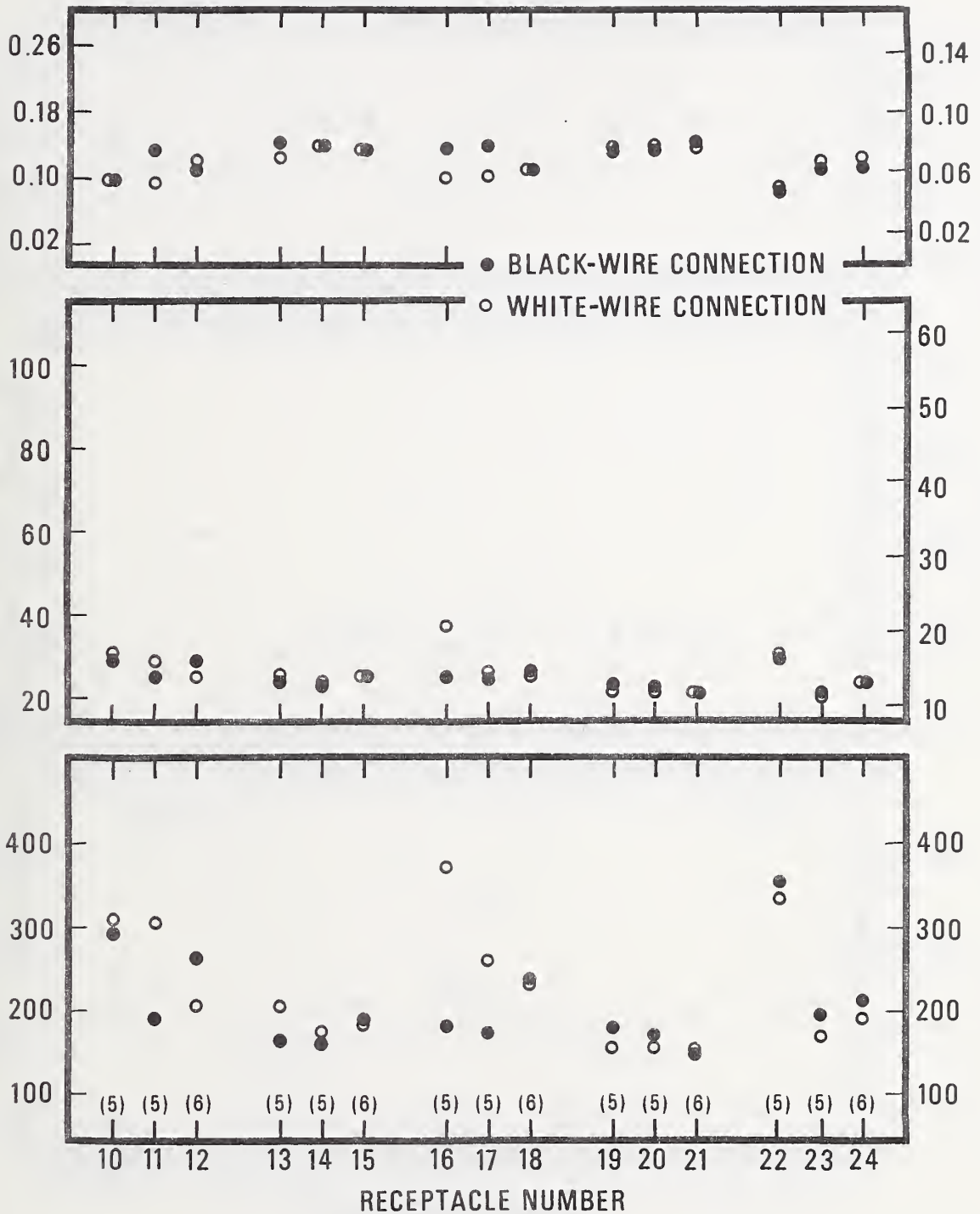
Figure 10. Values of the power loss, the tab temperature rise, and the ratio of the tab temperature rise to the power loss obtained for the black-wire and white-wire connections of the conventional receptacles during group receptacle tests: receptacles spaced two outlet boxes apart, terminal screws tightened with a torque of 12 lbf·in. The values plotted are averages of values determined in tests employing test voltages of 10 V(ac) and 115 V(ac). The figures in parentheses indicate the number of tests used in computing the averages. The range of the values was less than the symbol heights, which are equivalent to about 15 mW, 3 °F, and 0.015 °F/mW for the power loss, the temperature rise, and the ratio, respectively.
