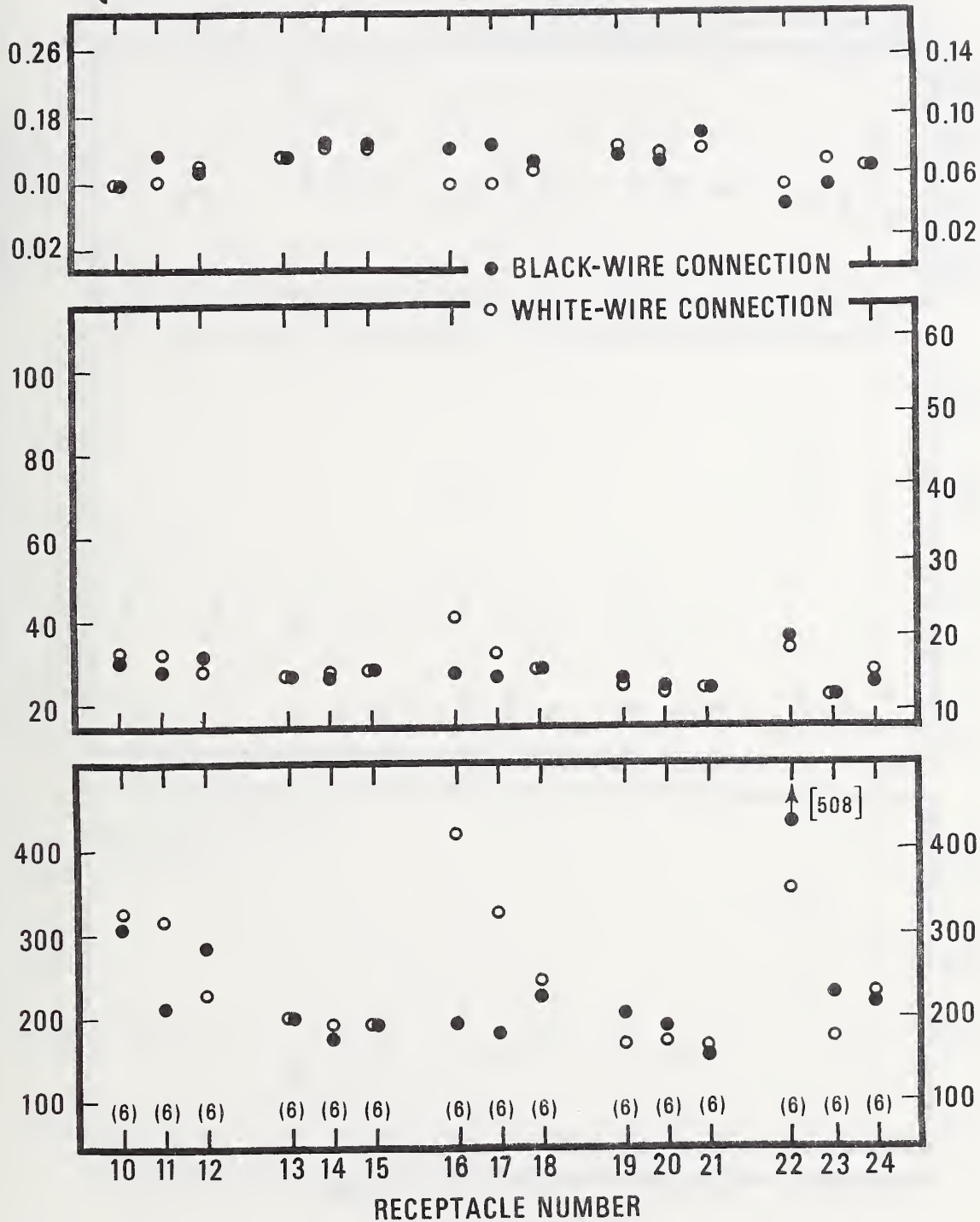
Figure 12. Values of the power loss, the tab temperature rise, and the ratio of the tab temperature rise to the power loss obtained for the black-wire and white-wire connections of the conventional receptacles during group receptacle tests: receptacles spaced one outlet box apart, terminal screws tightened with a torque of 6 lbf·in. The values plotted are averages of values determined in tests employing test voltages of 10 V(ac) and 115 V(ac). The figures in parentheses indicate the number of tests used in computing the averages. The range of the values was less than the symbol heights, which are equivalent to about 15 mW, 3 °F, and 0.015 °F/mW for the power loss, the temperature rise, and the ratio, respectively.
