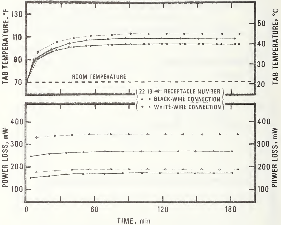
Figure 37. Power loss and tab temperature as a function of time for the black-wire and white-wire connections of the indicated conventional receptacles. The test circuit was energized at time equals 0 by applying a test voltage of 10 V(ac); the test current was maintained at 15 A. The values plotted were obtained in tests 161 through 172: receptacles installed in adjacent outlet boxes, terminal screws tightened with a torque of 12 lbf·in.
