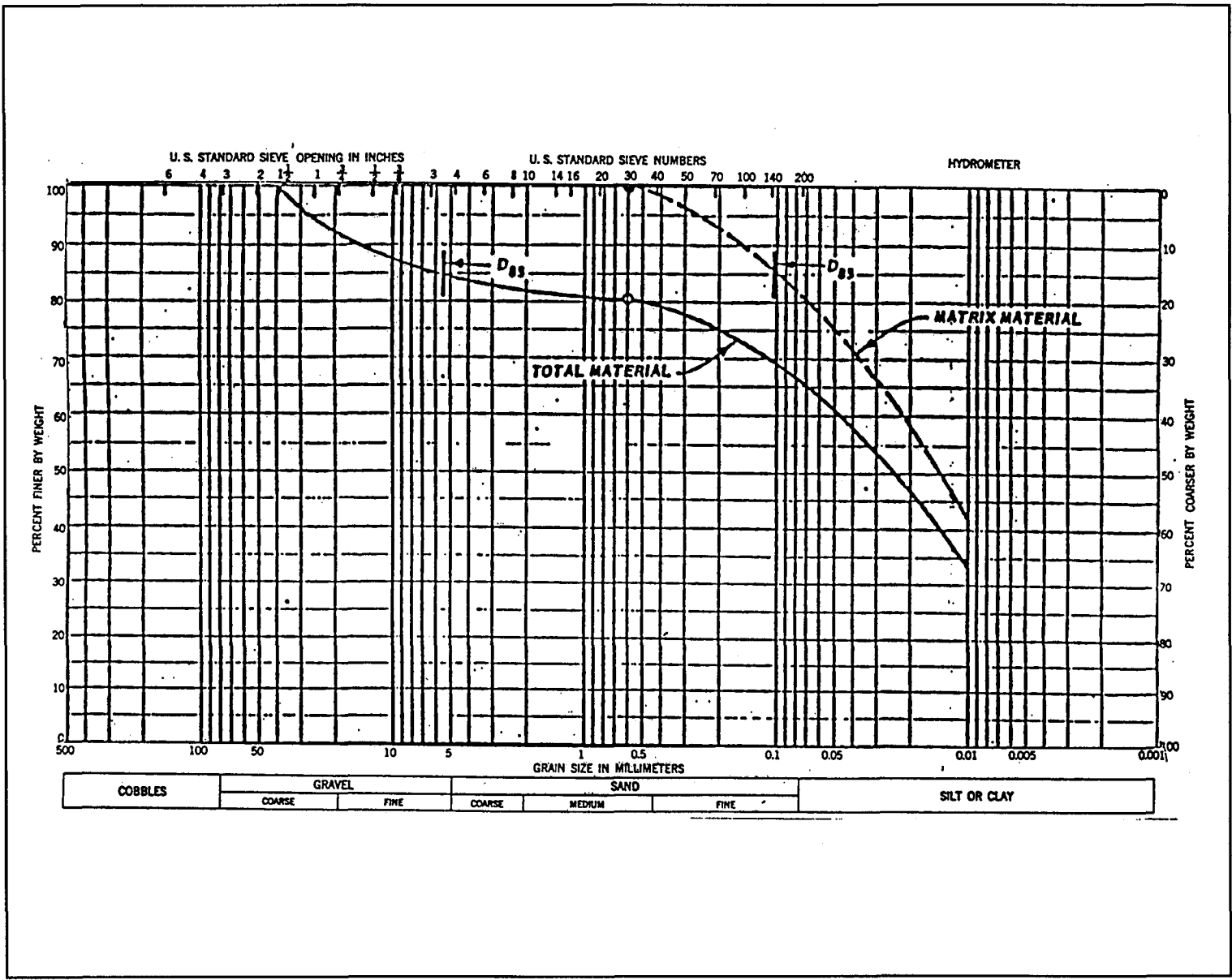
Figure D-1. Analysis of a gap-graded material
