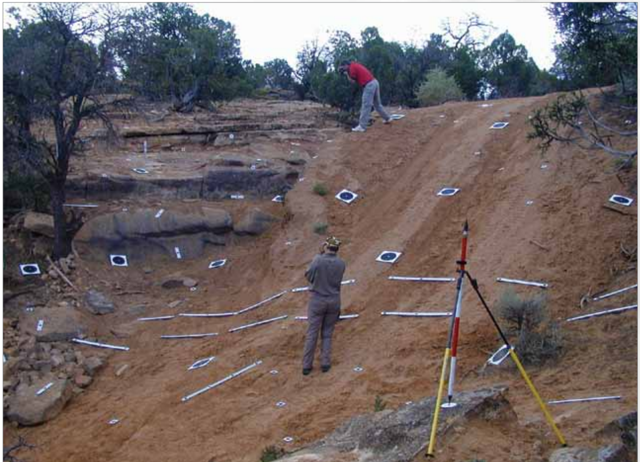
BLM geographer Neffra Matthews (bottom) and BLM physical scientist Tom Noble take a series of photos so they can use close-range photogrammetry methods to create three dimensional surface information to help quantify effects from rapidly increasing off-highway vehicle (OHV) use in the Dry Creek Extreme OHV Area.
