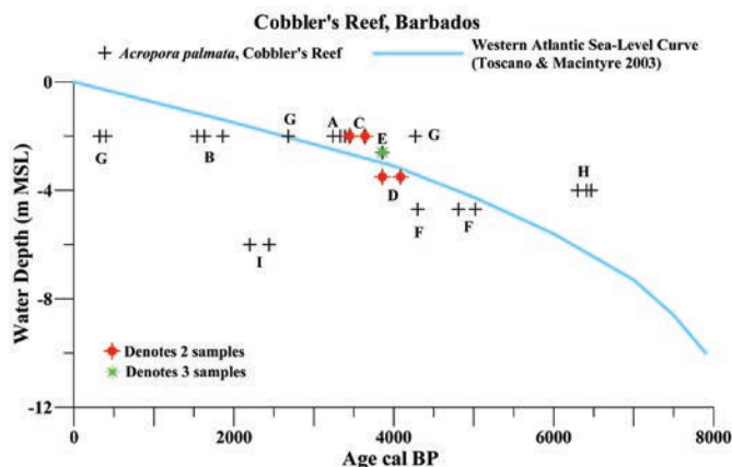
FIGURE 9. Radiocarbon dates of Acropora palmata from the crest of Cobbler's Reef plotted in relation to the Western Atlantic sea-level curve (Toscano and Macintyre, 2003). Note the samples that plot above the sea-level curve, which indicate storm damage. There has been no additional reef accumulation for the past 3,000 years (Macintyre et al., 2007). Letters refer to the sites in Figure 7.
