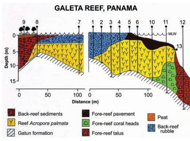
FIGURE 2. Transect across Galeta Reef showing the six reef facies and peat accumulation.
