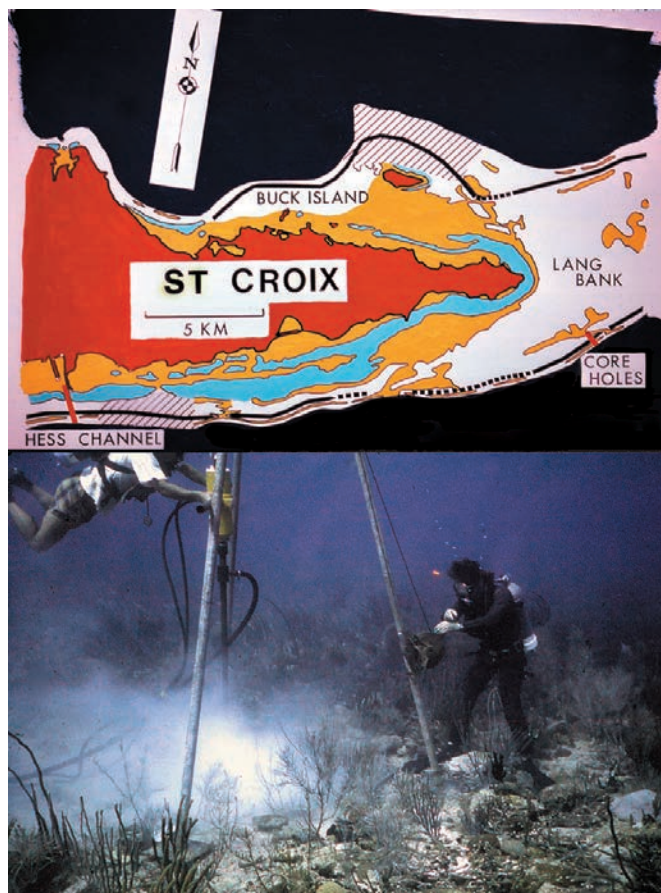
FIGURE 4. Map of the east end of St. Croix showing location of core-hole drilling on a bottom of scattered coral heads and octo-corals (modified from Adey et al., 1977; photo courtesy of Ian G. Macintyre).
