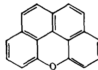
1,8,9-Perinaphthoxanthene
